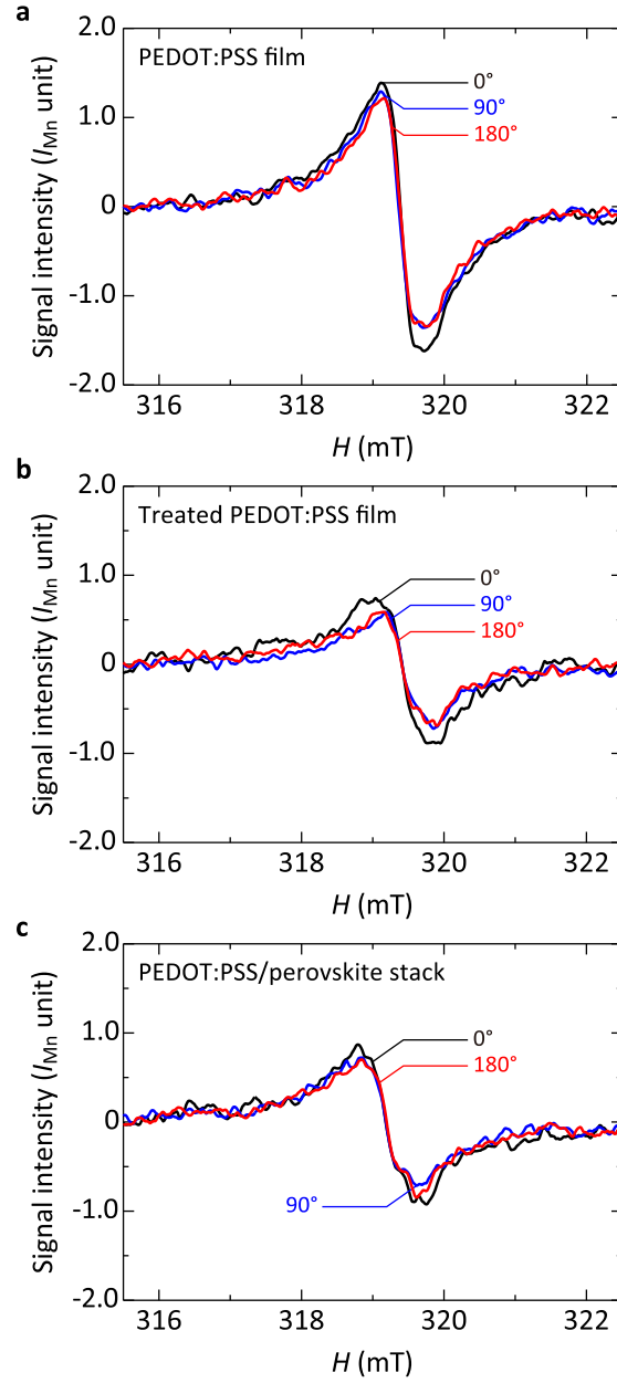
Supplementary Figure 1 | Anisotropy of g -factors of PEDOT:PSS films. Angular dependence of ESR spectra of a , as-fabricated PEDOT:PSS film, b , treated PEDOT:PSS film, and c , PEDOT:PSS/perovskite stack. The angles indicated here are angles between the external magnetic field to the substrate plane.
