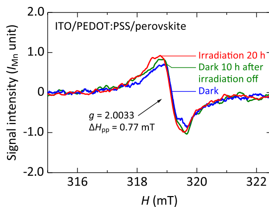
Supplementary Figure 2 | ESR spectra of an ITO/PEDOT:PSS/perovskite stack under simulated solar irradiation.
