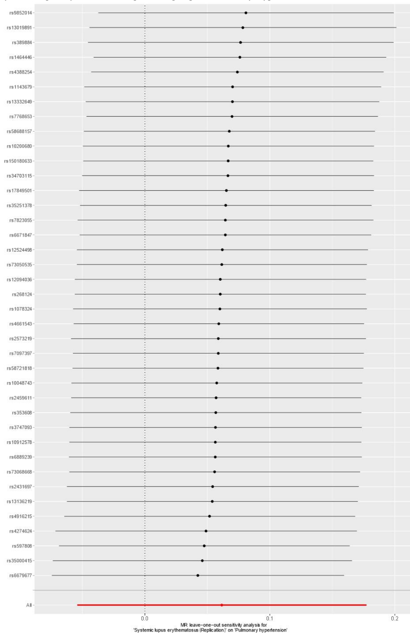
Supplementary Figure S2. Leave-one-out analysis, MR effect size, funnel plot and MR-Egger scatter plot for Systemic lupus erythematosus Replication group on Pulmonary Hypertension.
