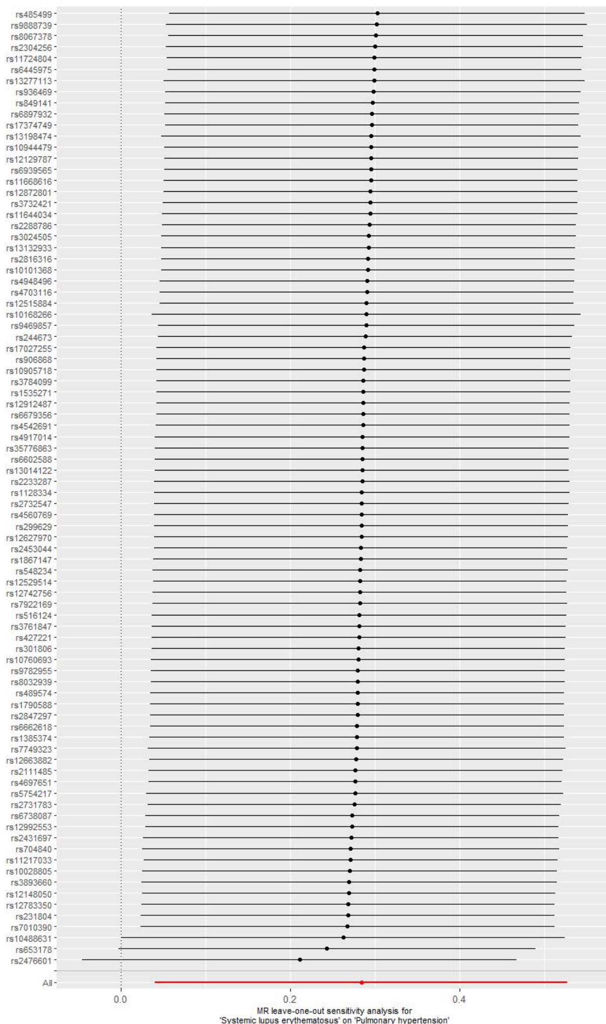
Supplementary Figure S1. Leave-one-out analysis, MR effect size, funnel plot and MR-Egger scatter plot for Systemic lupus erythematosus on Pulmonary Hypertension.
