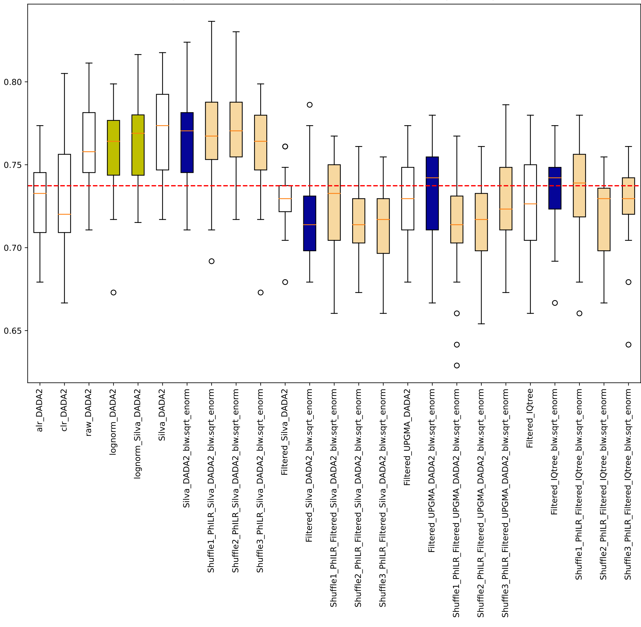
Vangay sklearn random forest manual 0.75training Accuracy Ethnicity
