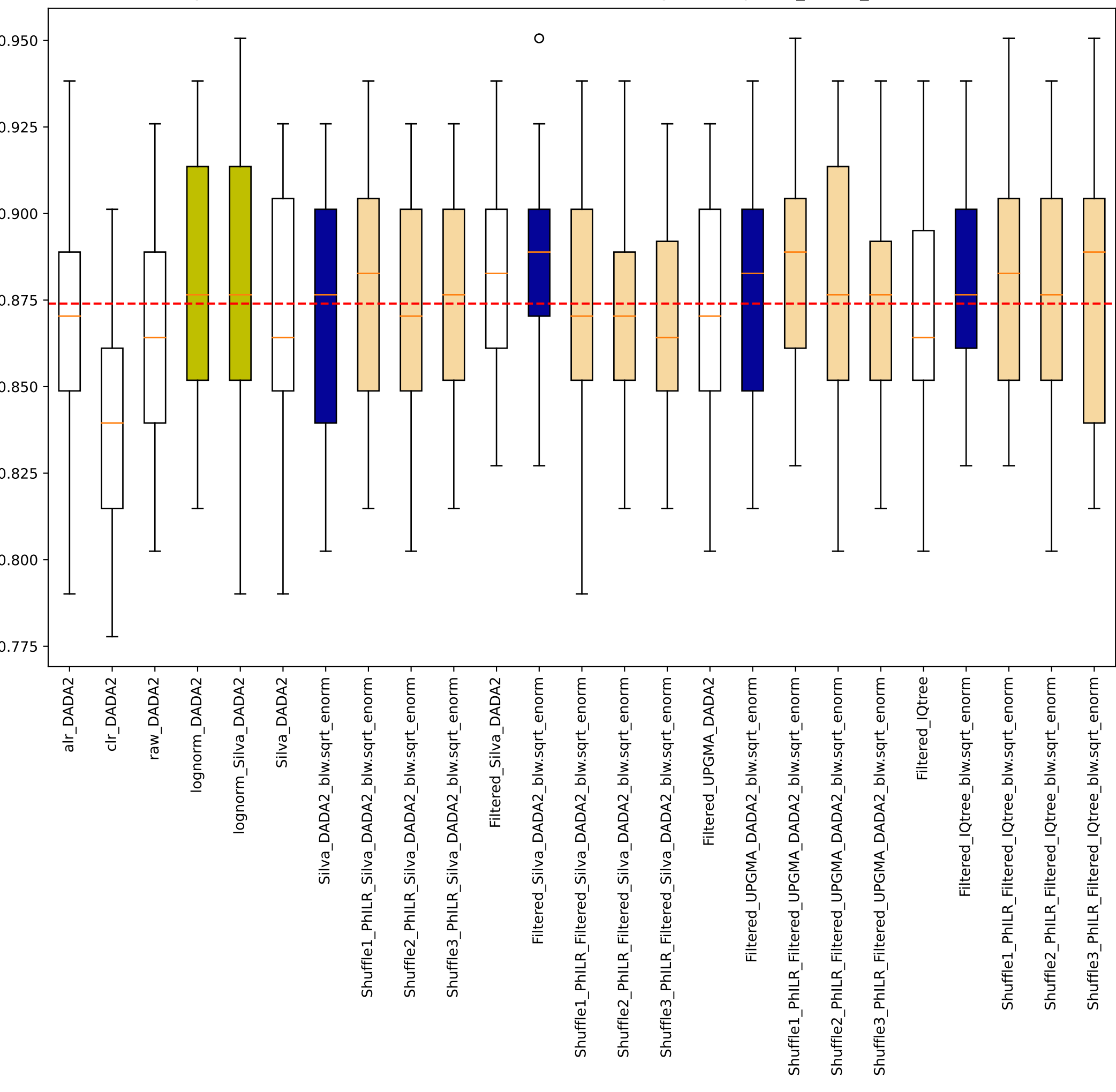
Noguera-Julian sklearn random forest manual 0.75training Accuracy host_sexual_orientation
