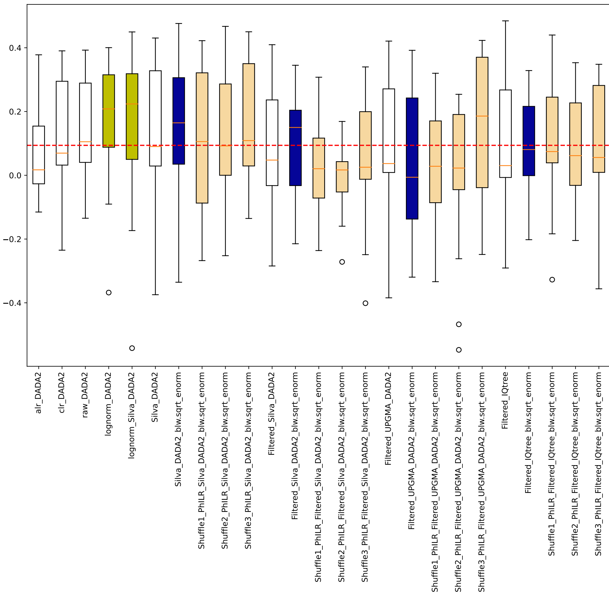
Noguera-Julian sklearn random forest manual 0.75training Accuracy CD4+_Tcell_counts
