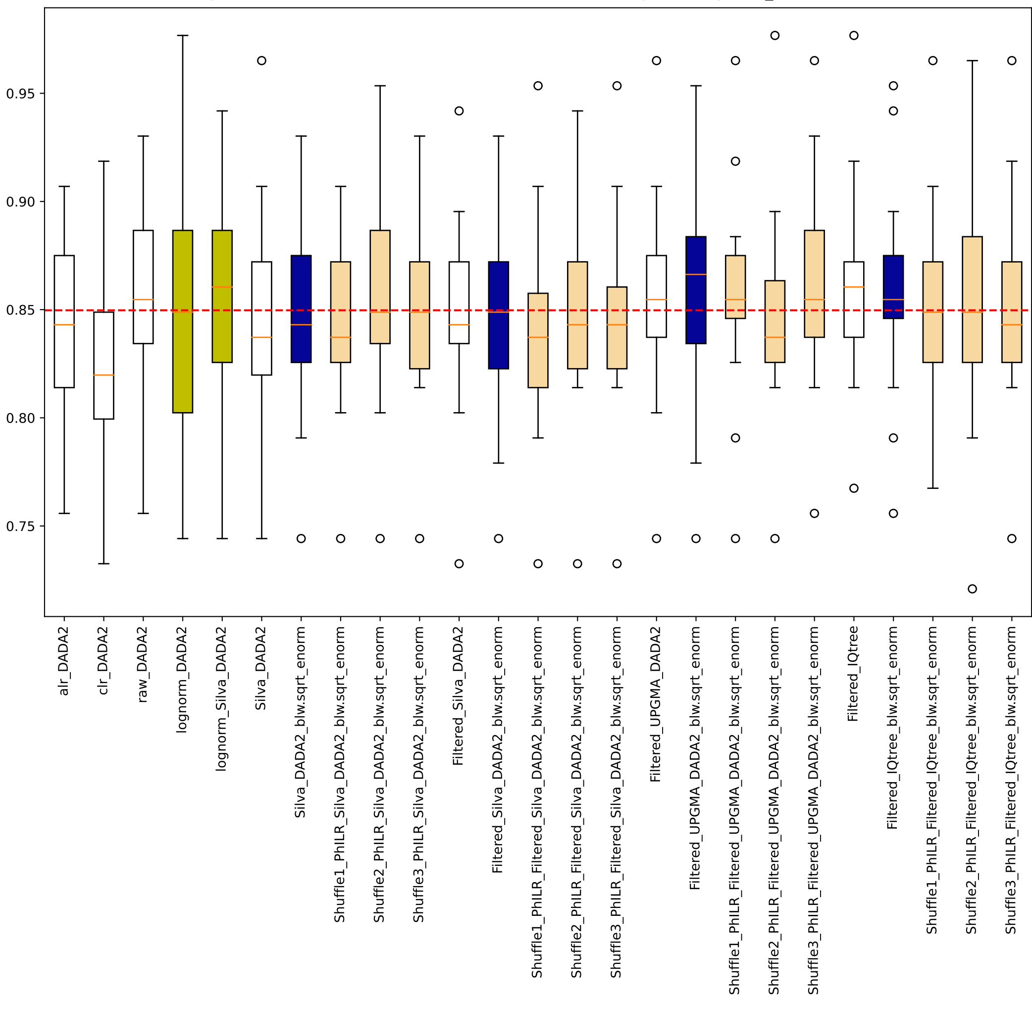
Noguera-Julian sklearn random forest manual 0.75training Accuracy HCV_coinfection
