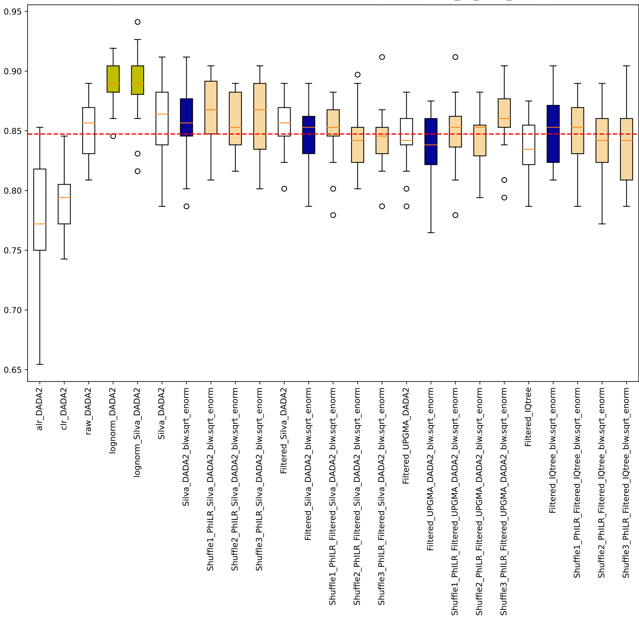
Noguera-Julian sklearn random forest manual 0.75training Accuracy geo_loc_name_country
