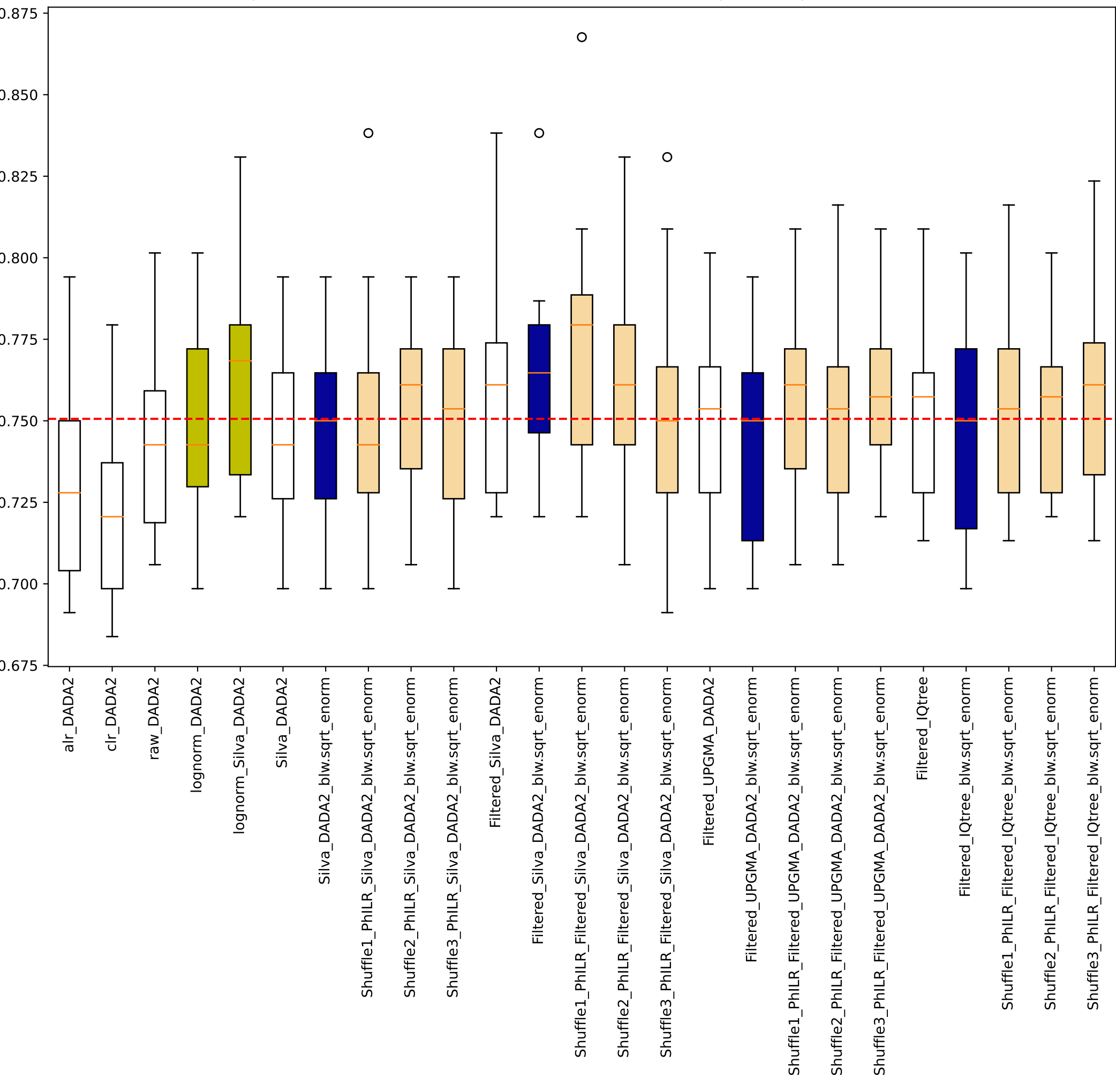
Noguera-Julian sklearn random forest manual 0.75training Accuracy ETHNICITY
