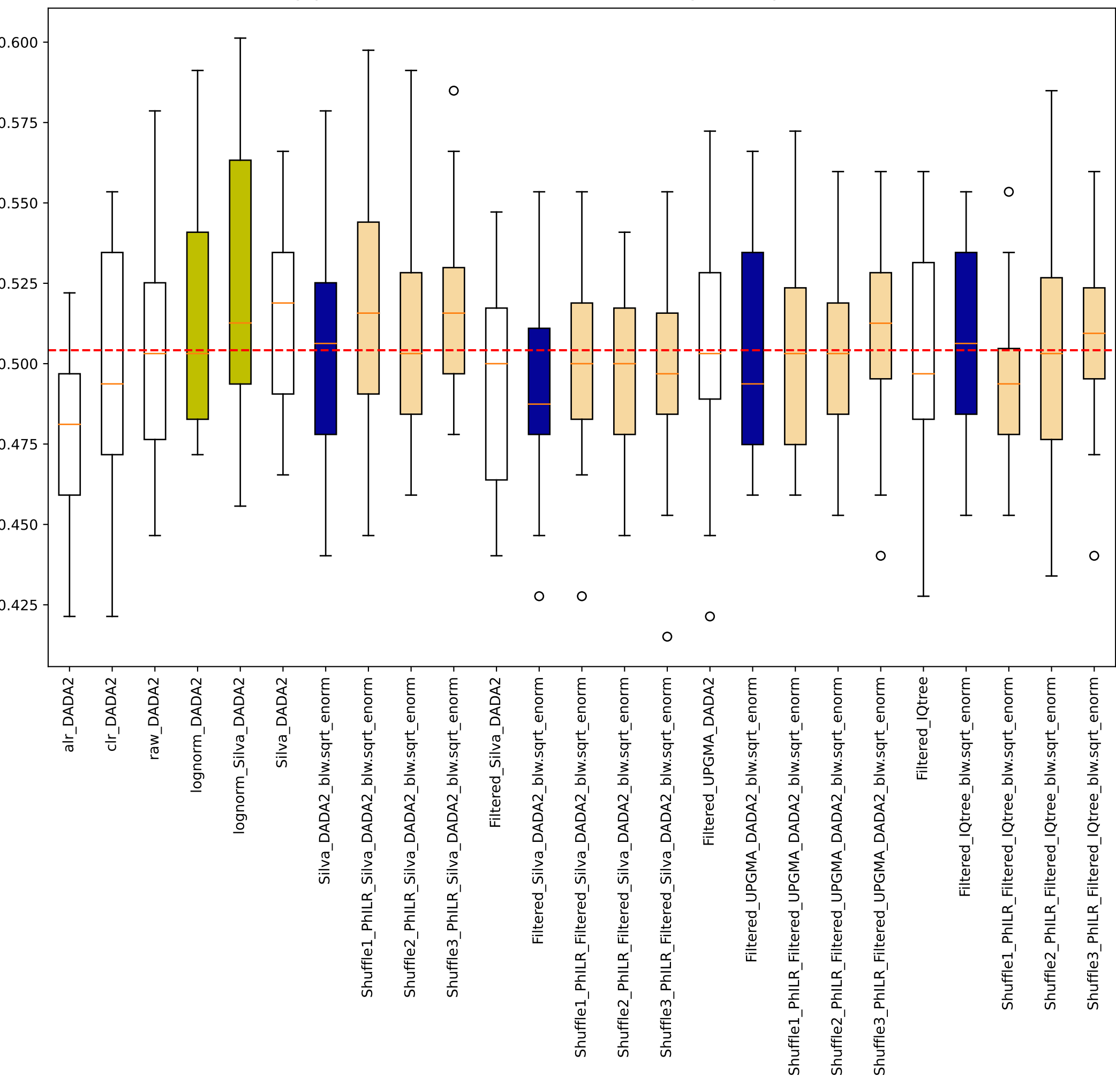
Vangay sklearn random forest manual 0.75training Accuracy BMI.Class
