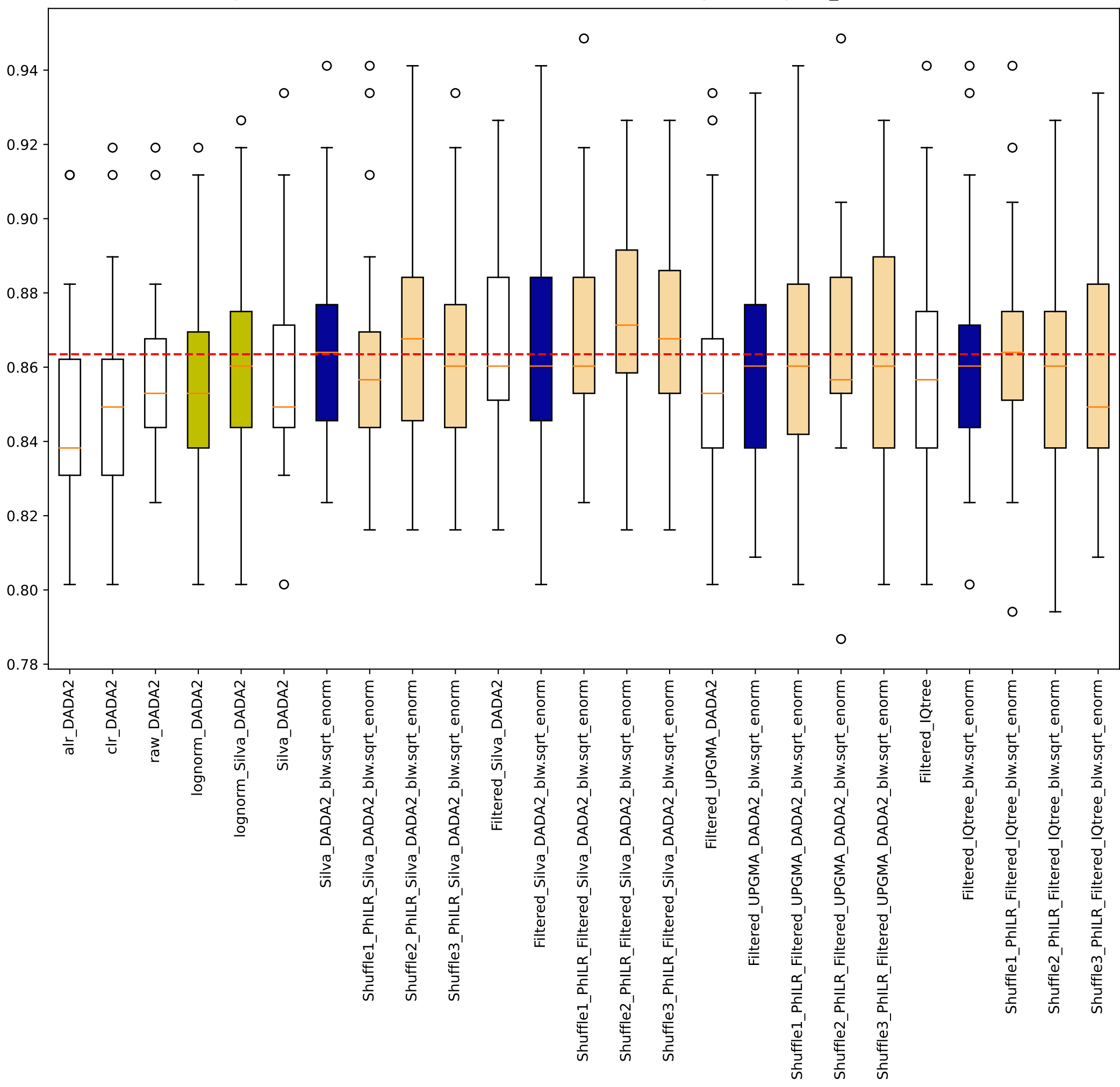
Noguera-Julian sklearn random forest manual 0.75training Accuracy HIV_serostatus
