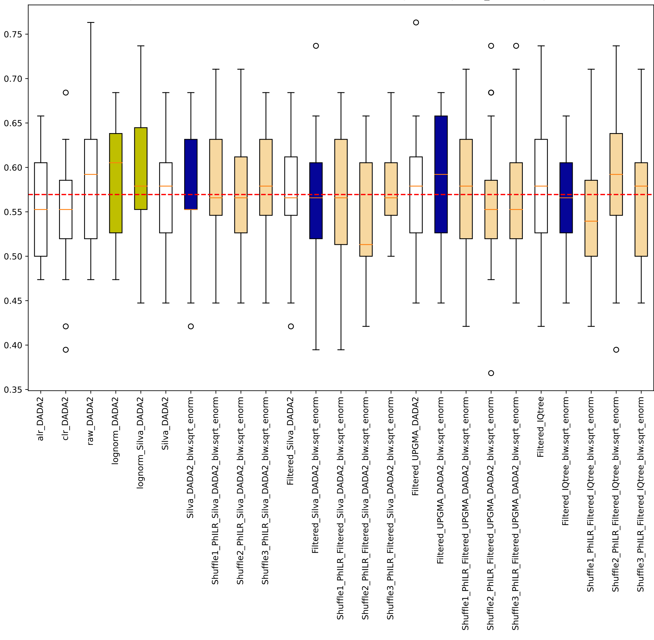
Noguera-Julian sklearn random forest manual 0.75training Accuracy stool_consistency
