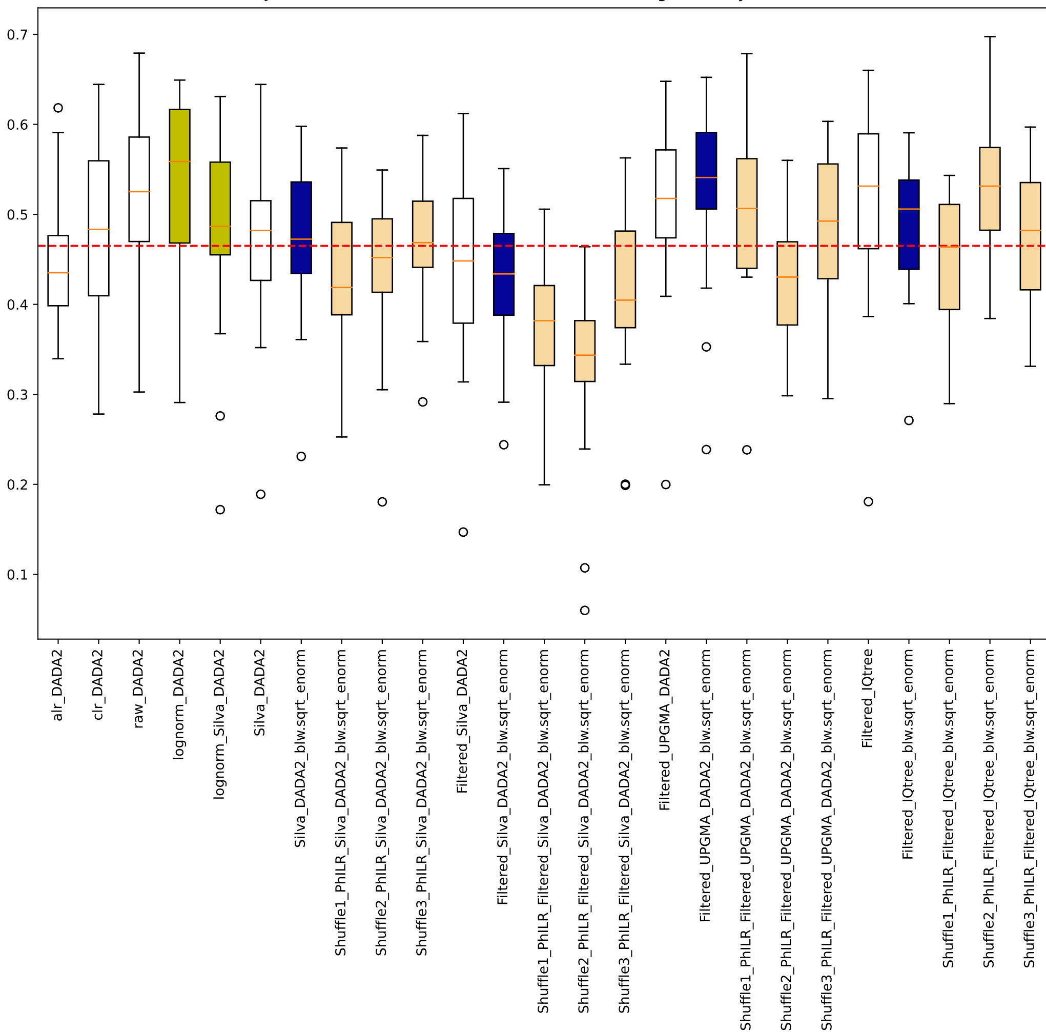
Jones sklearn random forest manual 0.75training Accuracy BMI
