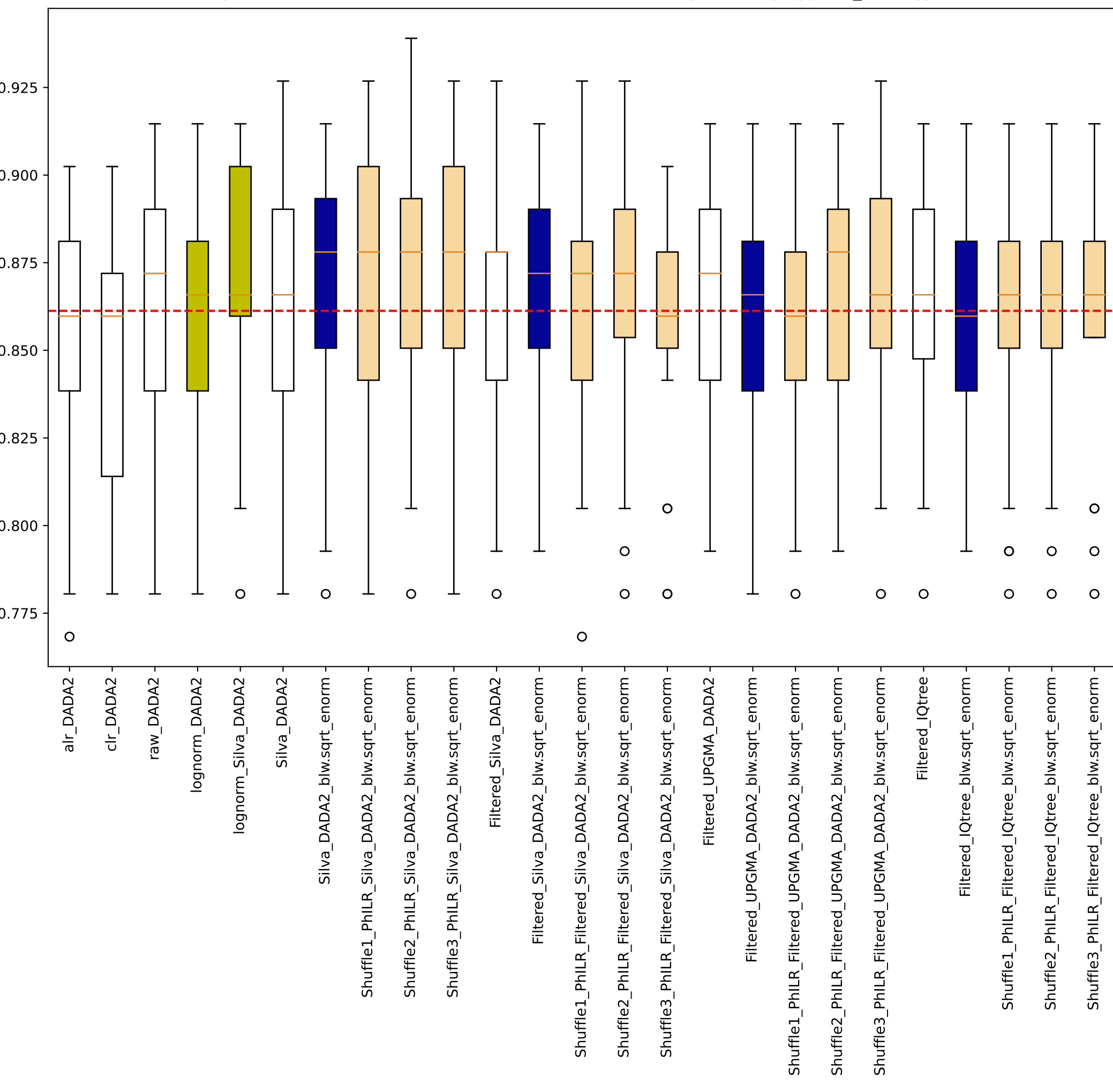
Noguera-Julian sklearn random forest manual 0.75training Accuracy Syphilis_serology
