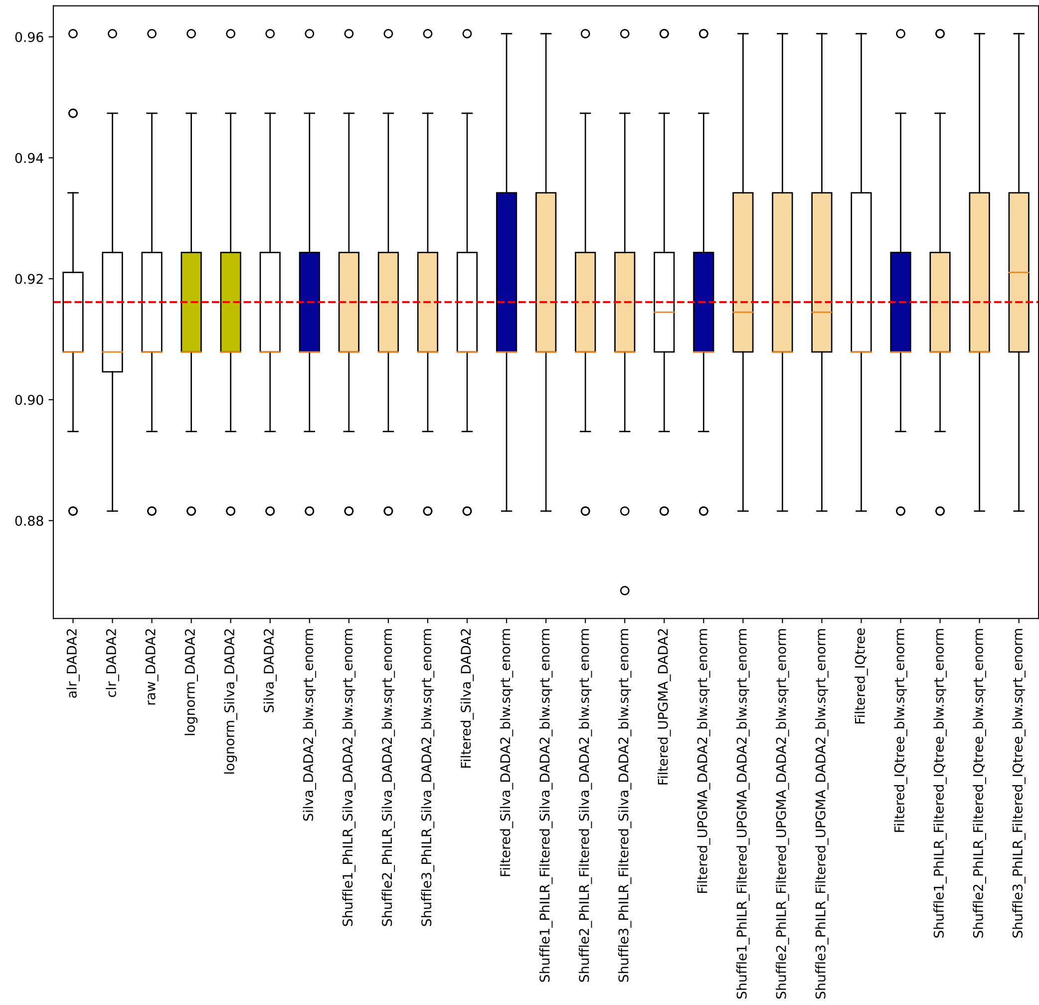
Noguera-Julian sklearn random forest manual 0.75training Accuracy PCR_Chlamydia_trachomatis
