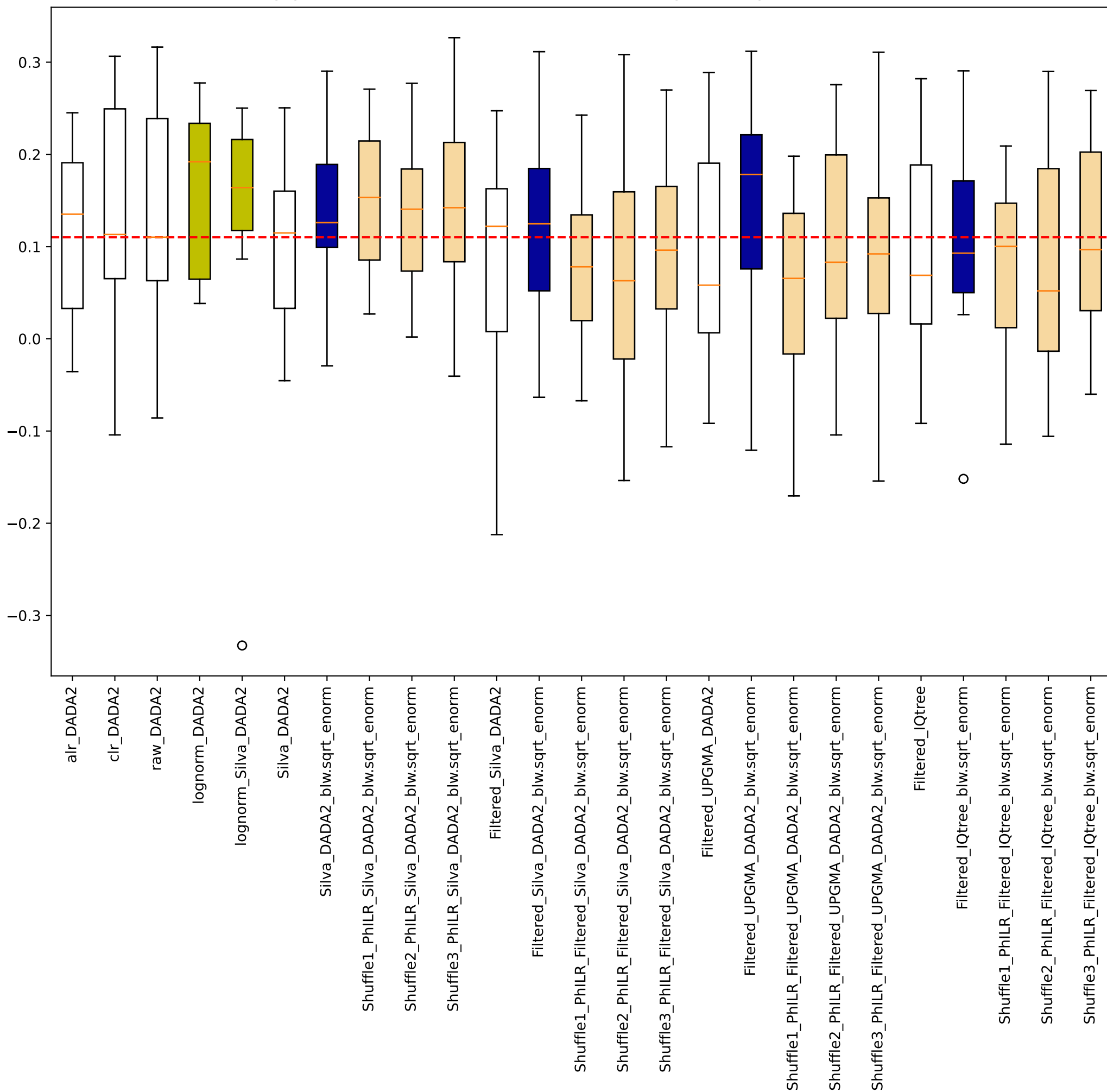
Vangay sklearn random forest manual 0.75training Accuracy Years.in.US
