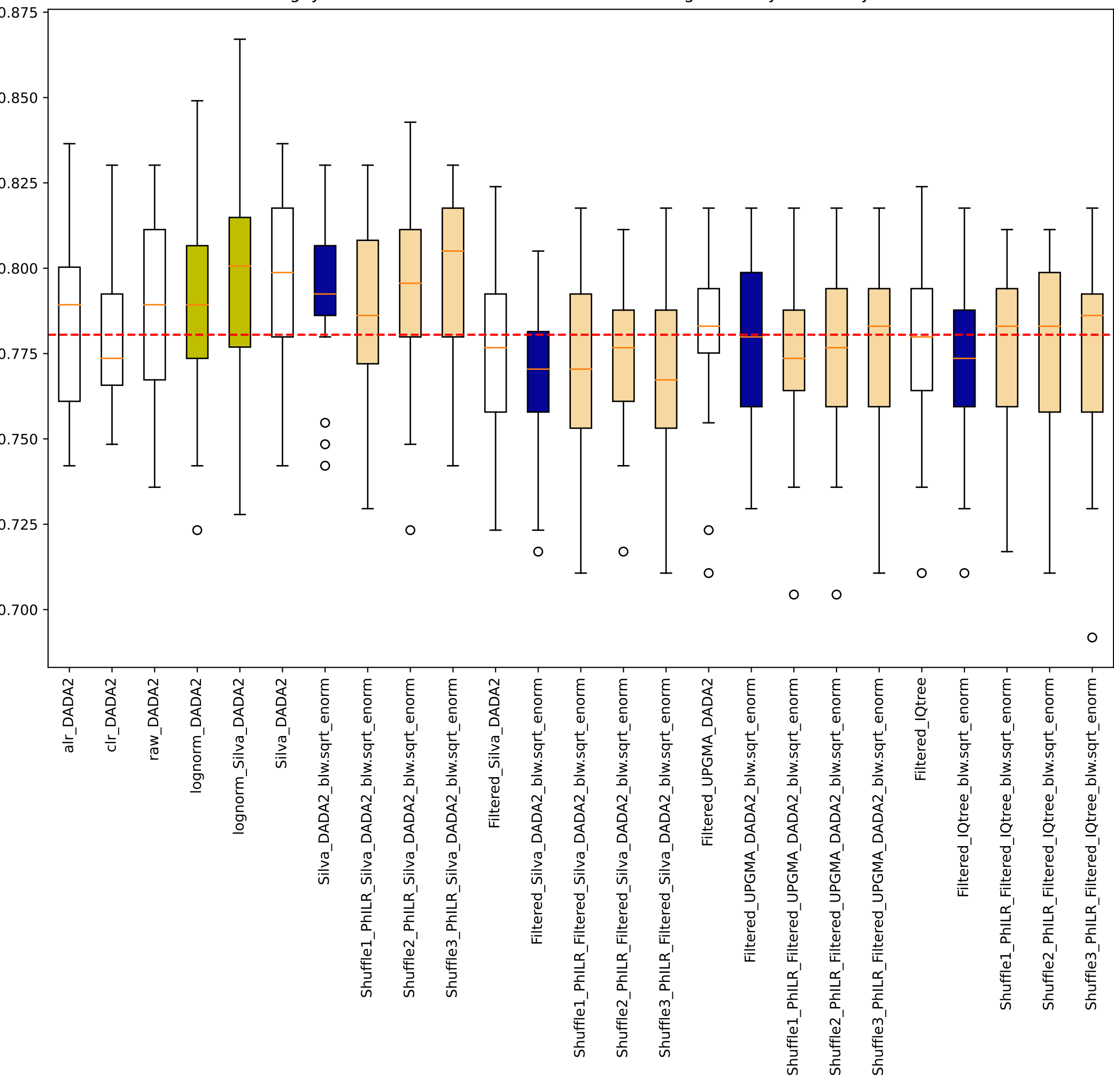
Vangay sklearn random forest manual 0.75training Accuracy Sub.Study
