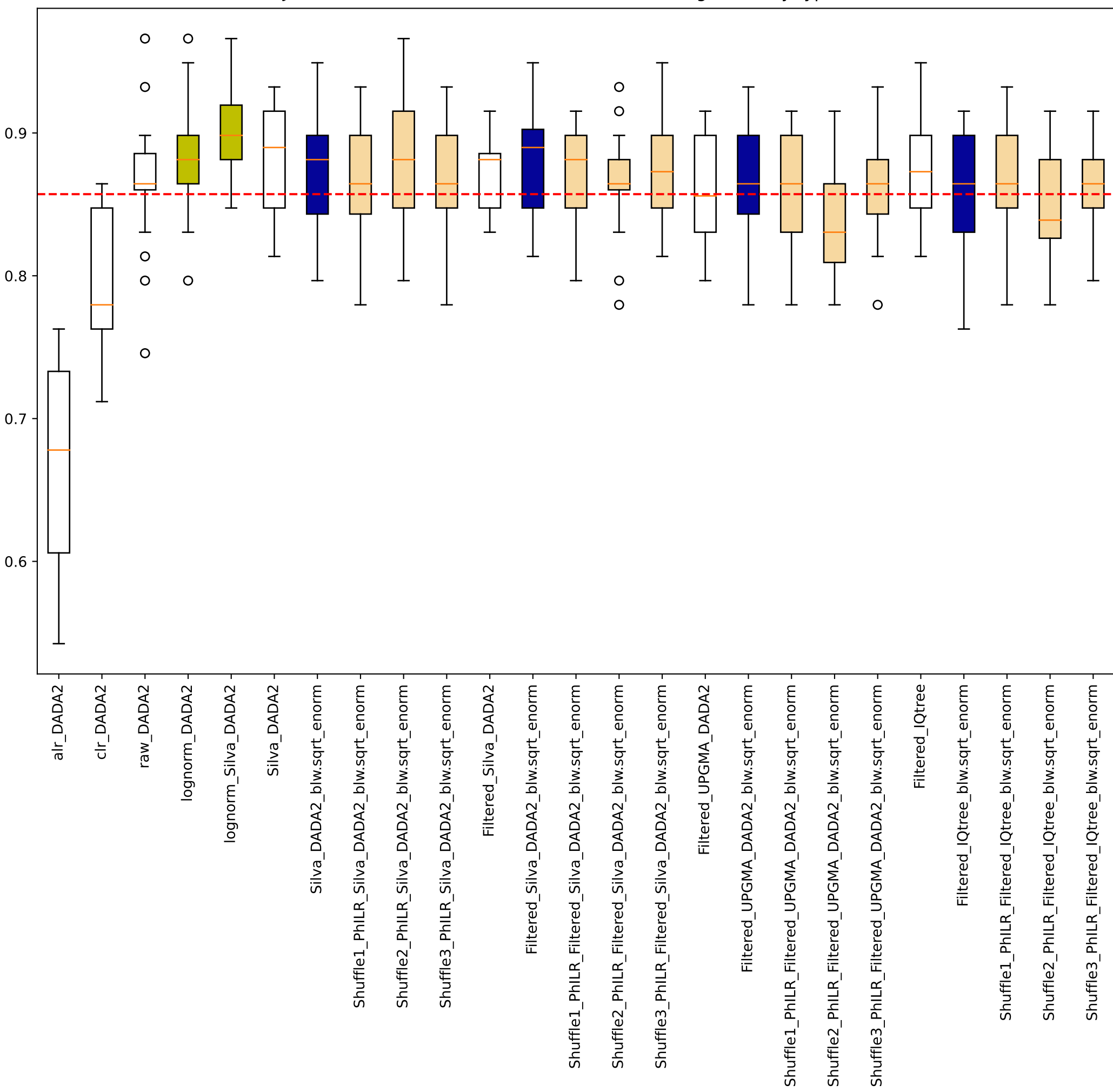
Jones sklearn random forest manual 0.75training Accuracy type
