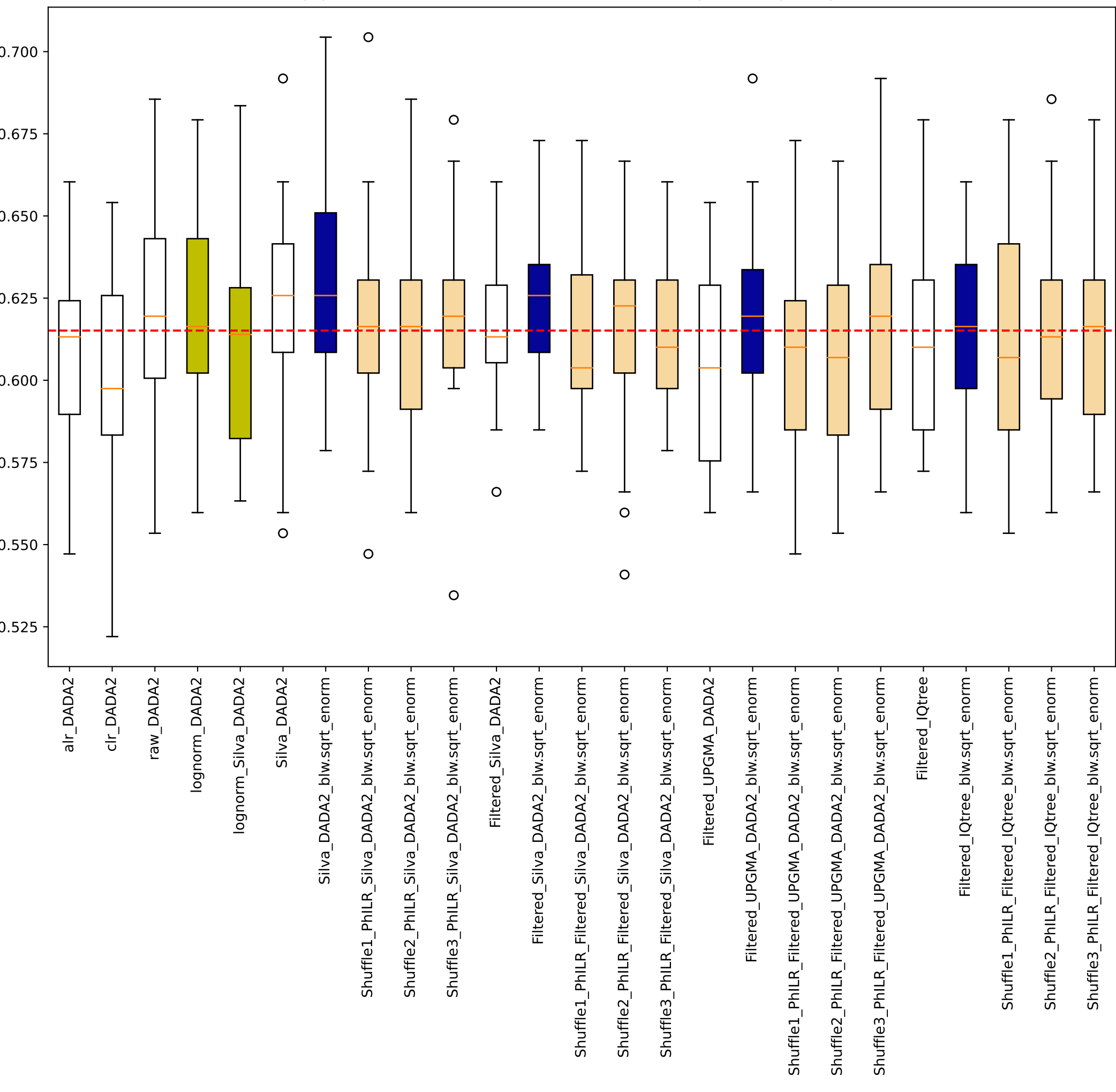
Vangay sklearn random forest manual 0.75training Accuracy Religion
