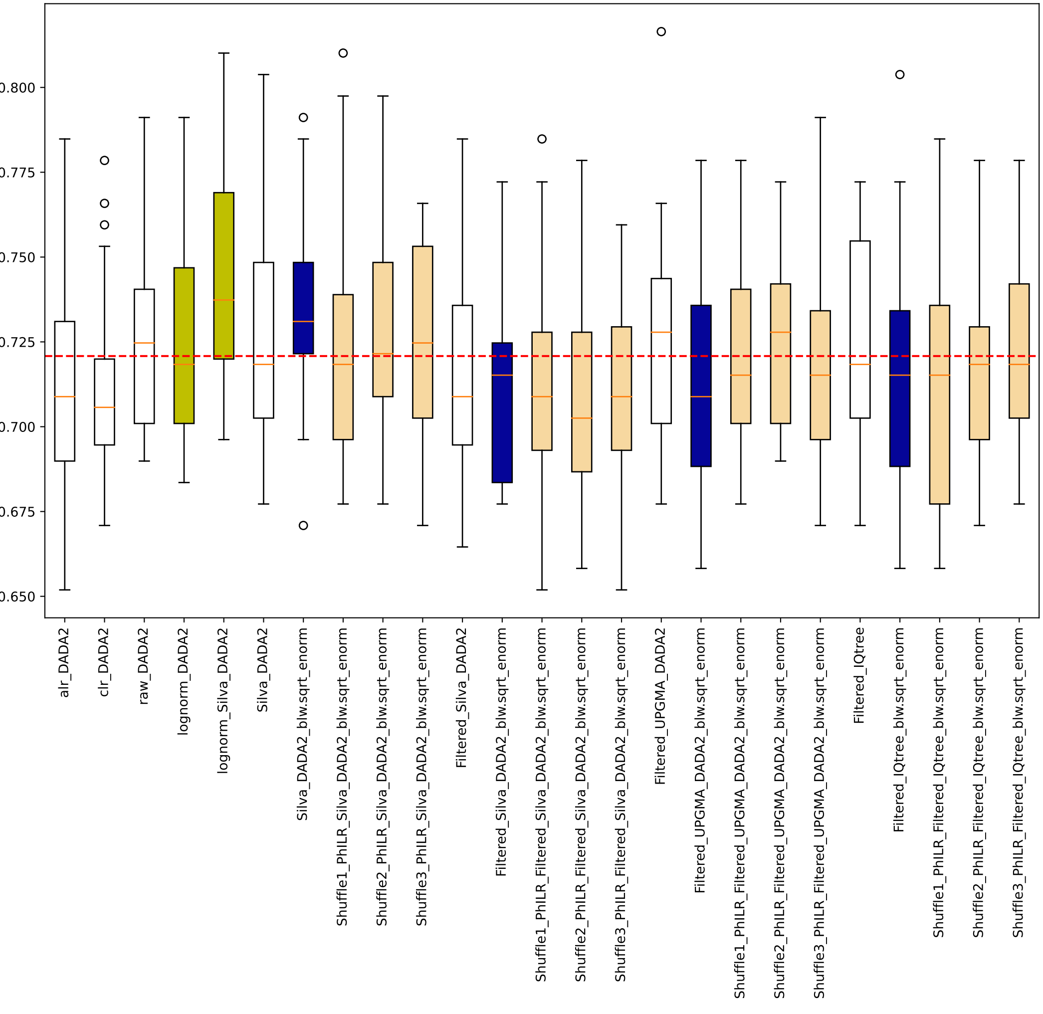
Vangay sklearn random forest manual 0.75training Accuracy Type.Birth.Location
