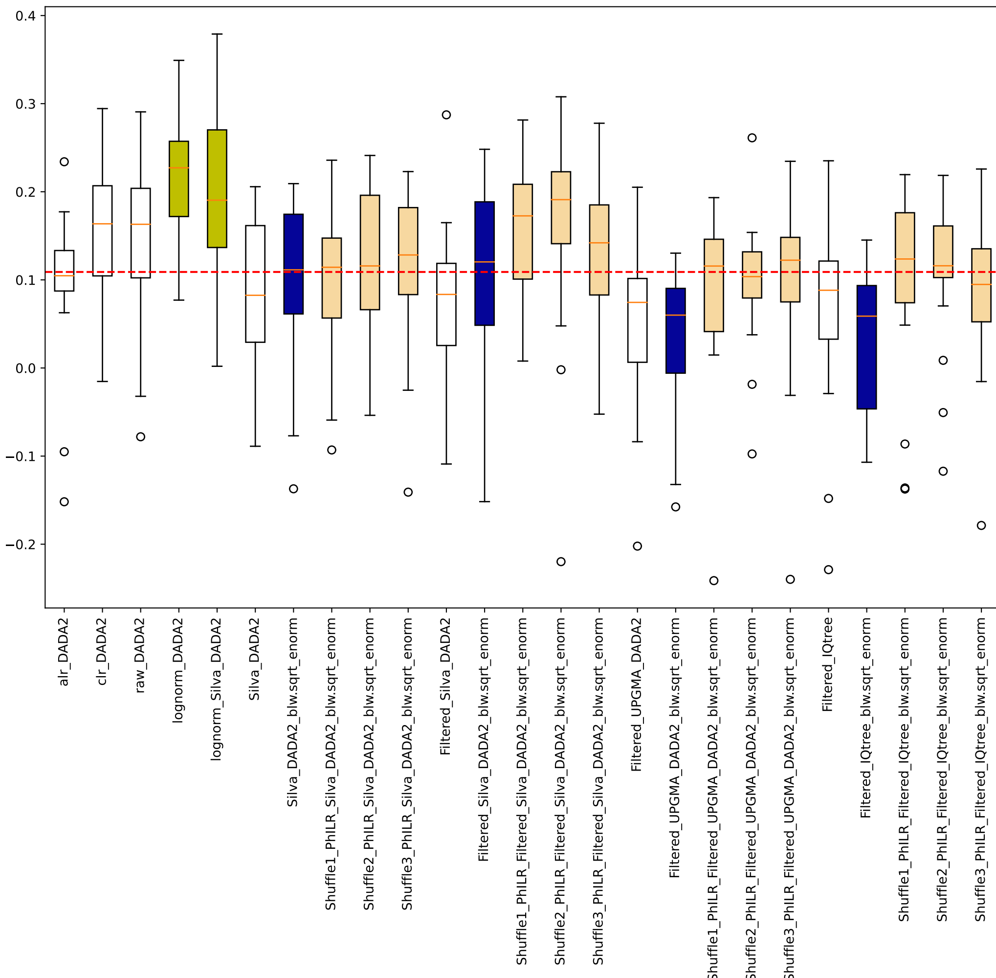
Noguera-Julian sklearn random forest manual 0.75training Accuracy host_deposition_frequency_per_day
