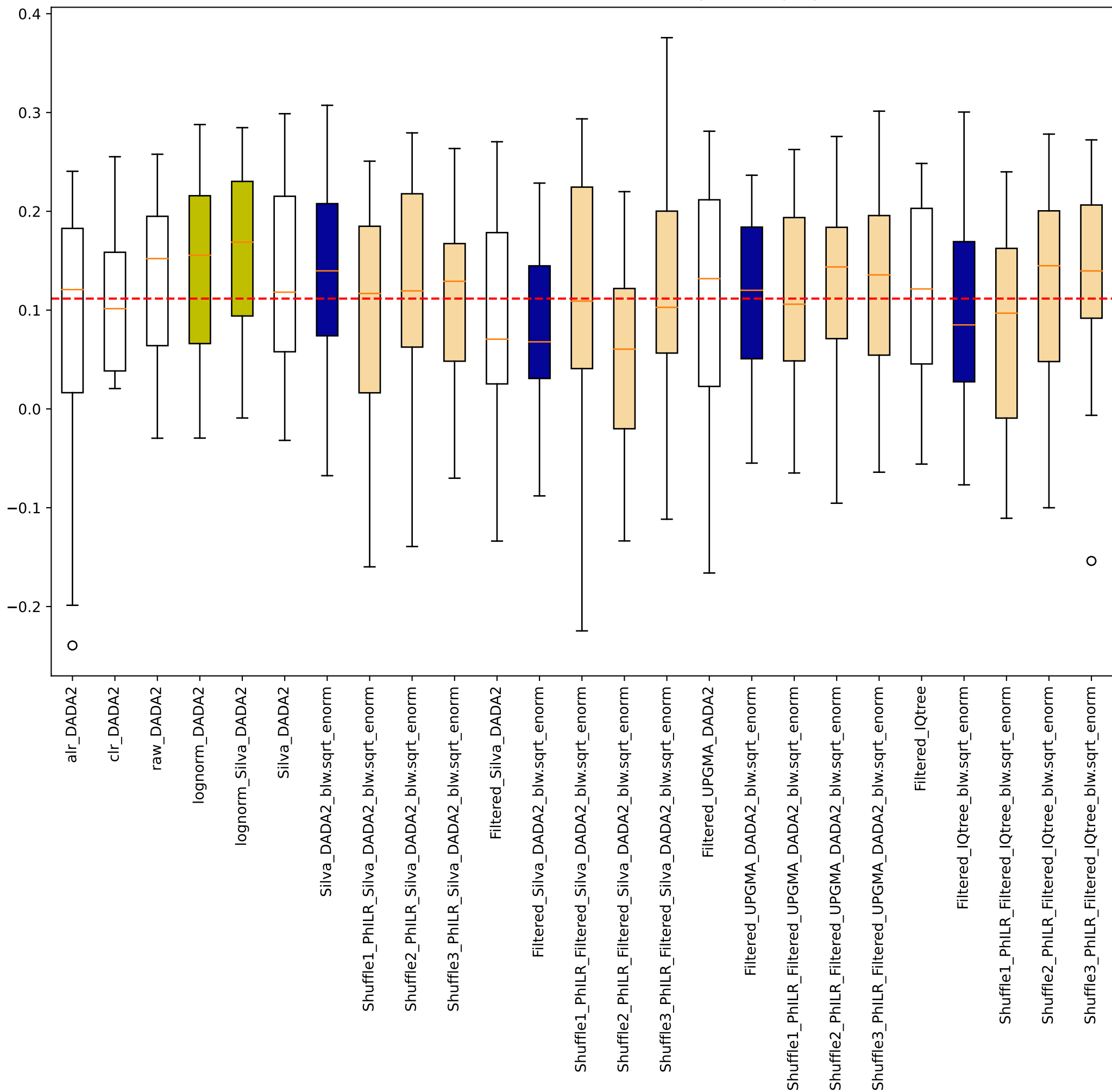
Zeller sklearn random forest manual 0.75training Accuracy Age
