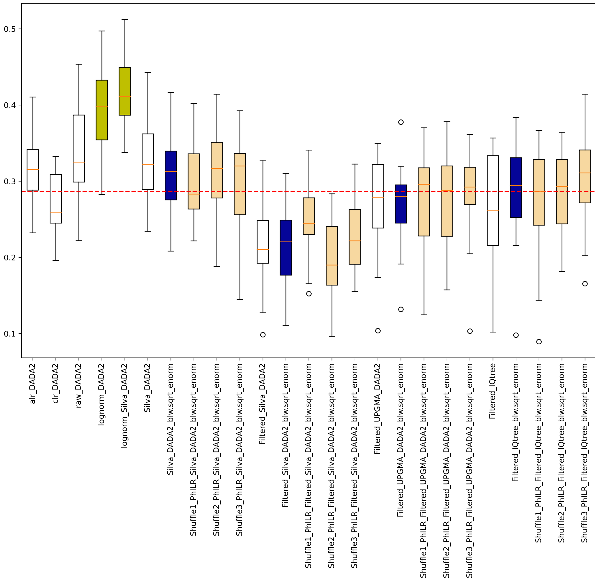
Noguera-Julian sklearn random forest manual 0.75training Accuracy Host_Age
