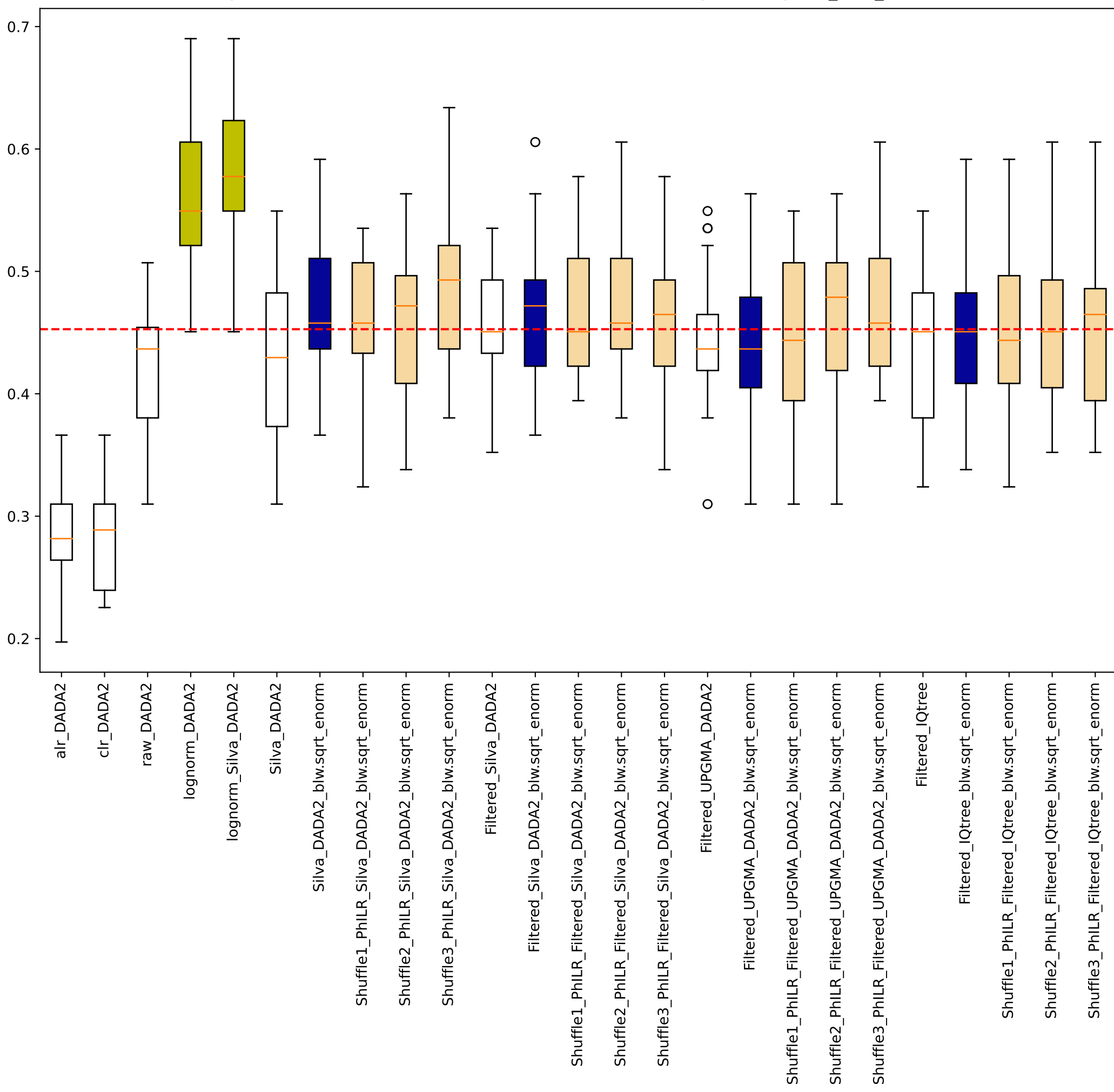
Noguera-Julian sklearn random forest manual 0.75training Accuracy HIV_viral_load
