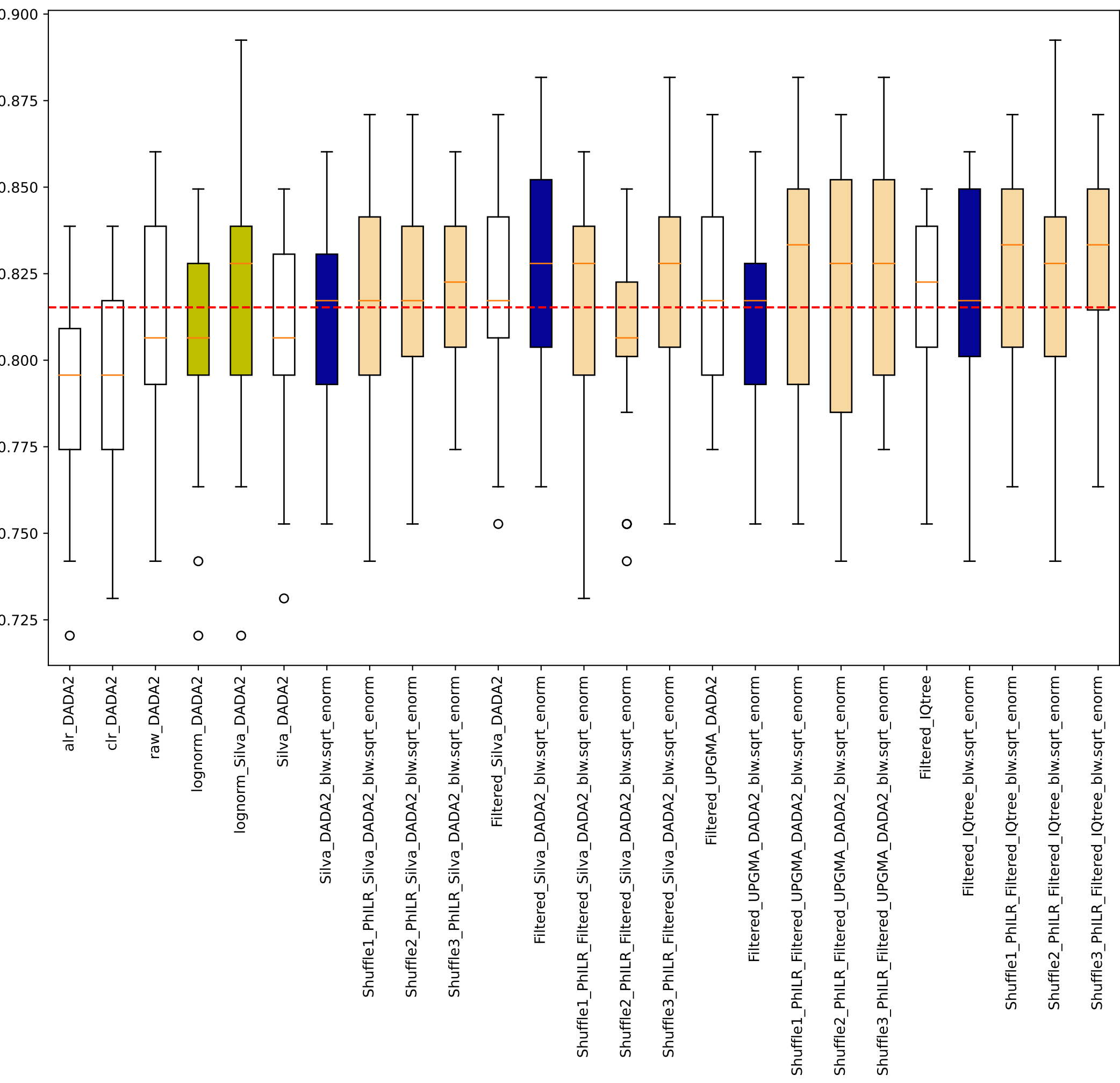
Noguera-Julian sklearn random forest manual 0.75training Accuracy host_allergy
