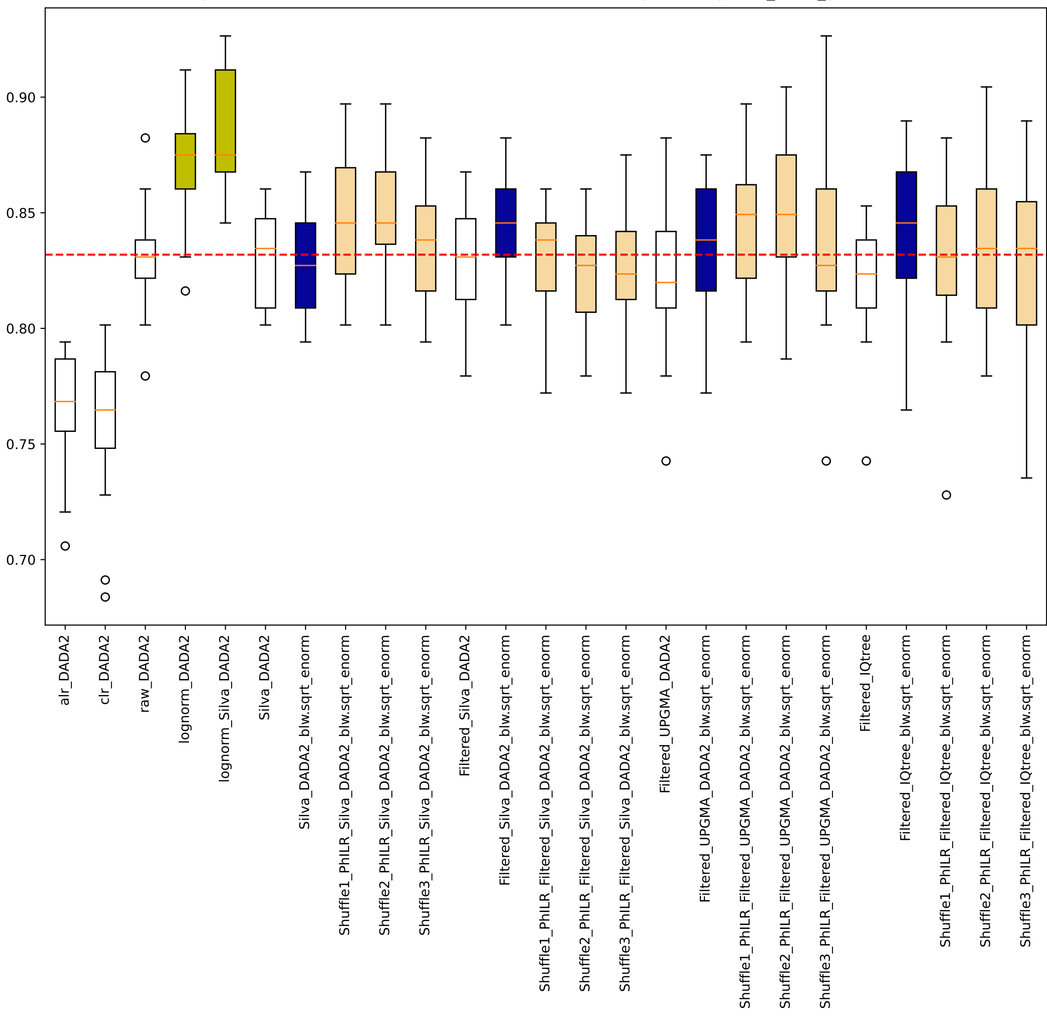
Noguera-Julian sklearn random forest manual 0.75training Accuracy host_other_gender
