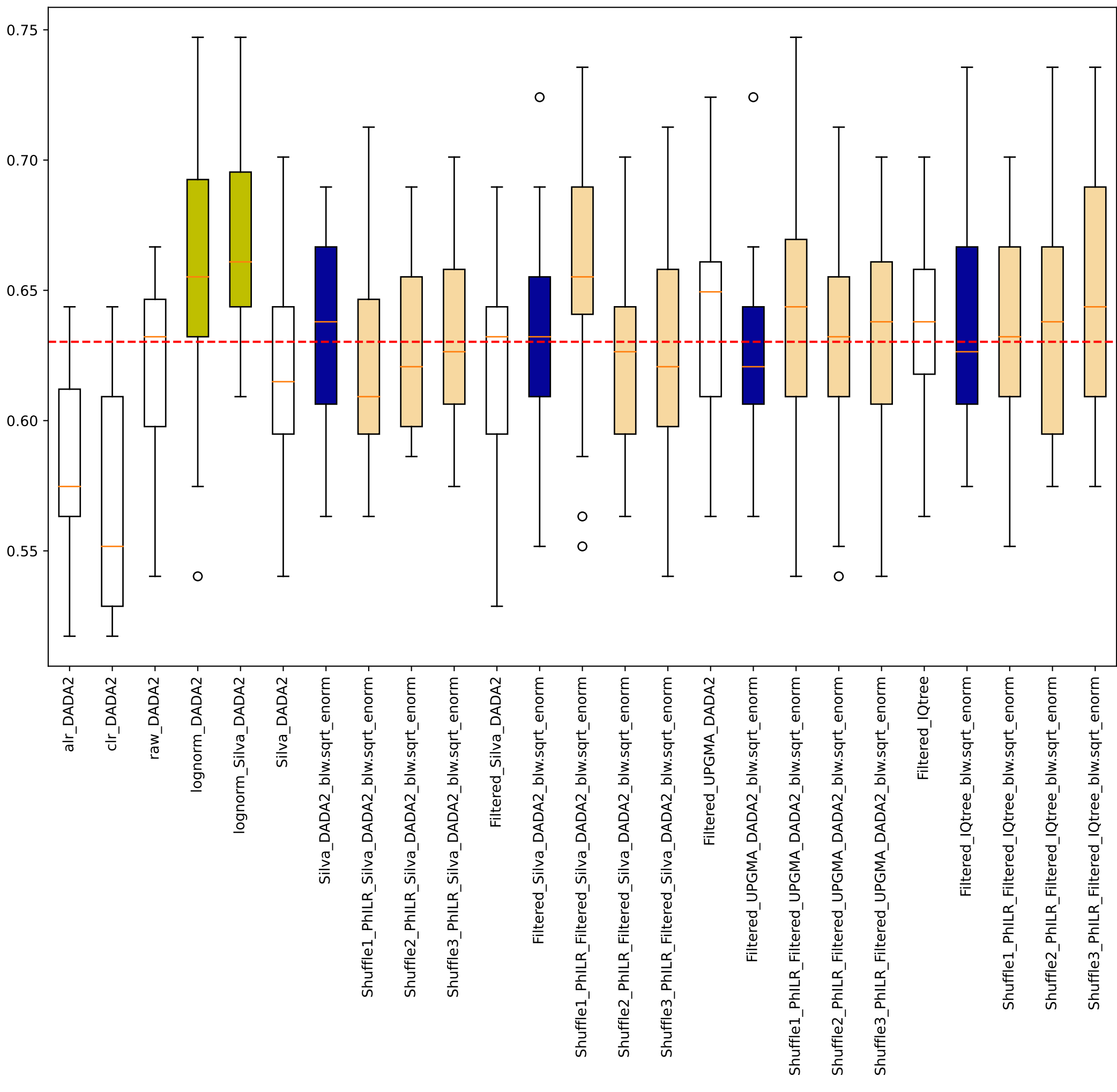
Noguera-Julian sklearn random forest manual 0.75training Accuracy Anal_cytology
