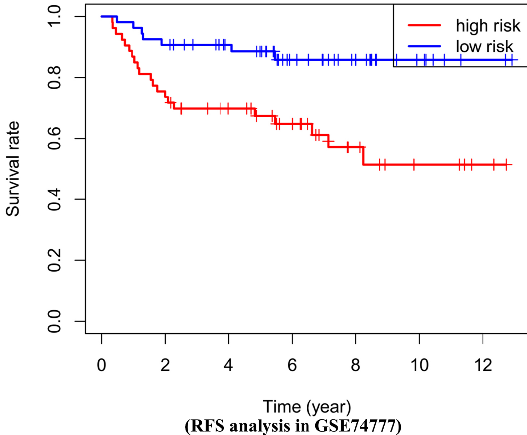
Supplementary Figure 2. LUSC patients (n=107) from the GSE74777 cohort. Survival analysis showed that patients in the high-risk group had a poorer 5-year RFS than those in the low-risk group ( P < 0.05 ).
