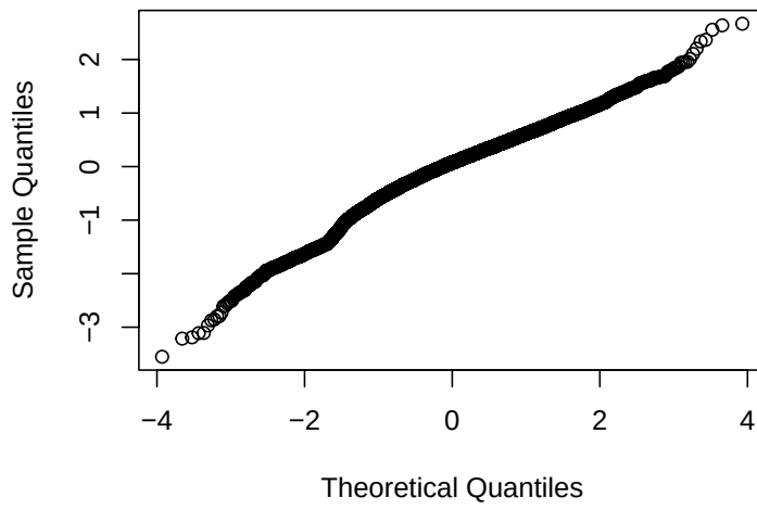
Figure A.2 QQ-plot of model residuals for log-transformed DV Duration Stay
