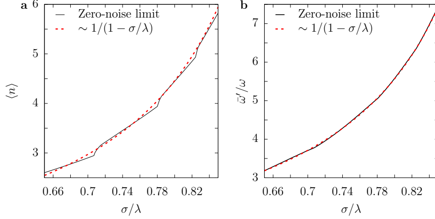
FIG. S2. Mean sizes and mean velocities of solitons in the zero-noise limit for f = 0.67 . (a) Mean size \langle n \rangle of solitons as a function of particle diameter \sigma . (b) Normalized mean angular velocity \bar{\omega}'/\omega in the corotating frame in dependence of \sigma . The black solid lines mark the exactly calculated results in the zero-noise limit, and the dashed red lines the approximate functional behavior according to equations (5) and (6) of the main text.
