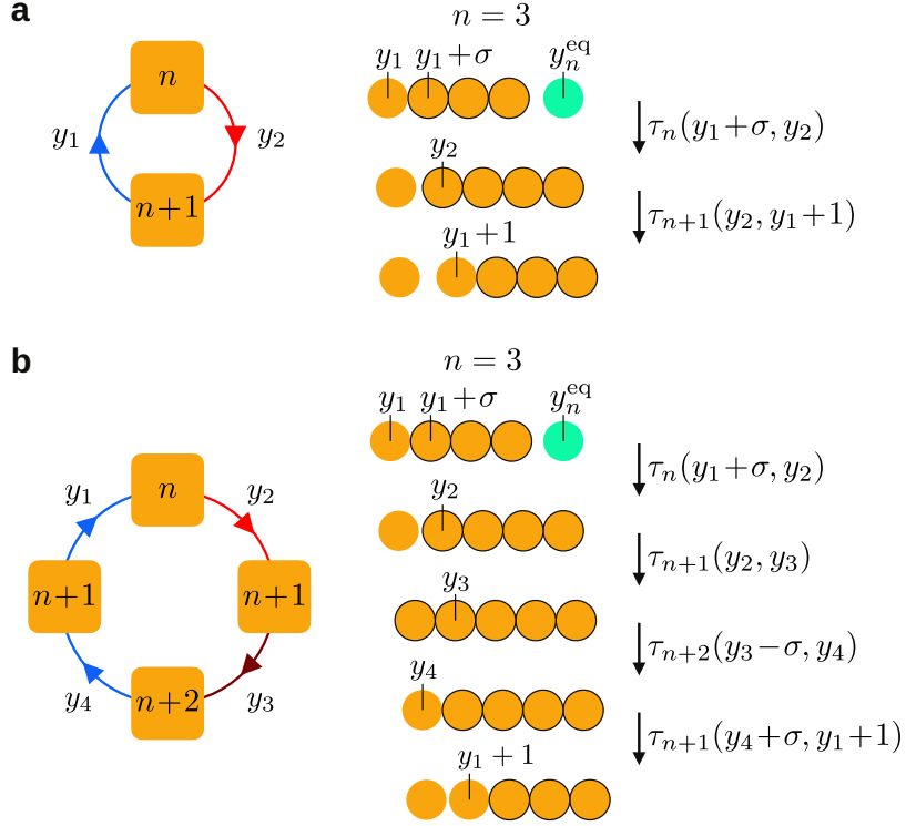
FIG. S1. Illustration of soliton types. Propagation of solitons is mediated by clusters of particles in contact, where the cluster size changes by detachments and attachments of single particles. Detachment events are marked by blue arrows and occur at the back end of clusters (back and front end refer to the cluster's direction of movement). Attachment events are marked by red arrows, where bright (dark) red arrows indicate attachments at the front (back) end of a cluster. Framed circles represent those particles that keep in contact with progressing time. Two types of solitons occur: (a) Type A soliton with core size n consisting of subsequent movements of an (n+1) - and n -cluster during one period. The (n+1) -cluster changes to an n -cluster due to the detachment of a single particle, if the (n+1) -cluster is at position y_1 \in [0, 1[ (the position of a cluster is always defined by the position of its leftmost particle). The n -cluster propagates until attaching to the resting particle at position y_n^{\text{eq}} , by which a new (n+1) -cluster is generated. Both the n - and (n+1) -cluster are at position y_n^{\text{eq}} - n\sigma at the moment of the attachment. The newly formed (n+1) -cluster continues to move until it reaches the position y_1 + 1 , where one cycle of the soliton motion is finished and the process starts anew. (b) Type B soliton with core size n consisting of subsequent movements of an (n+1) - n -, (n+1) - and (n+2) -cluster during one period. Starting with the detachment of a single particle from the (n+1) -cluster, analogous cluster moves occur as in the case of the type A soliton, until the attachment of the n -cluster to the resting particle at position y_n^{\text{eq}} . The newly formed (n+1) -cluster, however, now continues to move until the previously detached single particle reattaches at its back end. This happens when the (n+1) -cluster is at position y_3 and, accordingly, the single particle at position y_3 - \sigma . The (n+2) -cluster formed by the reattachment moves until reaching position y_4 , where the particle at its back end detaches again. The remaining (n+1) -cluster moves until reaching position y_1 + 1 , by which the soliton cycle is completed. The duration of the cluster movements is given by the functions \tau_n(a, b) in Eq. (S9a), where a and b denote the initial and final position of the cluster.
