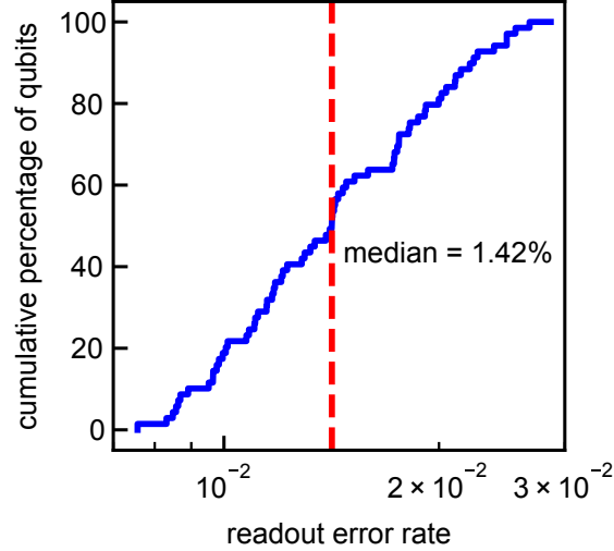
FIG. S2. Cumulative distribution of the readout error across the 70 qubit superconducting quantum processor with a dashed line indicating the median value of 1.42\% .
