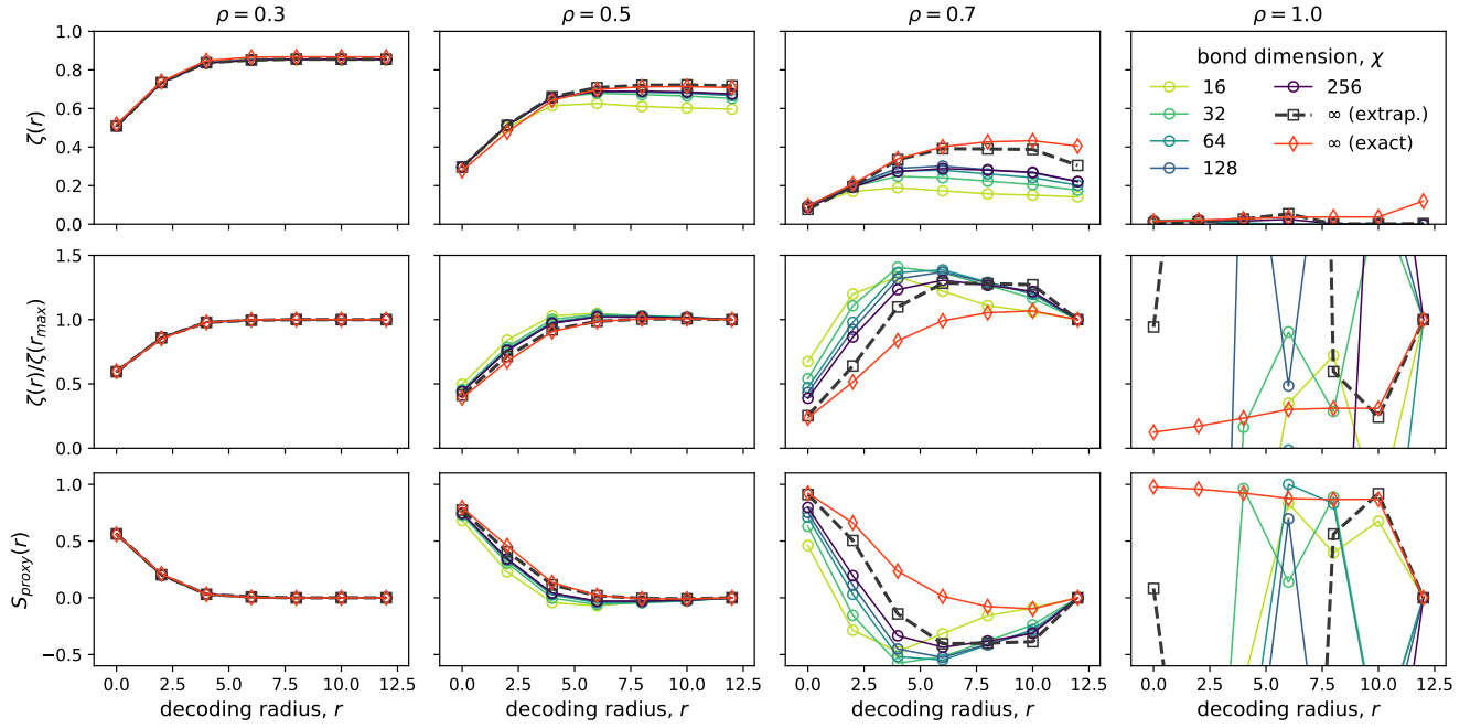
FIG. S17. Results of approximate decoding of N = 70 experimental data based on MPS with bond dimension \chi = 16, \dots, 256 , at four values of \rho across the phase diagram. Top row: decoded order parameter \zeta as a function of decoding radius r . Middle row: error-mitigated order parameter \tilde{\zeta}(r) = \zeta(r)/\zeta(r_{\max}) . Bottom row: error-mitigated proxy entropy \tilde{S}_{\text{proxy}}(r) = -\log_2[(1 + \tilde{\zeta}(r)^2)/2] . Along with the fixed- \chi data (circles), we show an extrapolation to \chi \rightarrow \infty (squares) and a comparison with the results of decoding based on exact simulation (diamonds) as in Sec. VI. The extrapolation is obtained from fits to an empirical ansatz \alpha/\log(\chi) + \beta on \chi = 32, \dots, 256 .
