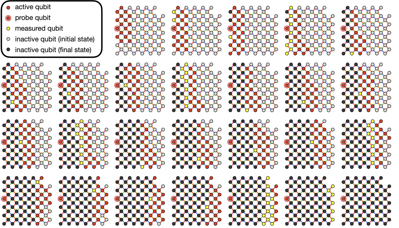
FIG. S14. Classical simulation algorithm for quantum circuits on N = 70 qubits (depth T = 5 ). The active subsystem A is indicated in red. It always includes the probe P (circled qubit). Light gray qubits make up the initial-state subsystem I (not yet part of the wavefunction), black qubits are the final-state subsystem F (already projected out and not part of the wavefunction anymore). Yellow qubits are projected out right before the evolution step in each panel. The active subsystem sweeps the chip from left to right and the simulation terminates when all qubits (except the probe) have been measured out. At each step in the simulation, the active subsystem contains at most 20 qubits.
