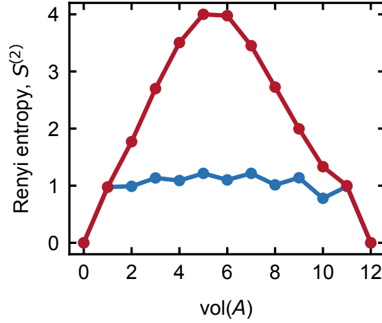
FIG. S7. Results of an exact numerical simulation of second Renyi entropy as a function of the volume of a subsystem A for experiment implemented in Fig. 2 of the main text. The curves agree qualitatively well with the experimental results.
