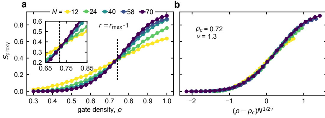
FIG. S15. Simulated decoding of probe qubit (cf. Fig. 4 in the main text). (a) Simulated proxy entropy S_{\text{proxy}} at decoding radius r = r_{\text{max}} - 1 as a function of \rho for all system sizes studied. Vertical dashed line indicates the estimated \rho_c = 0.72 . Inset: zoomed-in finite-size crossing. (b) Scaling collapse of the data vs (\rho - \rho_c)N^{1/(2\nu)} with \rho_c = 0.72 and \nu = 1.3 .
