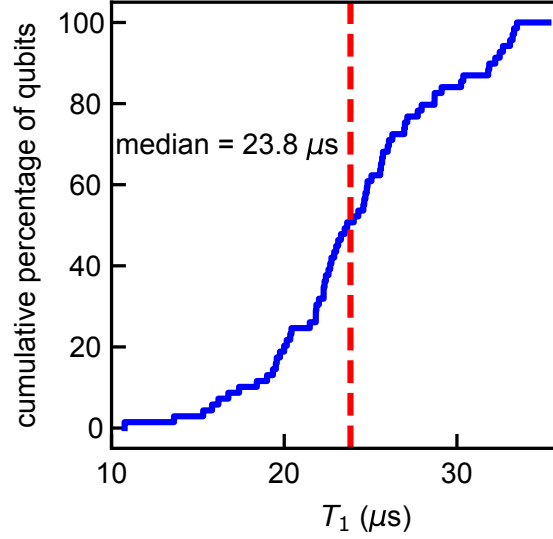
FIG. S1. Cumulative distribution of T_1 across the 70 qubit superconducting quantum processor with a dashed line indicating a median value of 23.8 \mu\text{s} .
