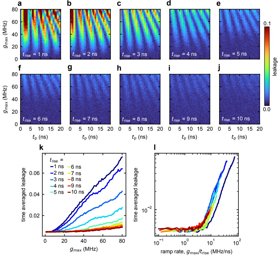
FIG. S5. a-j , Leakage measured as a function of the coupling strength g_{\max} and hold time t_p for fixed values of the rise time t_{\text{rise}} . k , The time averaged leakage (averaged over the range 0 < t_p < 20 ns) as a function of g_{\max} for different values of t_{\text{rise}} . The time averaged leakage plotted as a function of the ramp rate g_{\max}/t_{\text{rise}} for different t_{\text{rise}} .
