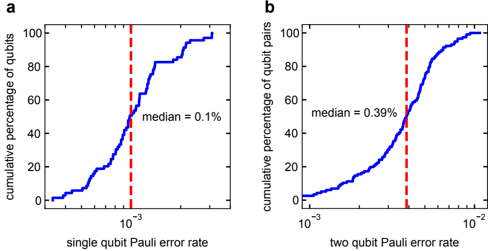
FIG. S3. a , b , Cumulative distributions of the single-qubit Pauli error ( a ) and two-qubit iSWAP-like Pauli error ( b ) across the 70 qubit superconducting quantum processor. We find median values of 0.10% and 0.39% for the single-qubit and iSWAP-like errors, respectively.
