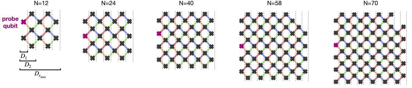
FIG. S13. The approximately square geometries of N = 12, 24, 40, 58 , and 70 qubits used in the decoding and finite size analysis experiment of Fig. 4 in the main text. The bond colors denote the gate sequence ((orange, blue, green, red, orange)). For each grid we show the probe qubit and the decoding patches D_1, \dots, D_{r_{\max}} employed in the decoding algorithm (dashed lines).
