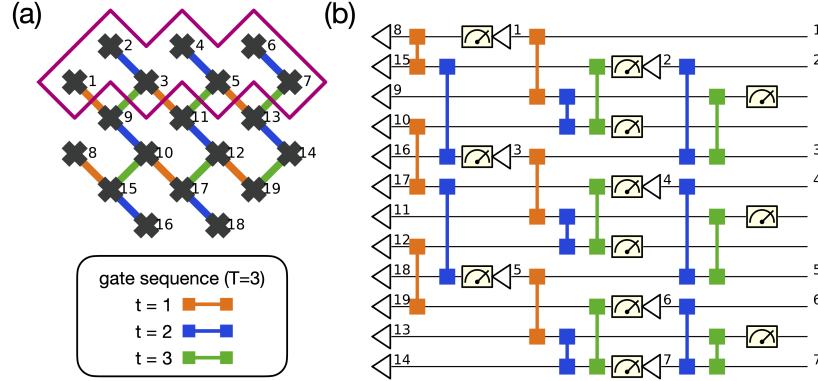
FIG. S12. Exact mapping of 2D shallow circuit used in Fig. 3 of the main text, for depth T = 3 , to 1D monitored circuit. (a) Shallow 2D circuit architecture. Qubits are numbered from 1 to 19; qubits Q_1 through Q_7 (purple contour) make up the final state. (b) Equivalent 1D monitored circuit. White triangles represent resets to |0\rangle states after measurement. Numbers on each qubit wire indicate the corresponding location in the 2D circuit (panel a). The circuit acts on 12 qubits but the final state involves only 7 of them (indicated by numbers on the right), the remaining 5 are decoupled by measurements.
