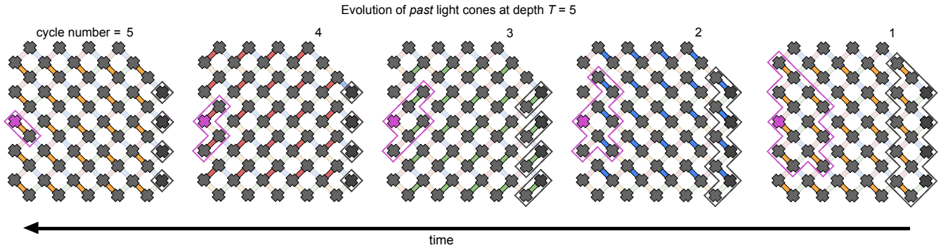
FIG. S16. Determination of the past light cones of the probe qubit (pink) and qubits along the right-most column (black) of the N = 58 geometry. We begin with the final cycle of two qubit operations at depth T = 5 and calculate the past light cone by going backward in time until we reach the first cycle of the circuit. The two subsystems have non-overlapping past light cones and are therefore causally disconnected.
