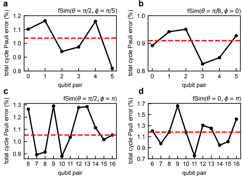
FIG. S6. a-d , Total cycle Pauli error of the fSim( \pi/2, \pi/5 ) (iSWAP-like), fSim( \pi/8, 0 ), fSim( \pi/2, \pi ) (SWAP), and fSim( 0, \pi ) (CZ), gates, respectively, as measured by cross entropy benchmarking (XEB) for the qubit pairs that utilized each gate. Red dashed line corresponds to the median.
