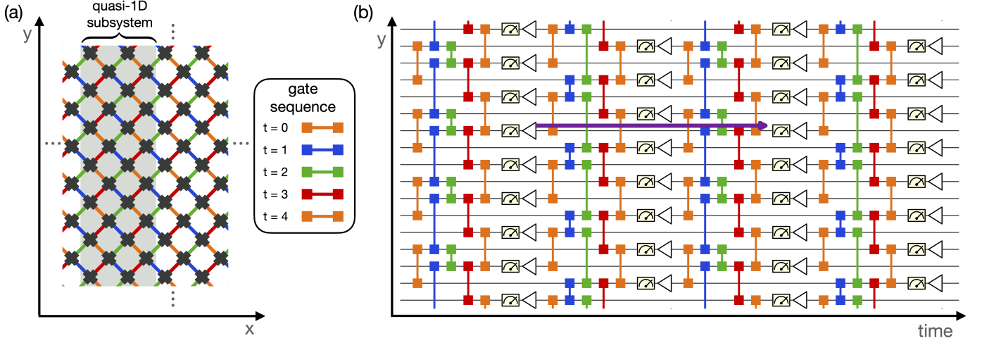
FIG. S11. Mapping of (2 + 1) -dimensional shallow circuits to (1 + 1) -dimensional monitored circuits. (a) 2D circuit architecture and gate sequence. (b) Equivalent 1D monitored circuit. Each measurement is followed by a reset to the |0\rangle state (white triangles). The purple arrow represents the “life cycle” of a qubit in the dynamics, from initialization in |0\rangle through the depth-5 gate sequence (orange, blue, green, red, orange), to final measurement. The circuit architecture is periodic in space and time.
