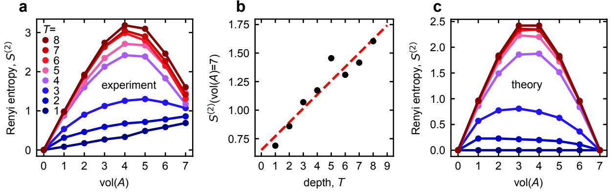
FIG. S8. a , Experimentally measured second Renyi entropy as a function of a sub-system A of the chain of 7 qubits at various depths without error mitigation. b , Second Renyi entropy of the entire 7 qubit chain after measurement of the lower 12 qubits as a function of circuit depth. The entropy grows approximately linearly due to decoherence in the system. Dashed line is a linear fit and intercepts the y -axis at a non-zero value, which we attribute to readout error. c , Exact numerical simulation of the second Renyi entropy as a function of the volume of a sub-system A of the 7 edge qubits at the same depths as in a . The results agree qualitatively well with the error-mitigated data presented in the main text.
