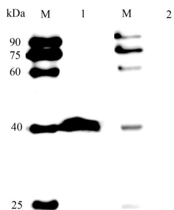
Fig. S1 Western-blotting analysis of NbGAPDH in N. bombycis .
