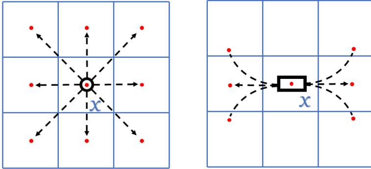
Fig. 3: Left: A* associates costs with centers of cells and only visits states that correspond to grid-cell centers. Right: Hybrid A* associates a continuous state with each cell, and the score of the cell is the cost of its associated continuous state. A* path can always move to the center of the adjacent node, while in hybrid A*, we consider the actual motion constraints of the object, so the red dot does not appear in the grid center.
