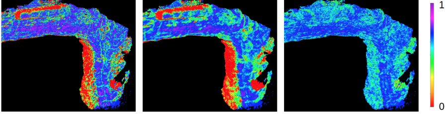
Fig. 2: Grid map output comparison: We show slope ( left ), step height ( middle ), and roughness ( right ) values in geometric traversability computations. All values are converted to the scale from 0 to 1. Slope value tends to have many small areas of peaks, while step height tends to have smoother values across a bigger region. On the other hand, roughness does not have many peak values, and many regions like hills are already captured by the previous two measurements.
