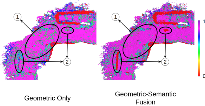
Fig. 7: Grid map comparison between the geometric-only scheme [8] and ours: (1) Our method is less noisy and has more connected regions to plan a feasible trajectory. (2) Our method can detect obstacles that the geometric method could not recognize.
