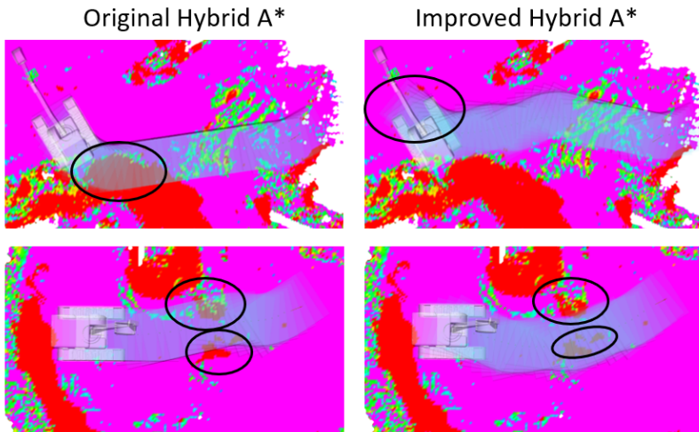
Fig. 4: Comparison between original and improved hybrid A* planners. Our planning method has more flexibility, including running over small obstacles between two tracks based on our traversability map.
