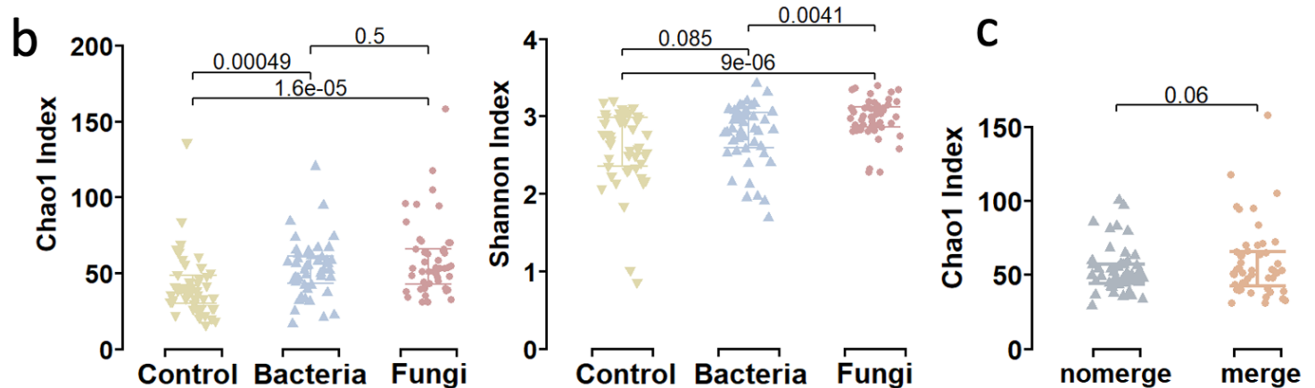
Supplementary Figure 1. Enrichment efficiency in bacteria. a, The genus-level taxa bar plot of the bacterial community compositions in bacterial, control, and fungal partitions. b, Boxplots of the species-level bacterial community alpha diversities (Shannon and Chao1 indices) in fungal, control, and bacterial partitions (n=143) ordered by their mean from smallest to largest (left to right). c, Boxplots of the species-level bacterial community alpha diversity (Chao1 index) before and after merging bacterial reads in the bacterial and fungal partitions (n=48) ordered by their mean from smallest to largest (left to right).
