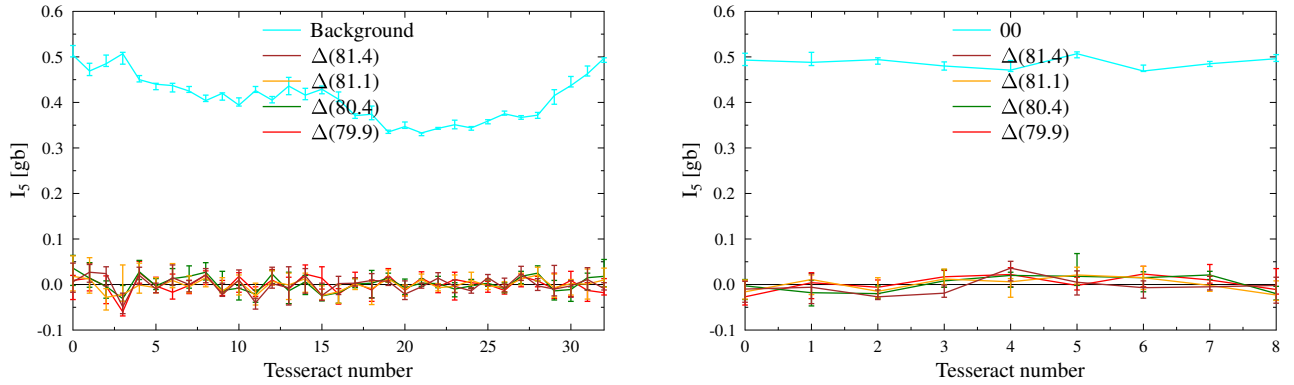
FIG. S3: Another Repeat of the analysis for one of the earlier side branches of the main positive leader.
