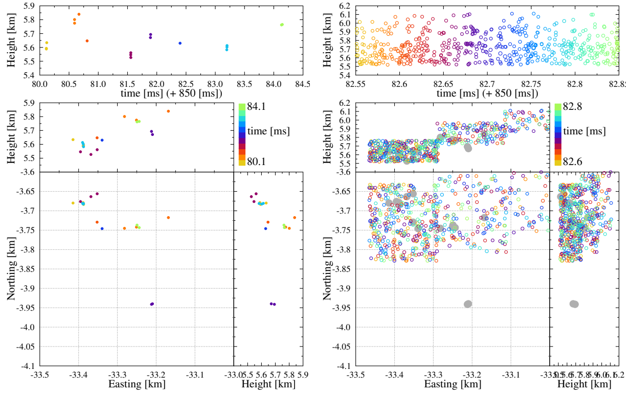
FIG. S4: The sources on the end of the positive leader at times when analysis is performed. Right: the nearest image cubes (# 32, 31, and part of 30) for t=82.7 are overlaid. TRI-D sources with an intensity in excess of 0.36 are shown only.
