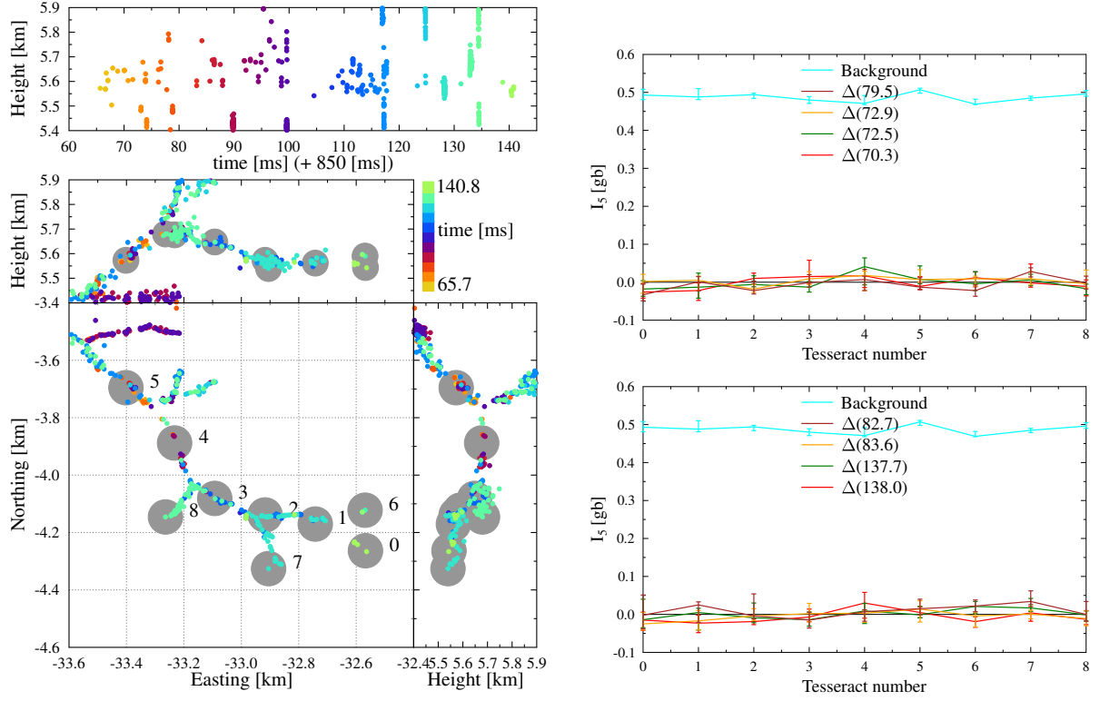
FIG. S2: Repeat of the analysis for one of the earlier side branches of the main positive leader.
