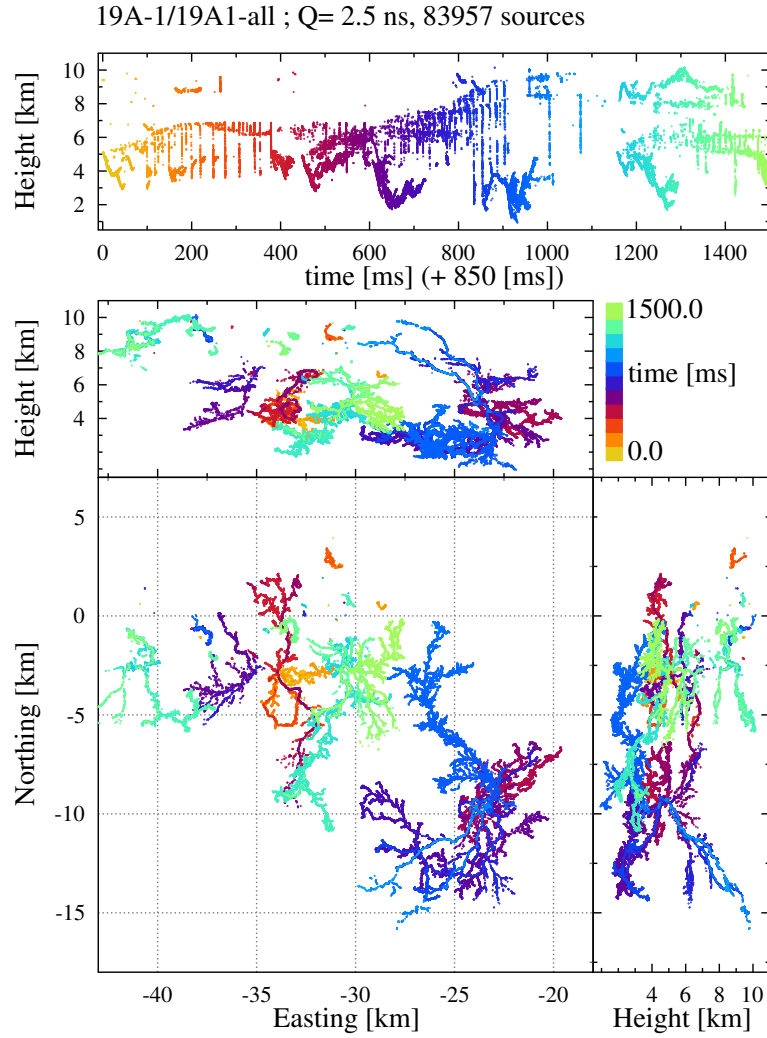
FIG. S1: An overview of the flashes for LOFAR recording 19A-1 that occurred on April 24, 2019 at 19:44:32 UTC. The image is made using the impulsive imager showing over 81,500 sources while requiring that the pulse of each source is detected in at least 157 of a total of 172 antennas and that the timing of these pulses is reproduced with an root-means square not larger than 2.5 ns.
