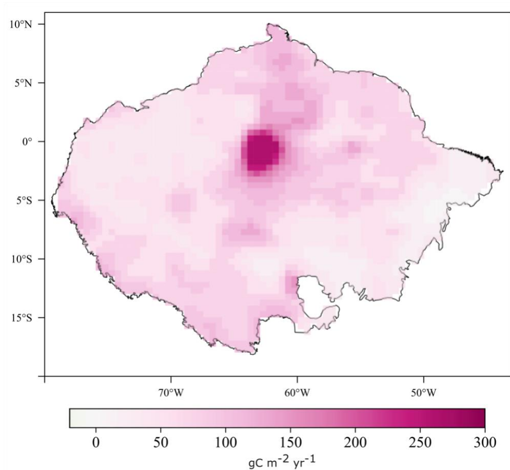
SI Figure 7 Average intact sink uncertainty from TRENDY-v11 DGVMs over the whole biogeographical Amazon ( \text{gC m}^{-2} \text{yr}^{-1} ).
