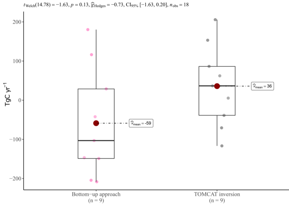
SI Figure 8 Welch's t-test to compare the net land carbon fluxes from bottom-up approach and top-down inversion over 2010-2018 for the Brazilian Amazon.
