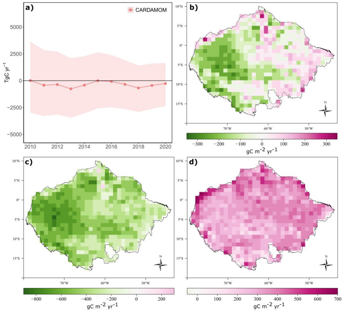
SI Figure 11 Net land carbon fluxes from CARDAMOM. a) Annual net land carbon fluxes for the whole biogeographical Amazonia; b) Spatial average net land carbon fluxes (gC m -2 yr -1 ) of from CARDAMOM between 2010 and 2020; c) Spatial average uncertainty (gC m -2 yr -1 ) of CARDAMOM between 2010 and 2020 (CI 97.5%); d) Spatial average uncertainty (gC m -2 yr -1 ) of CARDAMOM between 2010 and 2020 (CI 2.5%).
