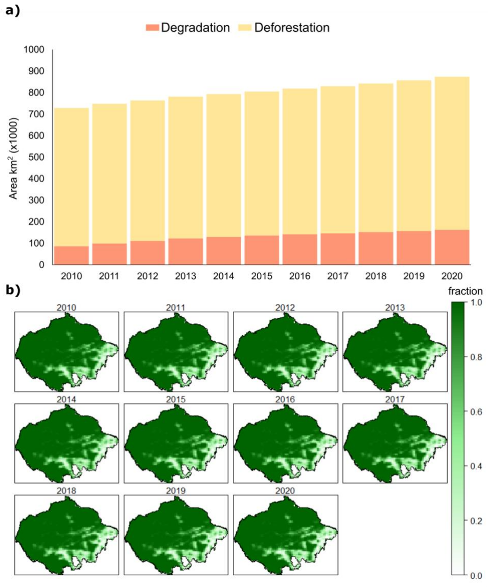
SI Figure 2 Correction of TRENDY-v11 sink estimates using an old-growth areas mask. a) Accumulated deforestation and degradation area in the Brazilian Amazon (km 2 x1000); b) Whole biogeographical Amazon old-growth forest fraction mask based on the annual accumulated disturbance area of deforestation and degradation from INPE.
