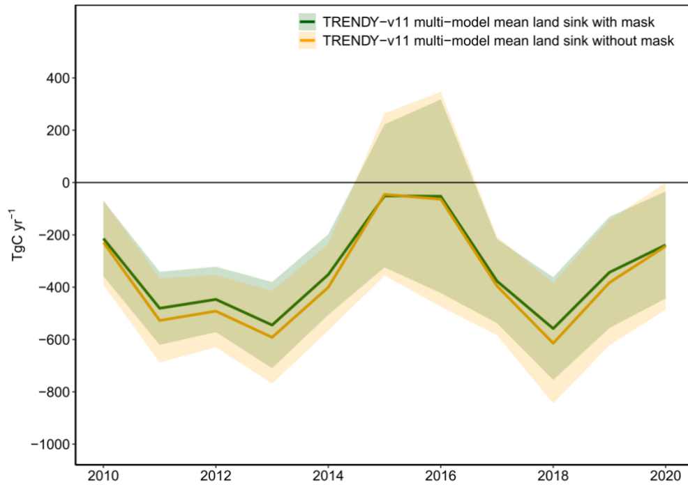
SI Figure 3 Annual intact sink over the whole Biogeographical Amazon simulated by TRENDY-v11 DGVMs with and without the accumulated disturbance mask (SI Figure 2) applied.
