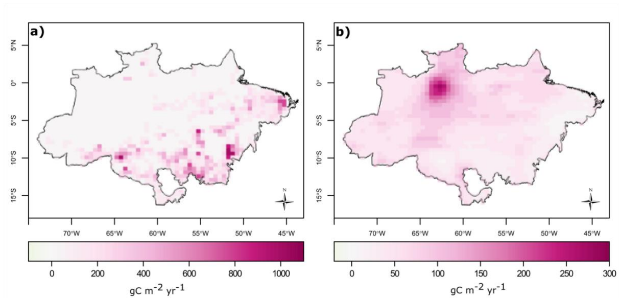
SI Figure 4 Spatial uncertainty of main Figure 1. a) Average spatial uncertainty (2010-2020) of the disturbance fluxes in the Brazilian Amazon; b) Spatial average uncertainty (2010-2020) of the intact sink from TRENDY-v11 DGVMs in the Brazilian Amazon. Data in \text{gC m}^{-2} \text{yr}^{-1} .
