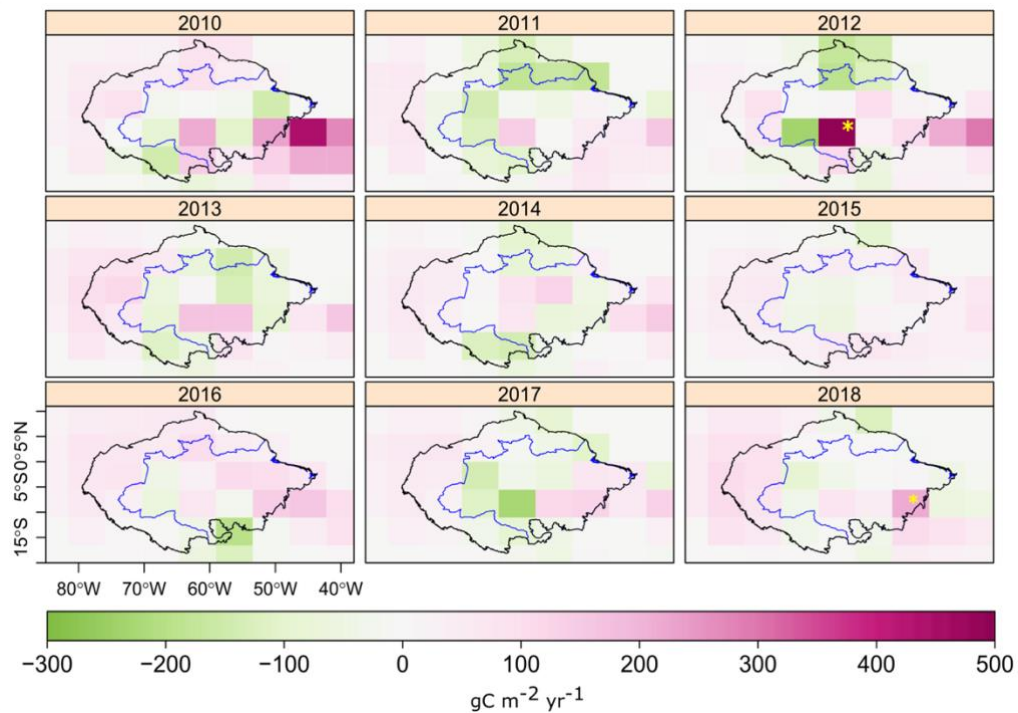
SI Figure 9 Annual spatial net land carbon flux from TOMCAT atmospheric inversion ( \text{gC m}^{-2} \text{yr}^{-1} ). The black line is the biogeographical Amazon limits, and the blue line is
