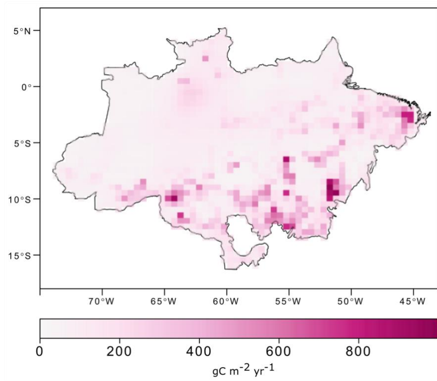
3 4 SI Figure 10 Spatial Brazilian Amazon net land carbon flux uncertainty from the 5 bottom-up approach over 2010-2020 ( \text{gC m}^{-2} \text{yr}^{-1} ). 6
