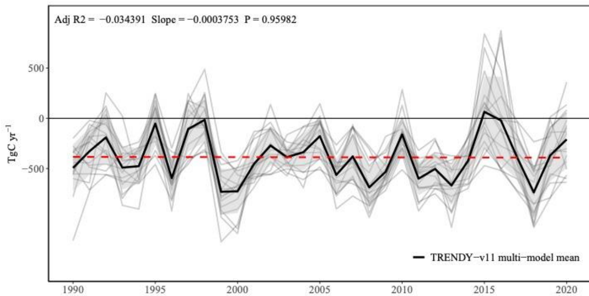
SI Figure 13 Multi-model mean of TRENDY-v11 old-growth forest sink between 1990 and 2020 ( \text{TgC yr}^{-1} ) over the whole biogeographical Amazon. The red dotted line is the linear trend line.
