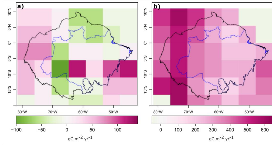
SI Figure 12 Spatial fluxes from the top-down atmospheric inversion. a) TOMCAT atmospheric inversion net land carbon fluxes over 2010-2018 ( \text{gC m}^{-2} \text{yr}^{-1} ); b) average uncertainty estimate over 2010-2018 from TOMCAT atmospheric inversion ( \text{gC m}^{-2} \text{yr}^{-1} ). The blue line is the Brazilian Amazon limits and the black line the biogeographical Amazon limits.
