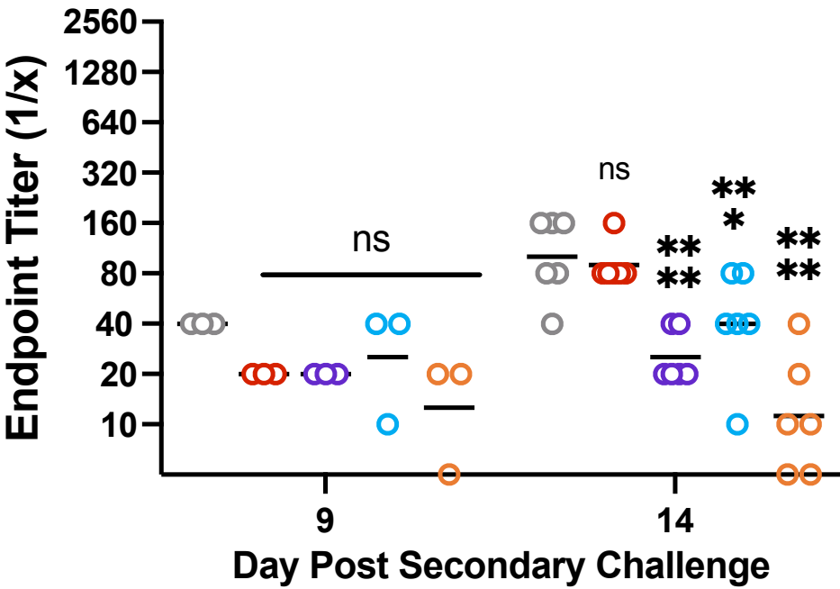
Mock-Wuhan
