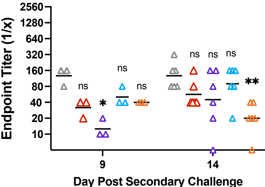
OC43-Wuhan
