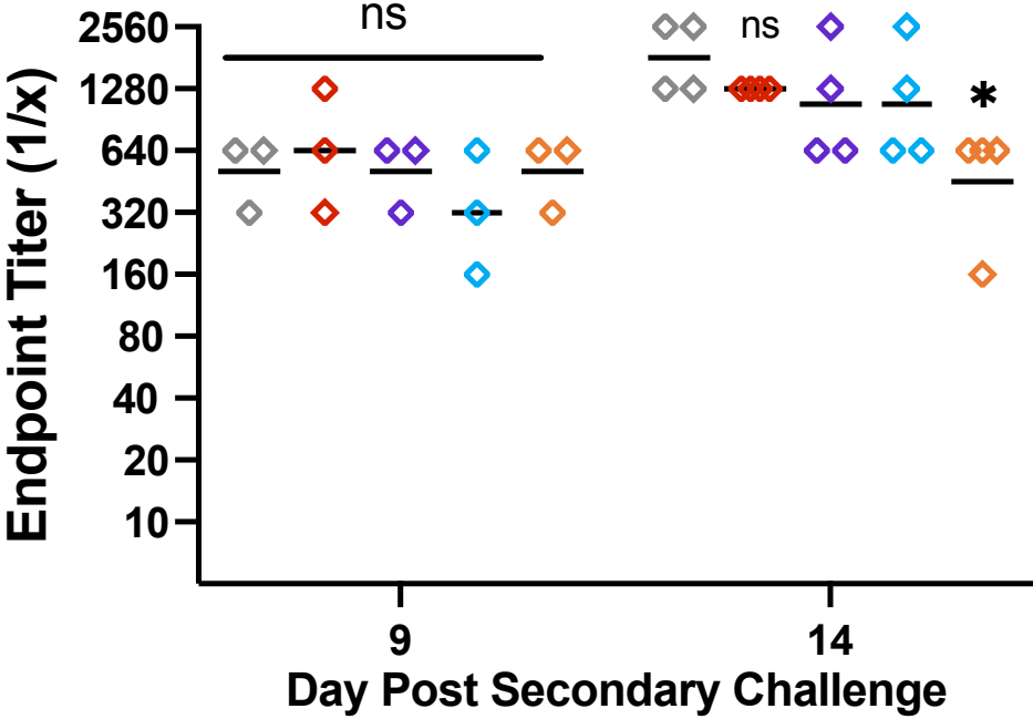
Wuhan-Wuhan
