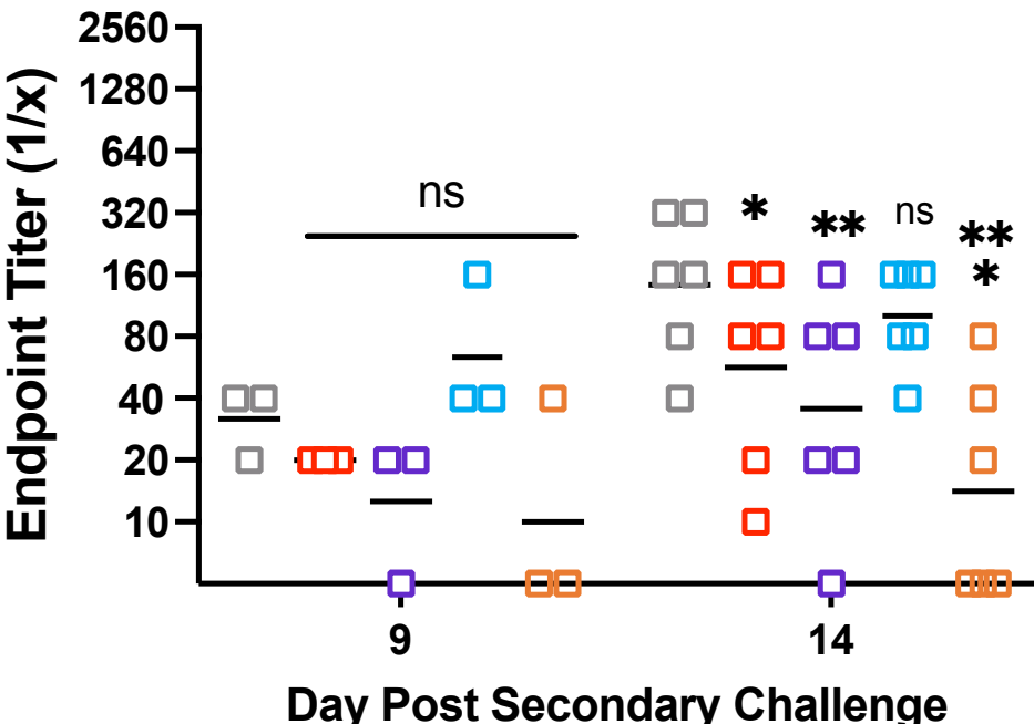
NL63-Wuhan
