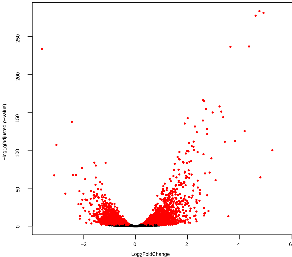
Fig. S2. A volcano plot of differentially expressed genes (DEGs). Y-axis denotes -\log_{10} -P-value while X-axis shows \log_2 FoldChange values. The scattered dots represent each gene, the grey dots indicate genes with no significant differences, and the red dots indicate up-regulated and down-regulated genes with significant differences.
