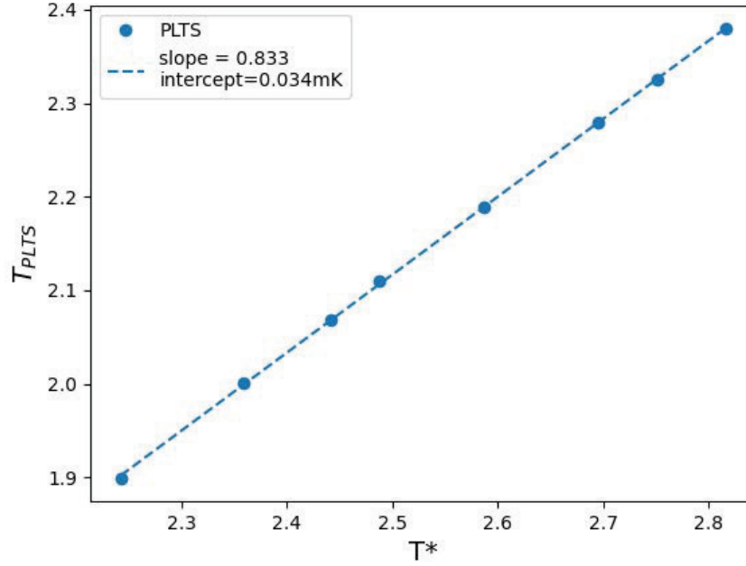
Supplementary Figure 1: Conversion from T^* to T_{PLTS} . Values of T_c^* [1,2] plotted against values of T_c on the PLTS scale 3,4 .
