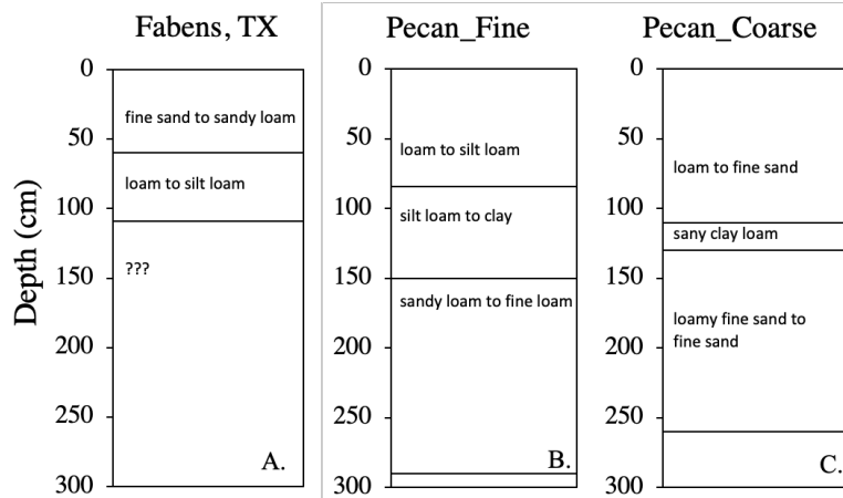
Appendix Figure 1. Soil texture changes with depth at three study sites: natural Fabens (A), Pecan_Fine (B) and Pecan_Coarse (C). Data are from Ortiz and Jin (2021).
