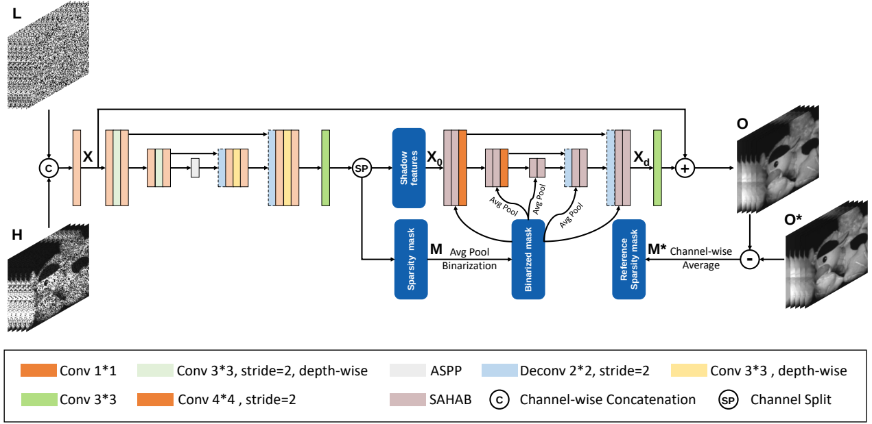
Supplementary Figure 5. The structure of the adopted coarse-to-fine network for multi-spectral reconstruction.
