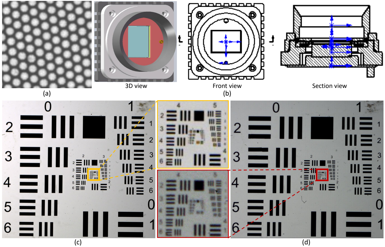
Supplementary Figure 4. The adopted fiber optic plate (FOP) and its performance in tens-megapixel image
