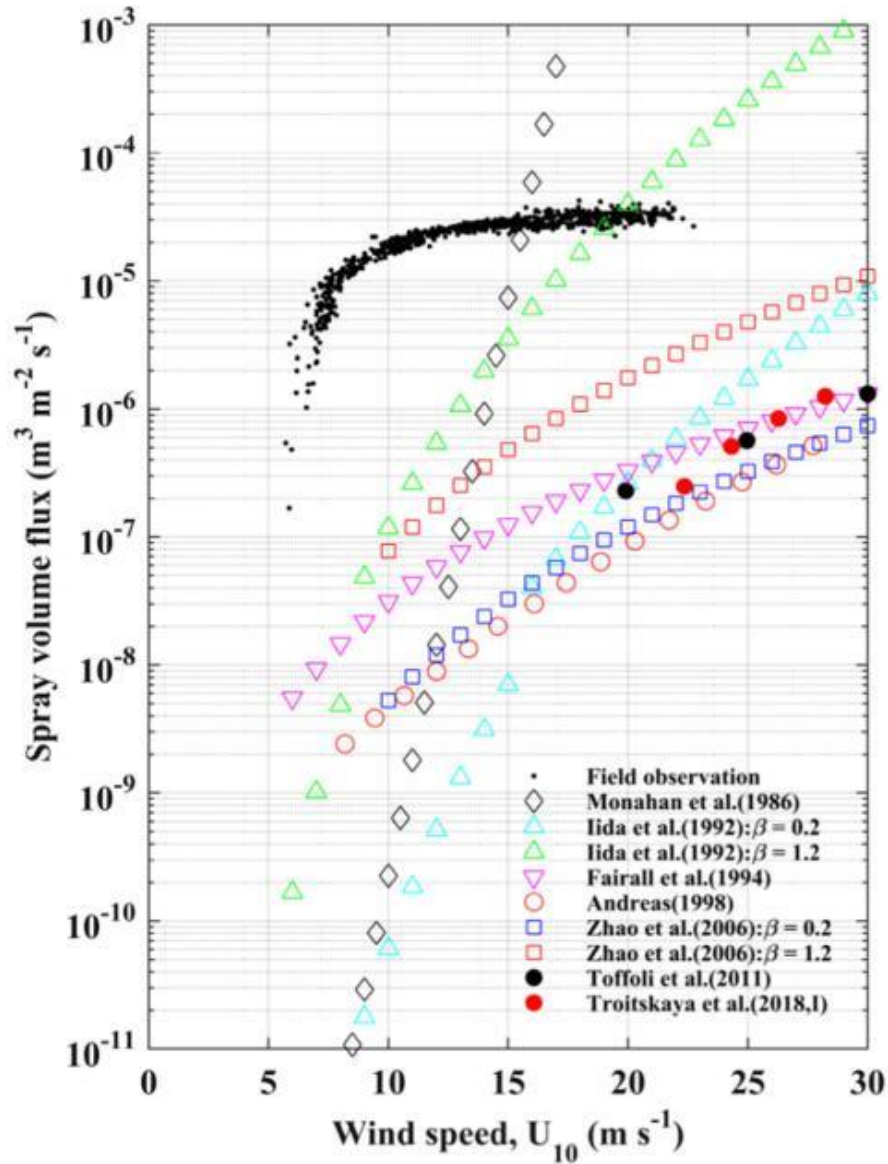
Fig. 7 Comparisons between the sea spray volume flux of the field observations in this article (black dots) and other studies; Monahan
