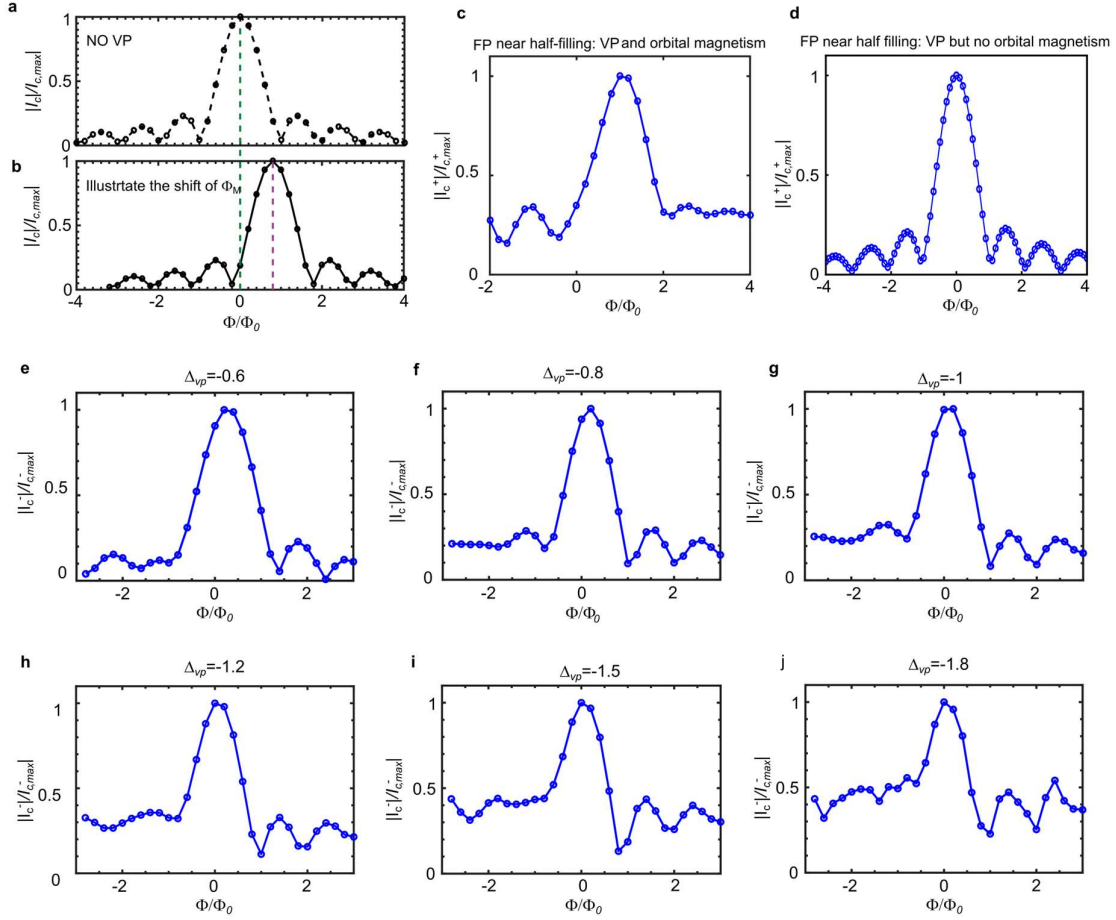
Figure S17: Fraunhofer pattern in the presence of valley polarization and orbital magnetism. a. Standard Fraunhofer pattern when the middle range is a metal, where I_c denotes the critical current. b. Shift of \Phi_M in the Fraunhofer pattern due to the orbital magnetism. c. Typical Fraunhofer pattern near half-filling, which supports an insulating gap. The asymmetry induced by the valley polarization is quite clear. d. Fraunhofer pattern near half-filling “”with no C2T symmetry breaking terms. The asymmetry is not present in this case as there is no orbital magnetization. e-j. Calculated Fraunhofer pattern with various valley polarized strength \Delta_{vp} (in units of meV) near half-filling. To compare with the experiment, we also add a shift of +0.8\Phi_0 for I_c^+ in the Fraunhofer pattern for c .
