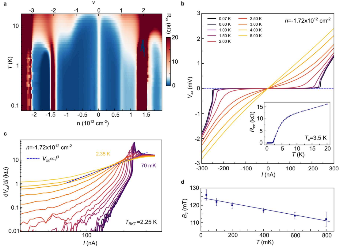
Figure S3. Temperature dependence and characterization of the superconducting state.
