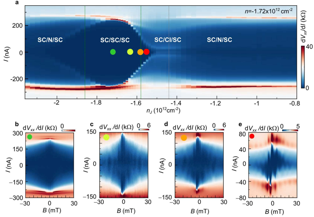
Figure S7. Carrier density dependence of the asymmetry in the Fraunhofer patterns. a. dV_{xx}/dI vs. I and n_J at T = 35 mK, keeping n in the superconducting state. b.-e. Fraunhofer patterns with the weak link being at different doping n_J , corresponding to those labelled by the color circles in a . The Fraunhofer patterns evolve from being symmetric in the SC/SC/SC to being asymmetric in the SC/CI/SC configuration.
