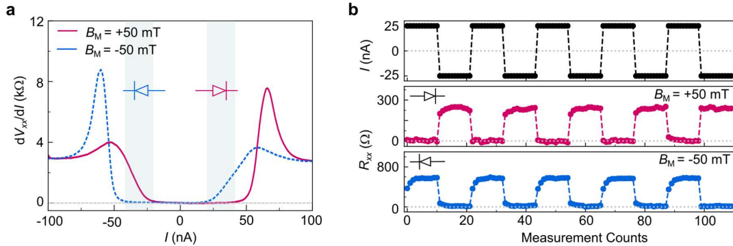
Fig. S11. Zero-field switchable superconducting Josephson diode. a, dV_{xx}/dI vs. I measured setting n_J = -1.56 \times 10^{12} \text{ cm}^{-2} at 35 mK. All curves are taken at B=0 mT after pre-magnetizing the sample at B_M = +50 mT (red) or B_M = -50 mT (blue). The shaded gray regions mark the values of current at which the diode behavior is observed. b, Switching between resistive and superconducting state by changing the direction of I as shown in the top panel. By applying opposite B_M , the diode behavior is inverted (red and blue curves).
