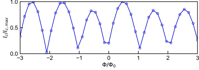
FIG. S18. SQUID Fraunhofer pattern induced by edge states. The parameters are \Delta_{vp} = -0.8 meV, the temperature T = 0.02\Delta_s , and the chemical potential is set within the insulating gap at half-filling.
