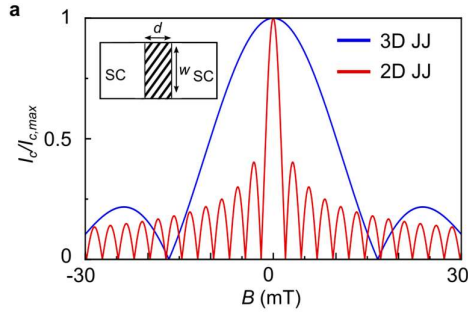
Figure S12. Planar and bulk Josephson Junctions Fraunhofer patterns and 2D SQUIDS.
