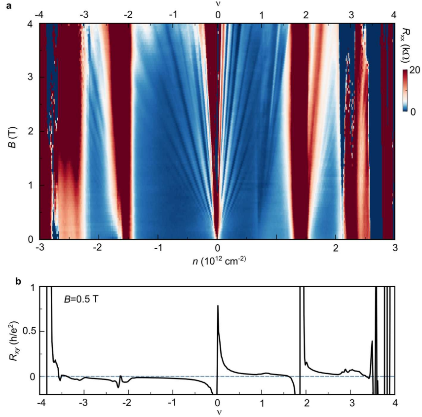
Figure S2. Landau fan diagram and absence of quantized plateau Hall resistance at low field. a. Longitudinal resistance R_{xx} vs. carrier density n and perpendicular magnetic field B , where Landau levels were used to calculate the twist angle of the device. b. Anti-symmetrized transverse resistance R_{xy} vs. n at B = 0.5 \text{ T} , plotted in units of h/e^2 , where h is Planck's constant and e is the electron charge. No quantized plateau Hall resistance close to \nu = -2 is observed. All data in the figure is taken setting V_{TG} = 0 \text{ V} .
