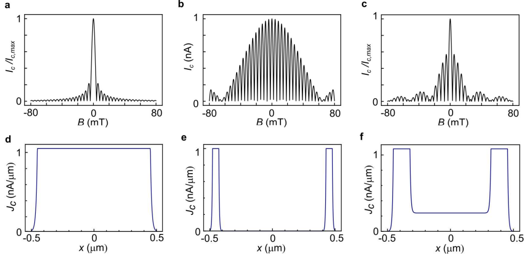
Fig S13. Fraunhofer patterns corresponding to different current density distributions. a-c. Fraunhofer patterns corresponding to the current density distributions shown in d-f .
