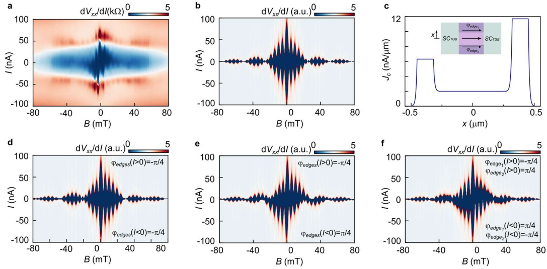
Fig. S14. Asymmetric Fraunhofer patterns corresponding to different symmetry broken current densities. a. Fraunhofer pattern to higher fields at the SC/CI'/SC position. b. Modelled Fraunhofer pattern based on the current density profile of c . c. Current density profile to calculate the Fraunhofer patterns including both bulk and edge contribution. Both edges and the bulk can include a different phase. d. Calculated Fraunhofer pattern having a different phase between edge and bulk but with the same phase between edges. e. Same as d. , but the phase of the edges changes when inverting the current direction. f. The phases of the two edges are opposite and they change sign upon changing the current direction.
