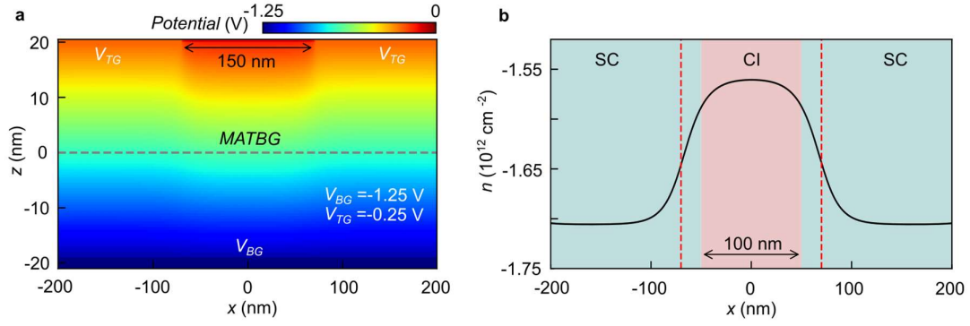
Figure S5. Simulations of the electrostatic potentials governing our devices. a. Calculated potentials as a function of position x and height z , for a junction configuration with V_{BG} = -1.25 V and V_{TG} = -0.25 V. The back gate and top gates are placed at z = -20 nm and z = 20 nm, respectively. The etched region is marked by the double arrow at the top of the figure. The dashed gray line shows the position at which the MATBG would be located. b. Extracted line-cut of the electrostatic potential from a at z = 0 nm, the MATBG position. Vertical red dashed lines show the position where the top graphite was etched. The light green and red regions show the extension of the SC and CI states. The effective length of the JJ in this case is 100 nm, as marked in the figure.
