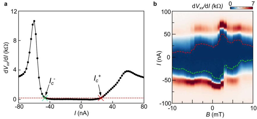
Figure S8. I_c extraction from the dV_{xx}/dI vs. I data. The plotted data corresponds to the same Fraunhofer pattern as in Fig. 1e (right) of the main text. a dV_{xx}/dI vs. I linecut of b at zero field. The red dashed line marks a threshold value defining the end of the superconducting state. b. dV_{xx}/dI vs. I and B . The extracted I_c^+ and I_c^- are sketched as dashed red and green lines.
