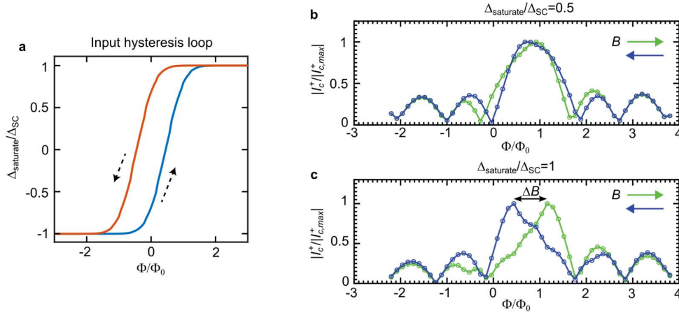
Figure S19. Hysteresis in Fraunhofer pattern from spin magnetism. a. Hysteresis loop inputted in the calculation, where \Delta_{saturate} denotes the saturated spin polarization. b. Fraunhofer pattern with \Delta_{saturate}/\Delta_{sc} = 0.5 . c. Fraunhofer pattern with \Delta_{saturate}/\Delta_{sc} = 1 . \Delta B signal the size of the hysteresis due to the spin polarization, as explained in the main text.
