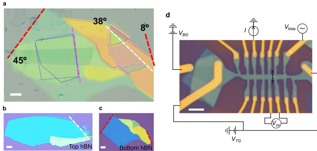
Figure S1. Optical image of the device and alignment to hBN. a. Resulting final stack, where the red and white dotted lines show misalignment between the edges of top and bottom hBN and those of the two graphene flakes composing the MATBG in blue. b. – c. Optical micrographs of top and bottom hBN used for stacking the van-der-Waals heterostructure shown in a . The white and red dotted lines mark the crystallographic edges of the two hBN flakes. d. Optical picture of the final device, with a schematic of our 4-probe measurement setup. The black dotted line marks the position of the narrow-etched region of the top-graphite gate, corresponding to the location of the weak link in the junction. Scale bars equal 5 \mu\text{m} in all figures.
