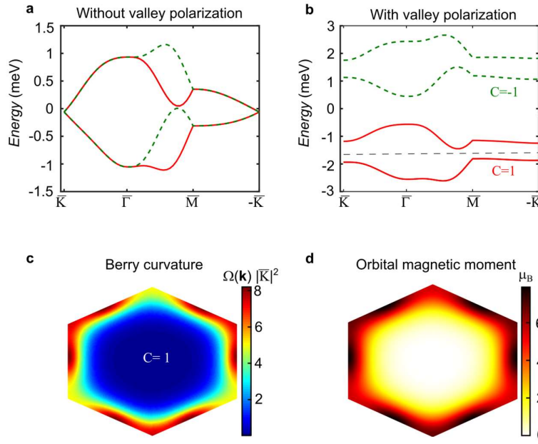
Figure S16: a-b Band structures of MATBG with and without valley polarization. The solid red bands are from one valley, while the dashed green bands are from the opposite valley. In b the Haldane term is added to lift the degeneracies at \pm\bar{K} and a dashed black line is used to indicate the half-filling position, where there is an insulating gap. c Distribution of Berry curvature of the lowest bands in b in the Brillouin zone, which clearly shows a Chern number C = 1 . d Orbital magnetic moment in k -space in units of Bohr magneton \mu_B of the lowest band in b .
