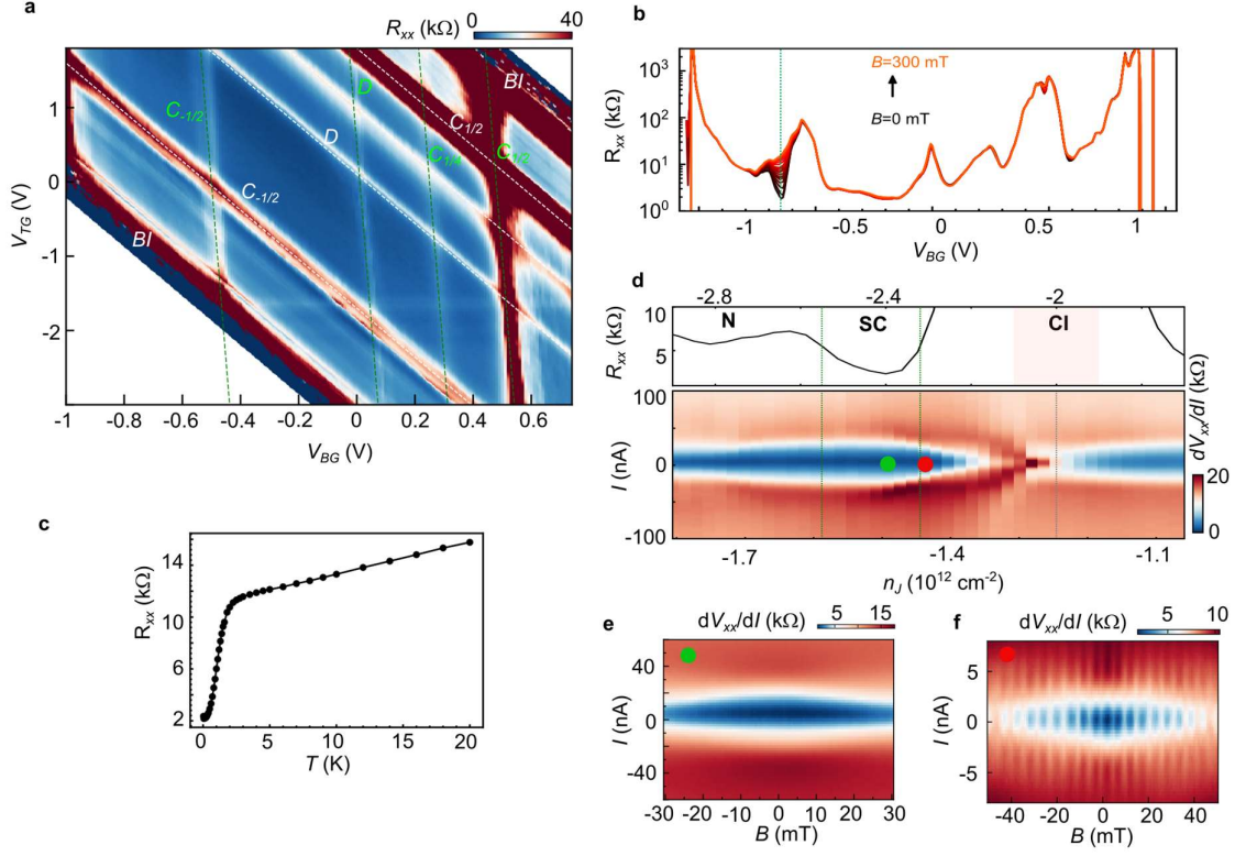
Figure S6. Device B transport characterization. a. R_{xx} vs. V_{BG} vs. V_{TG} at 35 mK. Very similar features to device A are visible and highlighted with the same nomenclature as in Fig. S4. The red cross marks the position where the Fraunhofer pattern shown in d. is measured, corresponding to the SC/CI'/SC position, similar to the main pattern of the other sample discussed in the main text. b. R_{xx} vs. v vs. B at low fields. c. R vs. T characteristics of the SC at the center of the dome as marked by the green dashed of b. d. (Top) Magnification of b around the SC state -3 < v < -1.8 . (Bottom) dV_{xx}/dI vs. I at different n_J , keeping n = -1.44 \times 10^{12} \text{ cm}^{-2} in the SC state. Dashed green vertical lines mark the position where n_J is no longer in the SC state. e. Fraunhofer pattern of the SC/SC/SC position in this device. f. Fraunhofer pattern of the SC/CI'/SC position in this device.
