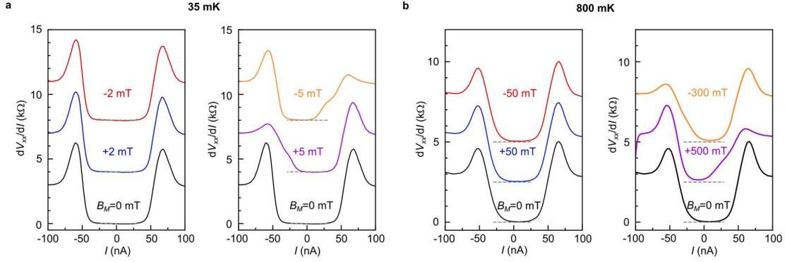
Fig. S10. Distinguishing between high and low field hysteresis. dV_{xx}/dI measured right after cooling down (black curves) or after applying different B_M at 35 mK a. and 800 mK b. While at 35 mK, fields above 3 mT are enough to switch the magnetic state, at 800 mK, fields above 300 mT are needed, proving we have two distinct effects. The behavior of the dV_{xx}/dI is also different for the two effects, i.e. for the low field effect I_c^+ > |I_c^-| , when B_M > 0 , whereas the opposite is true for the high field effect. This is clear comparing the orange and purple curves at the two temperatures.
