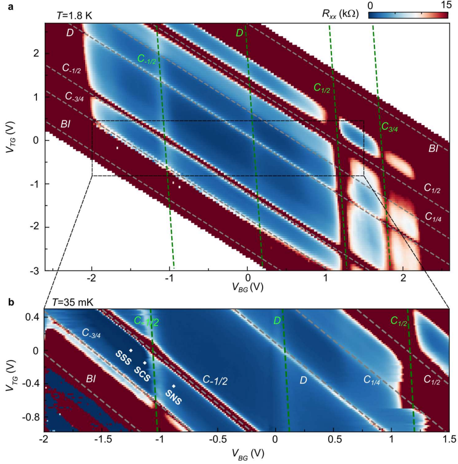
Figure S4. Dual-gated maps. a. R_{xx} vs. V_{BG} and V_{TG} at T = 1.8 K. The diagonal features marked with grey dashed lines are the integer fillings of the main regions ( n in Fig. 1b of main text), gated by both the back gate and top gates. Slightly tilted vertical features, fitted with green dotted lines, are the integer fillings of the junction region ( n_J in Fig. 1b of main text), mainly gated by the back gate. Labels of the integer filling factors marked by dashed lines correspond to: band insulator ( BI ) at full filling, correlated insulator at plus/minus three-quarter filling ( C_{\pm 3/4} ), plus/minus half filling ( C_{\pm 1/2} ) and one quarter filling ( C_{1/4} ) and Dirac point ( D ). b. Zoom-in of black-delimited area in A taken at base temperature T = 35 mK, where the superconducting state is fully developed. White squares mark the diagonal line in the map at which both main regions are kept in the superconducting state, and the junction region is set at different doping.
