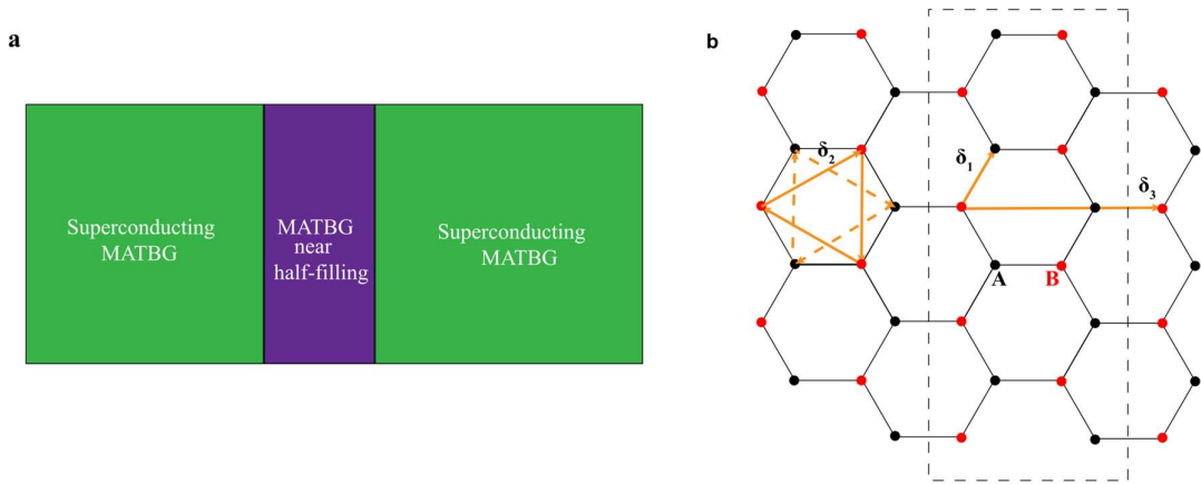
Figure S15. Sample and lattice geometry considered in the theoretical calculation for this MATBG based-Josephson junction. a. A schematic plot of the studied twisted bilayer
