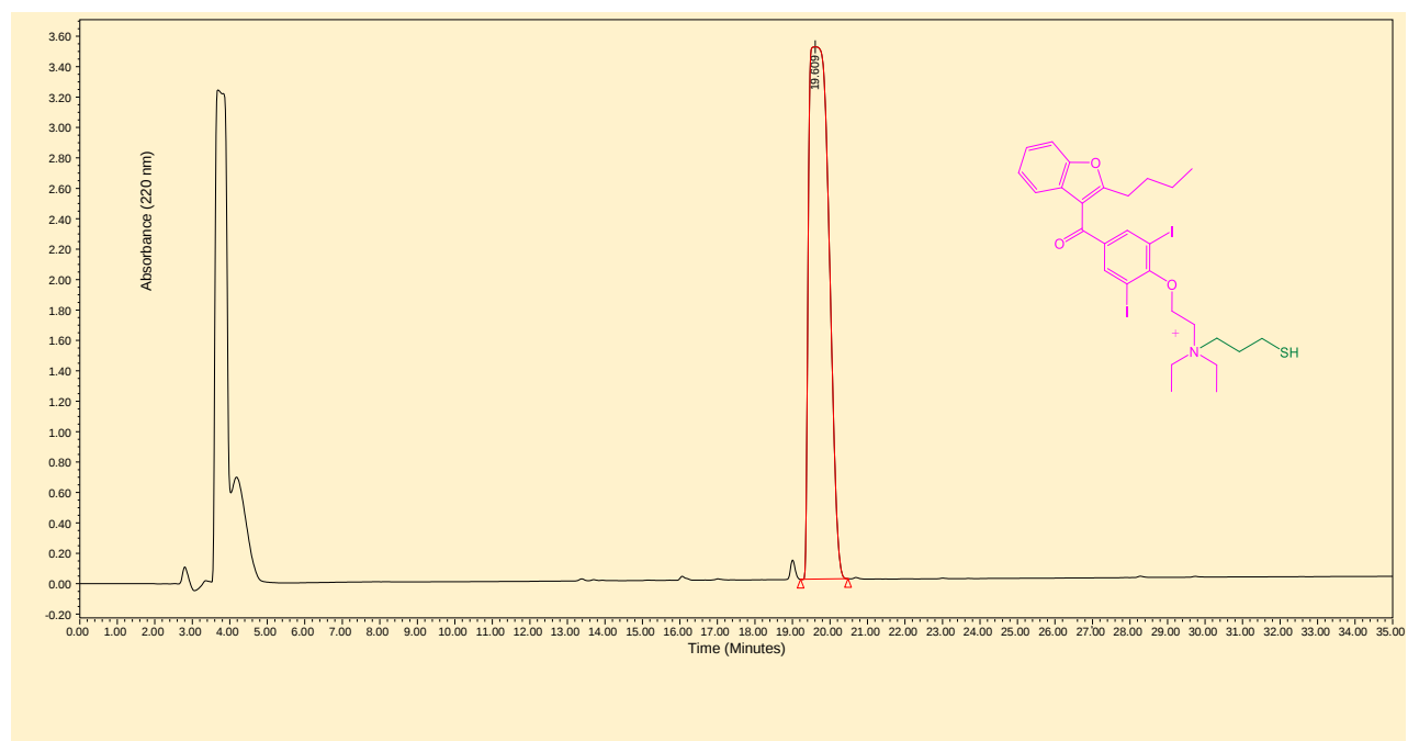
Figure-S5: HPLC Chromatogram of Amiodarone-thiol
