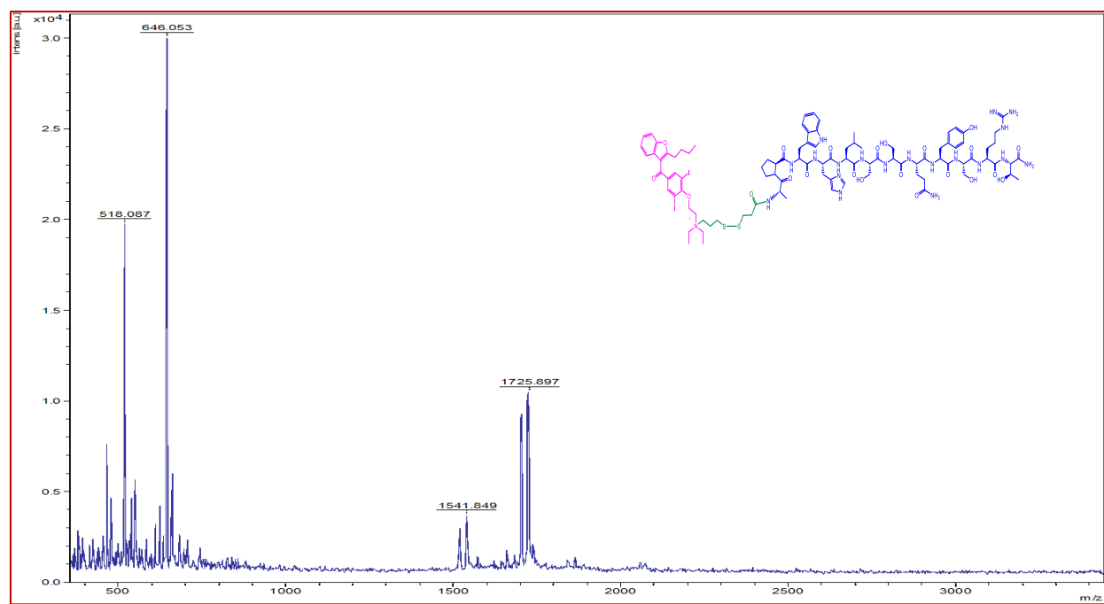
Figure S8: Amiodarone-SS-CTP-MALDI
