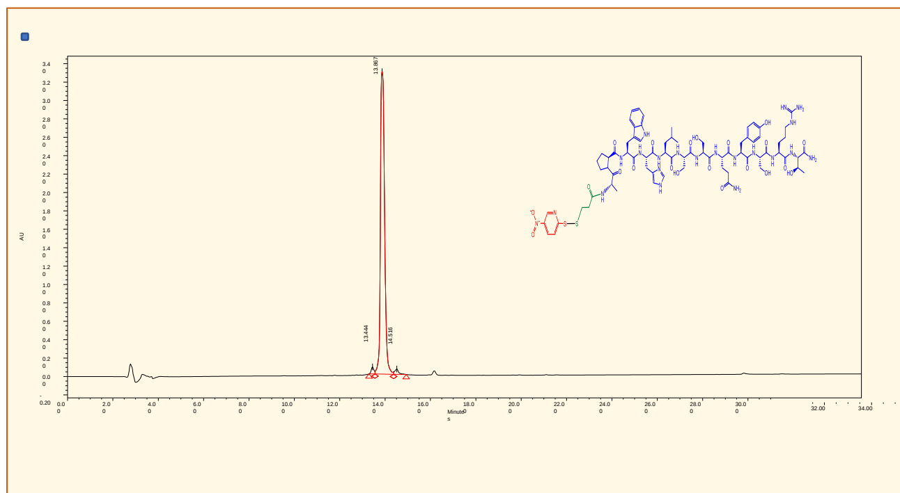
Figure-S3: HPLC Chromatogram of NPys-S-CTP
