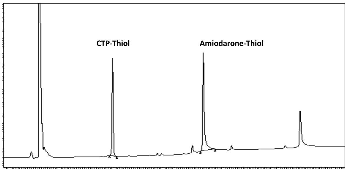
Figure S9-d: Amiodarone-CTP cleavage products from DTT reduction
