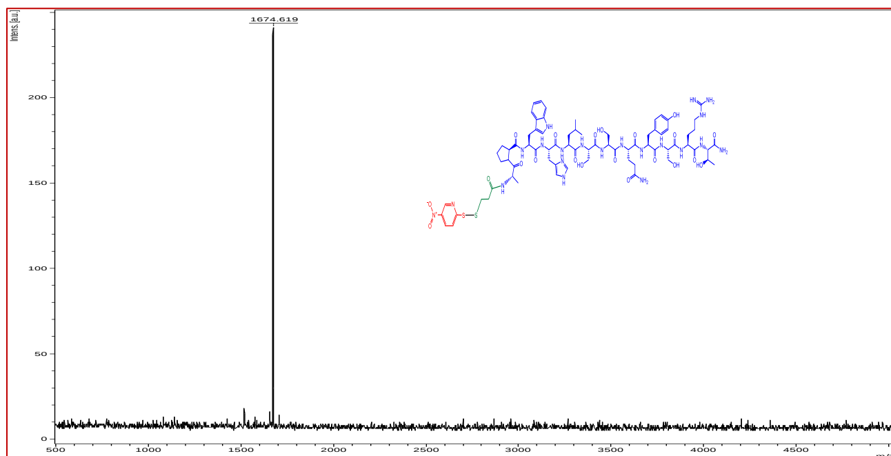
Figure-S4: MALDI analysis of NPys-S-CTP
