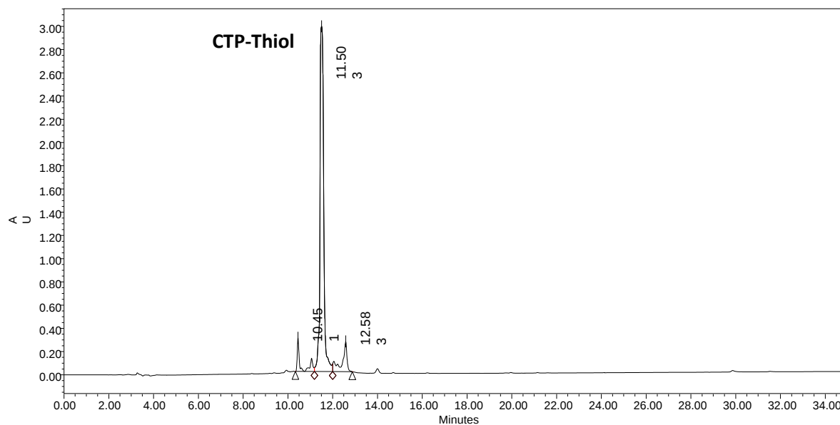
Figure S9-b: SH-CTP pure
