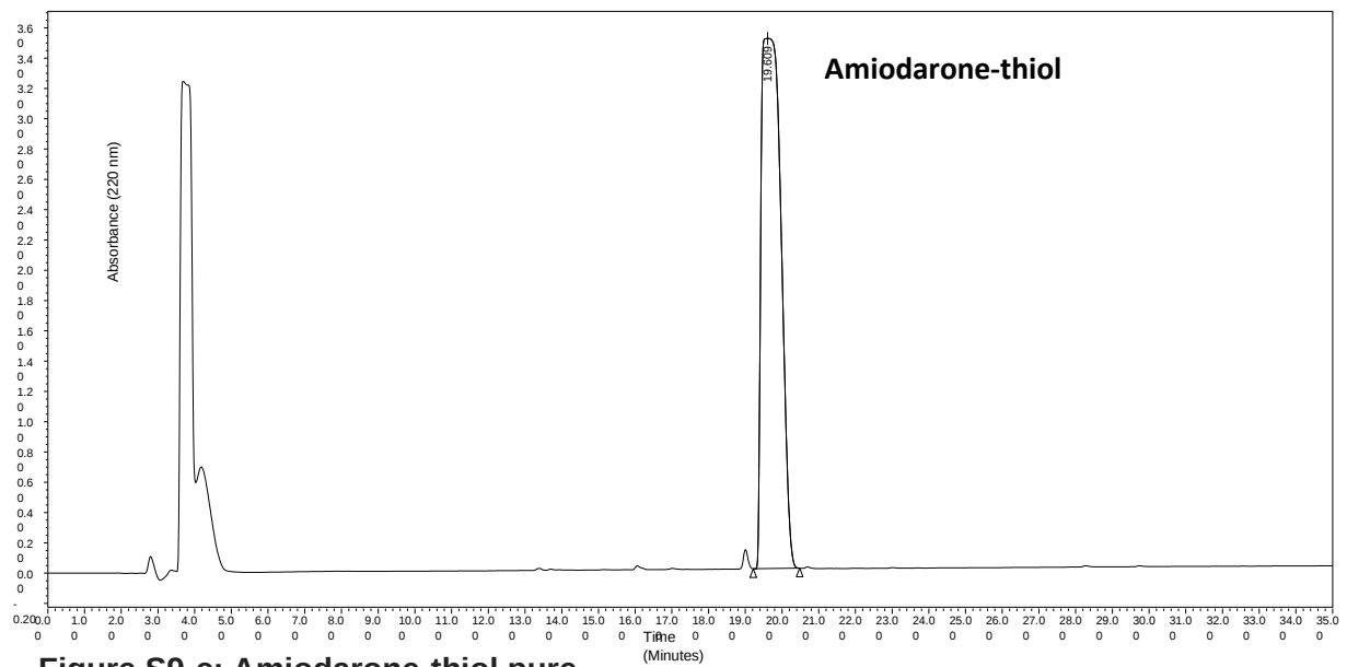
Figure S9-c: Amiodarone-thiol pure
