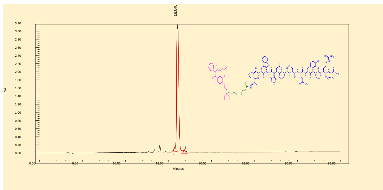
Figure S7: Amiodarone-SS-CTP-amide HPLC Trace
