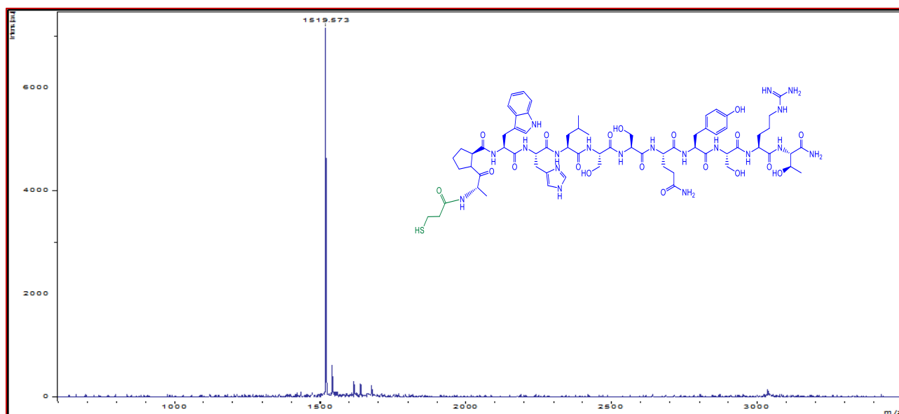
Figure-S2: MALDI analysis of CTP-thiol
