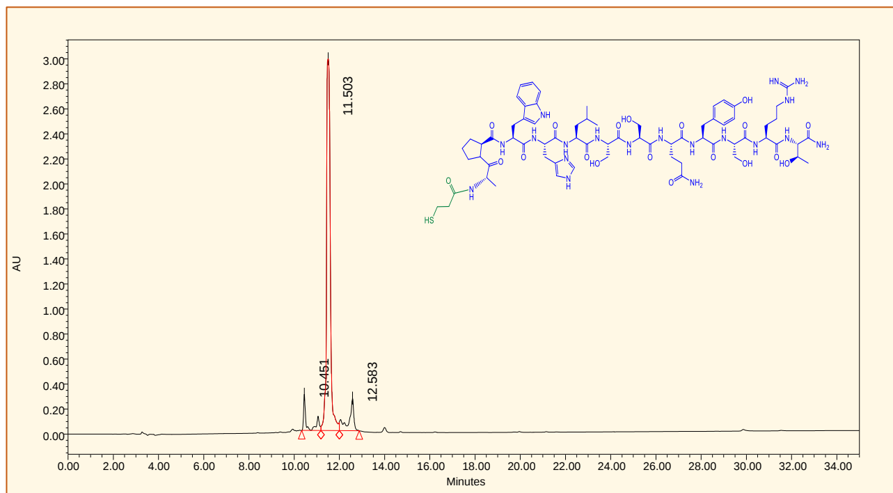
Figure-S1: HPLC Chromatogram of CTP-thiol
