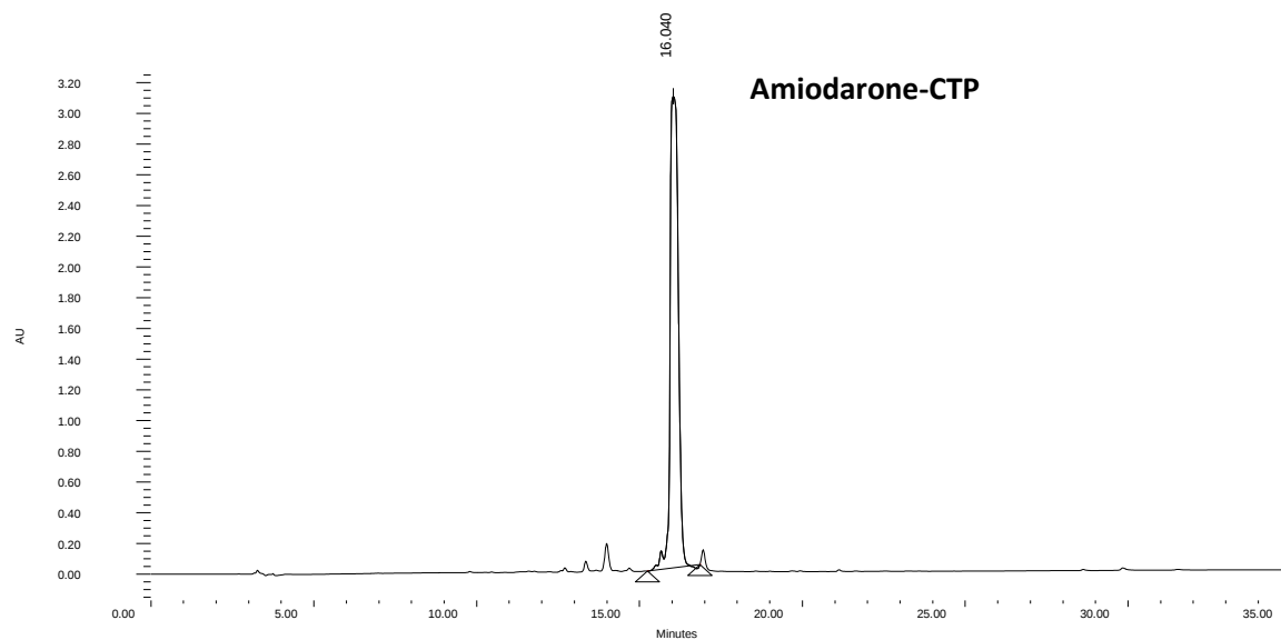
Figure S9-a: Amiodarone-CTP pure
