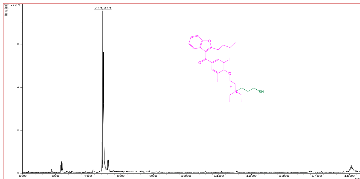
Figure-S6: MALDI analysis of Amiodarone thiol
