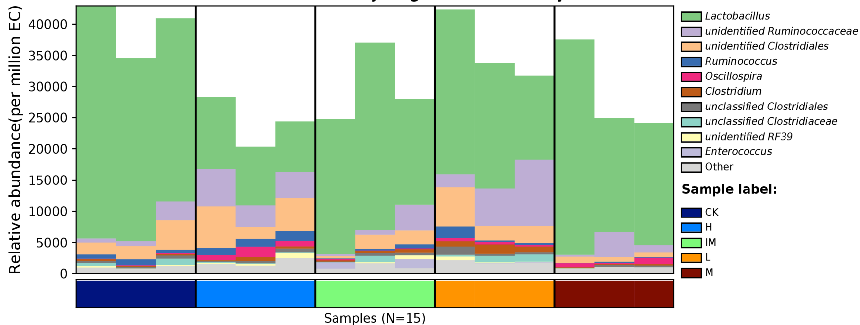
UDPNAGSYN-PWY: UDP-N-acetyl-D-glucosamine biosynthesis I
