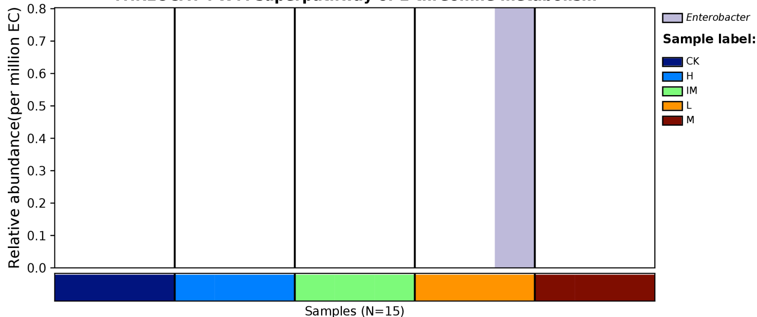
UDPNAGSYN-PWY: UDP-N-acetyl-D-glucosamine biosynthesis I
