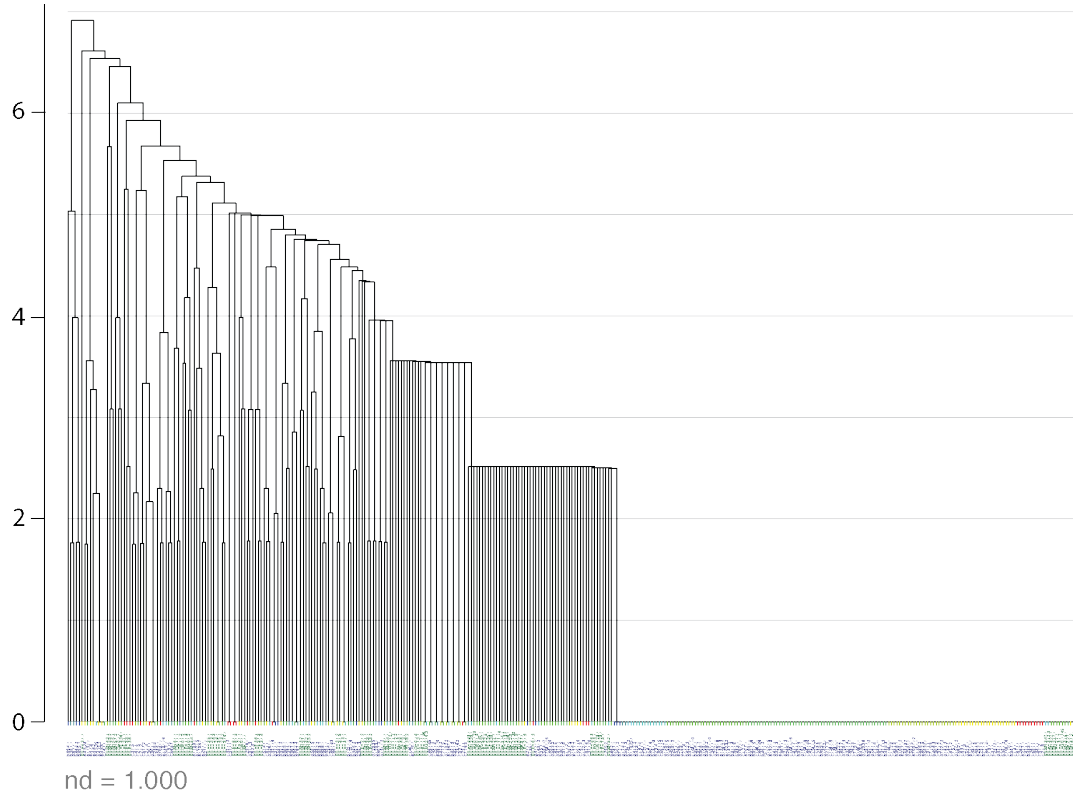
Fig. S4. Hierarchical organization of the fully-grown (extant) EF network ( nd=1.000 ). NG_{age} scaled modularity matrix 50 of the last distinguished EF network in the timeline was input to calculate Euclidean distance matrix 82 which was hierarchically clustered with the Ward's minimum variance method 83 . Vertical axis represents dissimilarity between clusters of the dendrogram. Horizontal axis labels are color-coded to distinctively identify the rearrangements of the two classes of constructs, loops (green) and domains (blue). The nodes are age-sorted ascendingly within clusters, color-coded by node age and labelled using standard SCOP nomenclature 28 . The most ancient loop motifs and domain structures of the clusters comprising 95% percentile connectivity of the two major waves of functional innovation and the hidden EF switch of power law and modularity exchange are displayed on the tips of clades.
