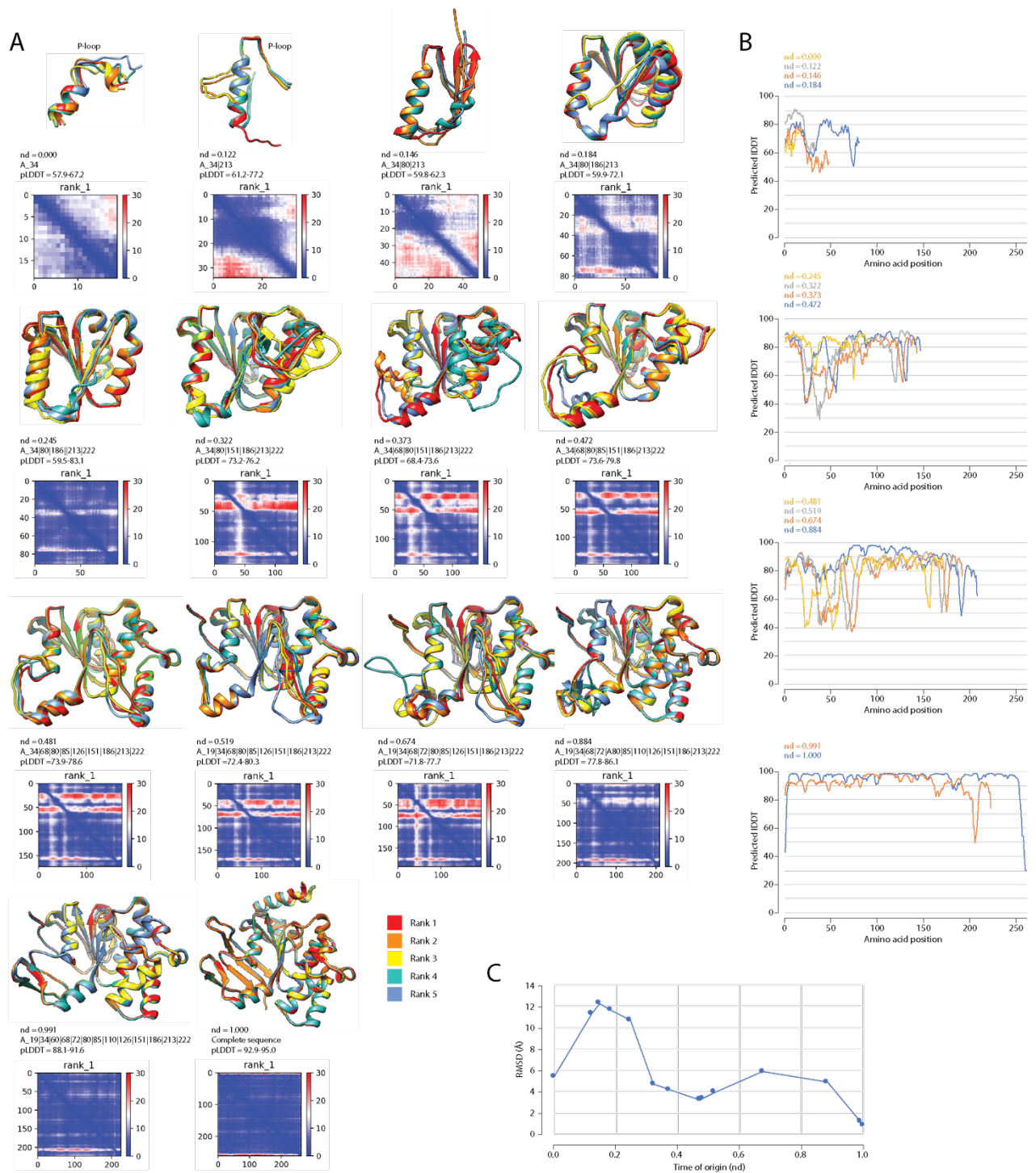
Fig. S8. Confidence parameters of AlphaFold2 structural predictions of a P-loop transporter. (A) Structural alignments of the 5 ranked predicted structures, pLDDT confidence levels, and predicted aligned error (PAE) plots that measure confidence in the relative position of residue pairs. (B) Predicted IDDT statistics at residue level for rank 1 predicted structures. (C) Pairwise structural alignments of predicted structures to the extant crystallographic entry (PDB 1B0U) show variation of RMSD values along the timeline.
