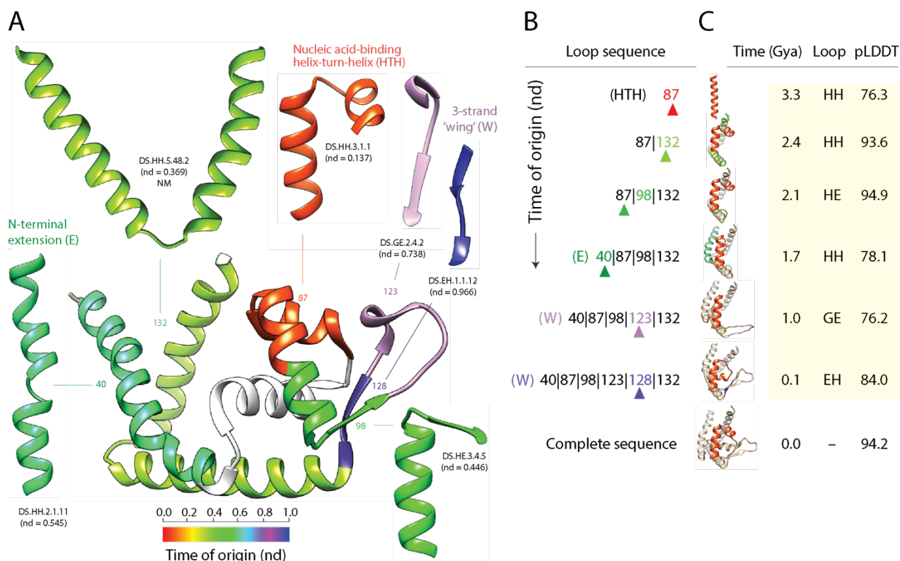
Fig. S11. Tracing the evolutionary history of loop prototypes embedded in the structure of a variant of the primordial winged-helix domain. (A) A crystallographic model describing the atomic structure of the helix-turn-helix (HTH) containing nucleic acid-binding domain of a MarR complex of Staphylococcus aureus (PDB entry 4EM2) shows the nucleic acid-binding helix-turn-helix (HTH)-containing bundle packed against the 3-stranded \beta -sheet with 'wings' (W) and linked to an N-terminal extension. The different loop prototypes that make up the winged-helix domain structure are colored according to their time of origin, which is given as relative age (nd) in a scale from 0 (origin of proteins) to 1 (the present). (B) A time-ordered series of growing molecules was constructed by stitching loops together according to their time of origin. The sequence of loops is given from N- to C-terminus, with loops labeled in numbers and stitching interfaces indicated by pipe symbols. The last loop to be added to the sequence is indicated with an arrowhead and colored according to its age in each model. (C) Atomic structures of the growing molecules were modeled directly from their sequences with AlphaFold2. The age of the first loop (the HTH motif) and the last loop to be added to the structure are colored in the growing structures. The time of origin (Gya), makeup of bracing secondary structures of the loop, and pLDDT confidence level of the ab initio prediction are given for each growing molecule.
