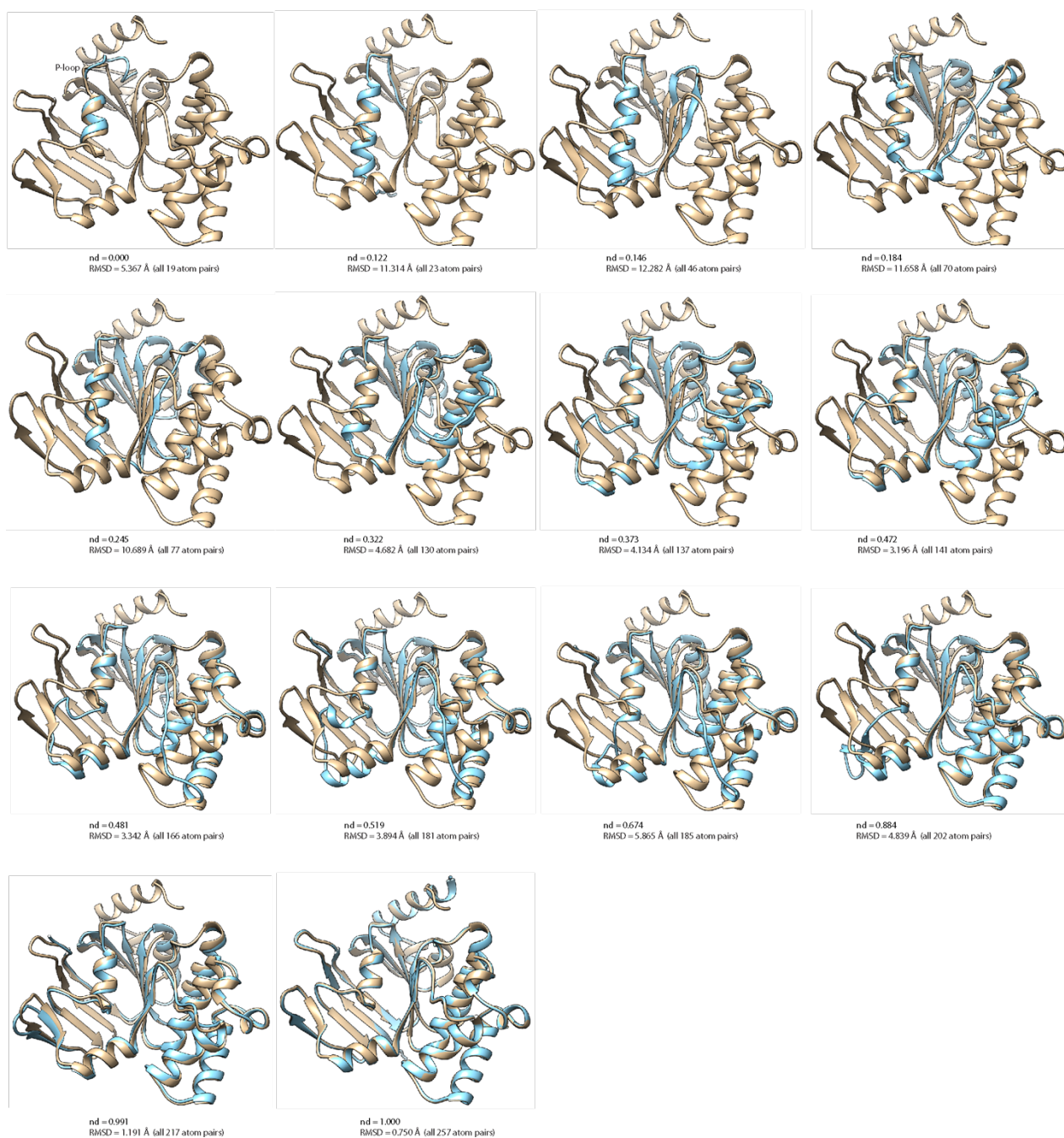
Fig. S9. Structural alignment of modelled structures to the crystallographic entry of the P-loop transporter (PDB 1B0U).
