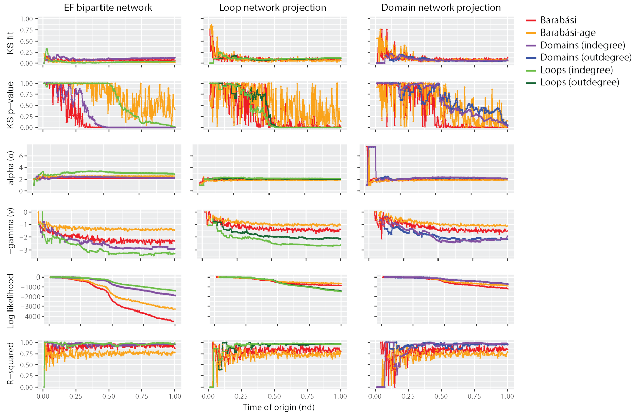
Fig. S2. Statistical descriptors of power law behavior for the EF bipartite network and its loop and domain network projections. Six differential indicators of preferential attachment were plotted for each network. Two reference curves, Barabási (red) and Barabási-Age (orange), were included for comparison. Barabási specifies the probability of preference of an old node as P_i \sim k_i^\alpha while Barabási-Age confers heavier power law properties to older (with smaller nd ) nodes using P_i \sim (k_i^\alpha)(l_i^\beta) . Here, k_i is the indegree of node i in the current event; \alpha is the preferential attachment exponent, with default value one, i.e. linear preferential attachment; l_i is the age of node i , i.e. the number of events elapsed since the node was added, with maximum number measured by the ‘aging.bin’ parameter; \beta is the exponent of aging, kept at 1 for linear increases in probability of preference of an older node (with high l_i ). Separate curves were computed for the ‘alldegree’ of loop and domain portions of the EF network and for ‘outdegree’ and ‘indegree’ of projected loop and domain networks. Degrees were cumulative and weighted. The six power law indices include: (i) the KS fit statistic that scores deviation of input degree data vector from the fitted power law distribution; smaller scores denote better fit; (ii) the KS p-value less than \alpha=0.05 indicate rejection of the null hypothesis of degree data being drawn from the fitted power-law distribution 46,47 ; (iii) the exponent of the fitted power-law distribution ( \alpha ); (iv) the slope of power-law linear regression model ( -\gamma ); (v) the log-likelihood of the fitted parameters (likelihood); and the (vi) coefficient of determination ( R^2 ) indicating confidence in the linear model through percentage of degree data explained by the regression line. Higher \alpha , lower -\gamma and closer to zero likelihood correspond to power law behavior. Statistics were calculated for each event of the growing networks. Time of origin ( nd ) is indicated on a relative 0-to-1 scale.
