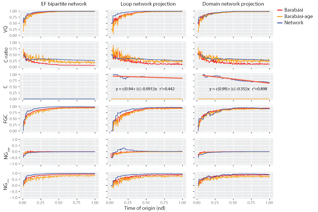
Fig. S3. Modularity indices of the EF bipartite network and its loop and domain network projections. Six indicators of modularity were plotted for each network. The coefficients of linear regression lines (grey) over C for the loop network were -0.000033 by network size ( N ) and -0.091 by age, and those for the domain network were -0.000190 by N and -0.350 by age. Determination coefficients ( R^2 ) were 0.372, 0.442, 0.960 and 0.898, in that order. The linear models shown are by nd . Two modeled control sets, Barabási (red) and Barabási-Age (orange) were included as reference. The “Age” control enriches preferential attachment properties in older (smaller nd ) nodes, inducing slightly different modularity curves. Single comprehensive modularity curves were computed for each network. Modularity calculations required cumulative and weighted connectivity input. Age ( nd ) is indicated on a relative 0-to-1 scale.
