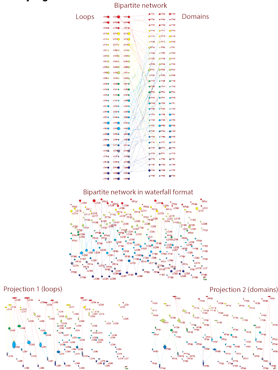
Fig. S1. Various network forms, features and layouts illustrated through a model miniature network. The diagrams illustrate an undirected bipartite miniature network in bipartite (A) and waterfall (B) layouts and its two network projections in waterfall layouts (C,D). The original form has 90 nodes per bimodal partition and 30 nodes per age, resulting in a reduction in number of corresponding node groups by one-third if shrunk by age. Loop nodes are designated as ‘loop classifiers’ (LC). Domain nodes are designated ‘fold families’ (FF). They are described with symbols, with size proportional to the number of links they establish. The connectivity in the undirected bimodal network was generated at random, strictly between the two partitions. The connectivity in the projections was generated based on the sharing instances within partitions and describes construction of directed ‘discrete event’ networks in waterfall format. As time progresses from top to bottom in a waterfall layout, events pan out as the progressive appearance of nodes and links, clustered from left to right. Network growth was made explicit by coloring of nodes according to age (red-to-blue) and that of links by node of origin, by using time-induced arrows or arcs (edges in case of undirected) with density
