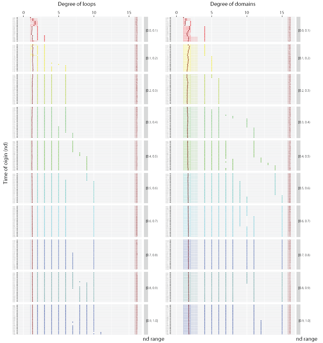
Fig. S7. Measure of central tendency and dispersion in loop and domain components of the EF network. The accumulation (and dispersion) of node degrees of the bipartite network components with age ( nd value) was captured through Tukey boxplots with boxes (first and third quartiles bracketing the median), whiskers (values within \pm 1.5 \times inner quartile range), and outliers. Each boxplot describes the span of cumulative connectivity along events of the evolutionary timeline by providing visualization of chronological accumulation of undirected connections with time. Average values of connectivity of loops and domains were mapped using red diamonds and reported with two digits of significance. Each one of the aggregate 228 events along the timeline are labeled with their relative age in a 0-to-1 scale. The timeline of events was also coarse-grained into 10 age bins (colored red-to-blue).
