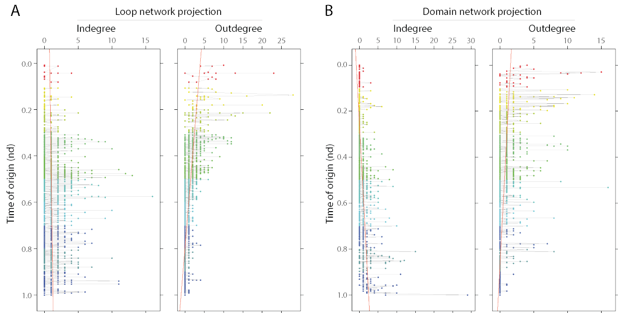
Fig. S6. Connectivity of events along the timeline in the loop (A) and domain (B) network projections of the EF network. Data points describe indegree and outdegree of nodes of different ages of networks analyzed at present time ( nd = 1 ). Symbols were color-coded according to node age. Linear regression lines (tomato-red) show rigorous trend of co-option of loops throughout the timeline and gradual growth of recruitment (embedding of loops) with age in emergent domains until recent times to cater for modern loop functionome (indegrees of panel A and B).
