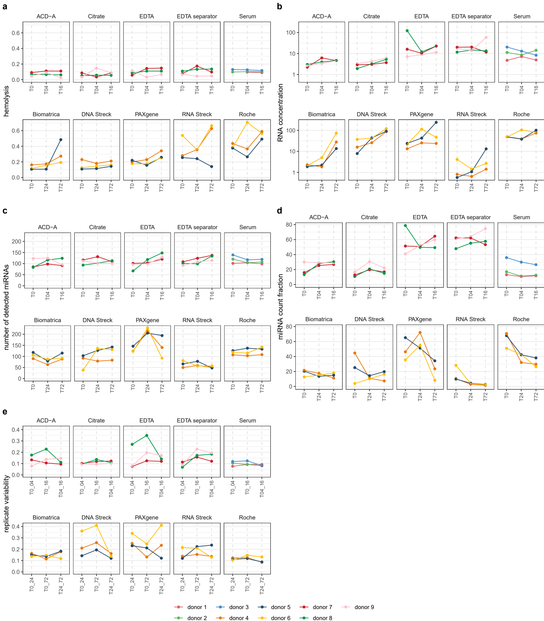
Supplementary Fig. S7: Performance metrics of blood collection tubes over time at miRNA level. Evolution of hemolysis in plasma (a), measured by absorbance at 414 nm with Nanodrop. Evolution of RNA concentration (b) calculated based on the number of endogenous counts vs RC spike-in RNA counts. Evolution of the number of miRNAs (c). Evolution of the fraction of counts mapping to miRNAs vs all counts (d). Evolution of the pairwise area left of the curve (replicate variability (e) performance metrics). T0=plasma prepared immediately after blood draw. T04, T16, T24, T72=plasma prepared 4, 16, 24 and 72 hours after blood draw, respectively. Note that different donors were sampled and that tubes were processed at different time intervals for preservation and classic tubes.
