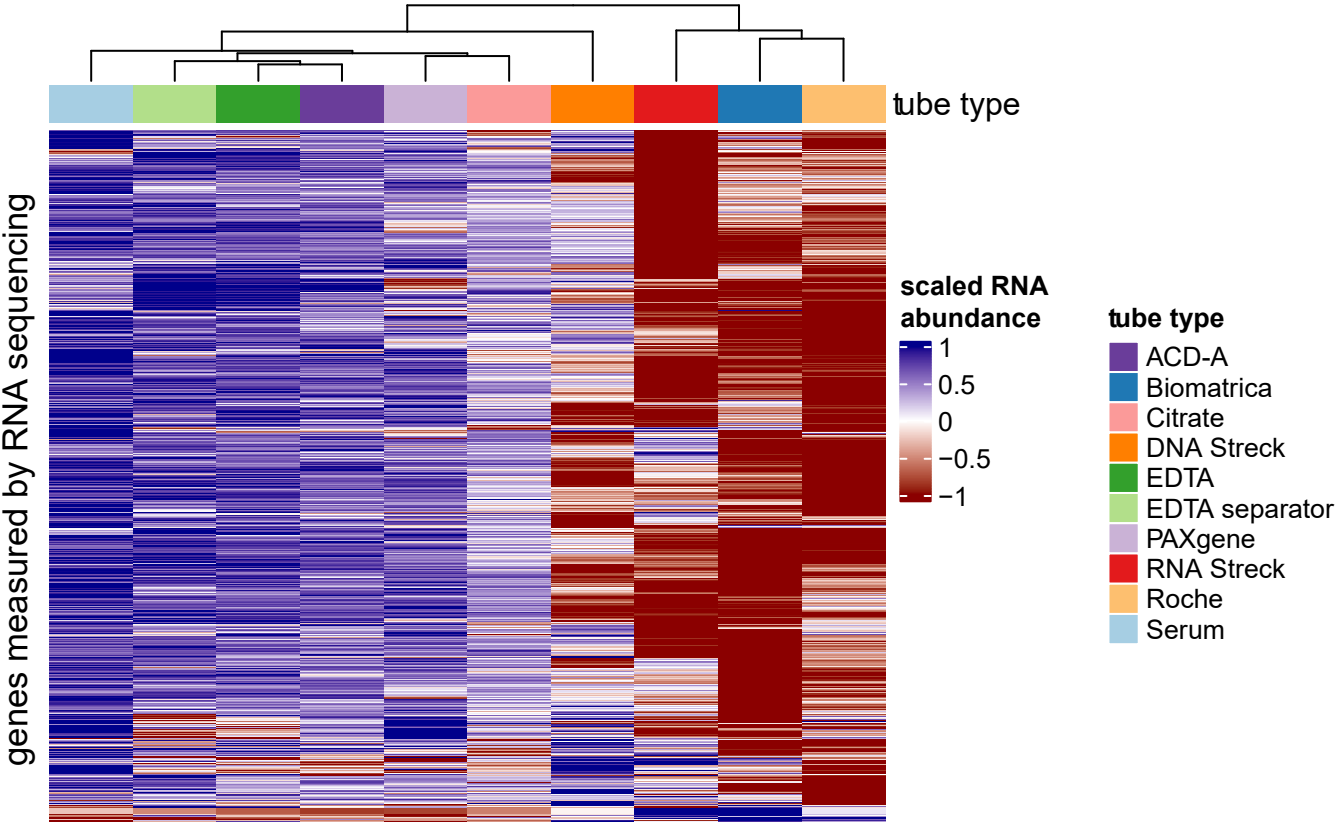
Supplementary Fig. S12: RNA abundance levels differ across blood collection tubes. Using normalized and scaled count data, gene abundance levels (i.e., mean abundance of the tube replicates) are shown for each tube type at time interval T0. The normalised counts are scaled between -1 (low abundance) and 1 (high abundance) per gene to make abundance differences across genes comparable. Only genes with \geq 10 counts in all three replicates of one tube type were included. T0=plasma prepared immediately after blood draw. Note that different donors were sampled for preservation and classic tubes.
