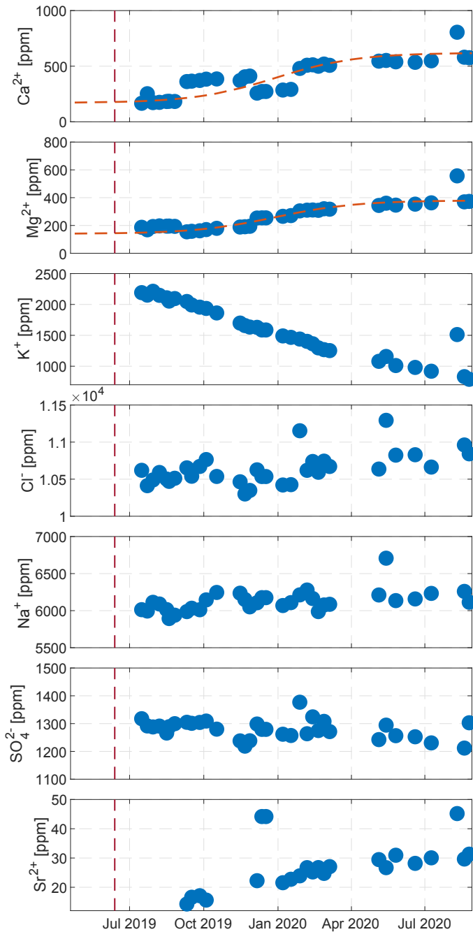
Fig. 2 Ion concentrations. Concentrations during the course of the experiment of [a] Ca, [b] Mg, [c] K, [d] Cl, [e] Na, [f] SO 4 , [g] Sr. For Ca and Mg idealized lines are drawn in red. For Cl, Na and SO 4 the third last data point lies outside of the depicted range.
