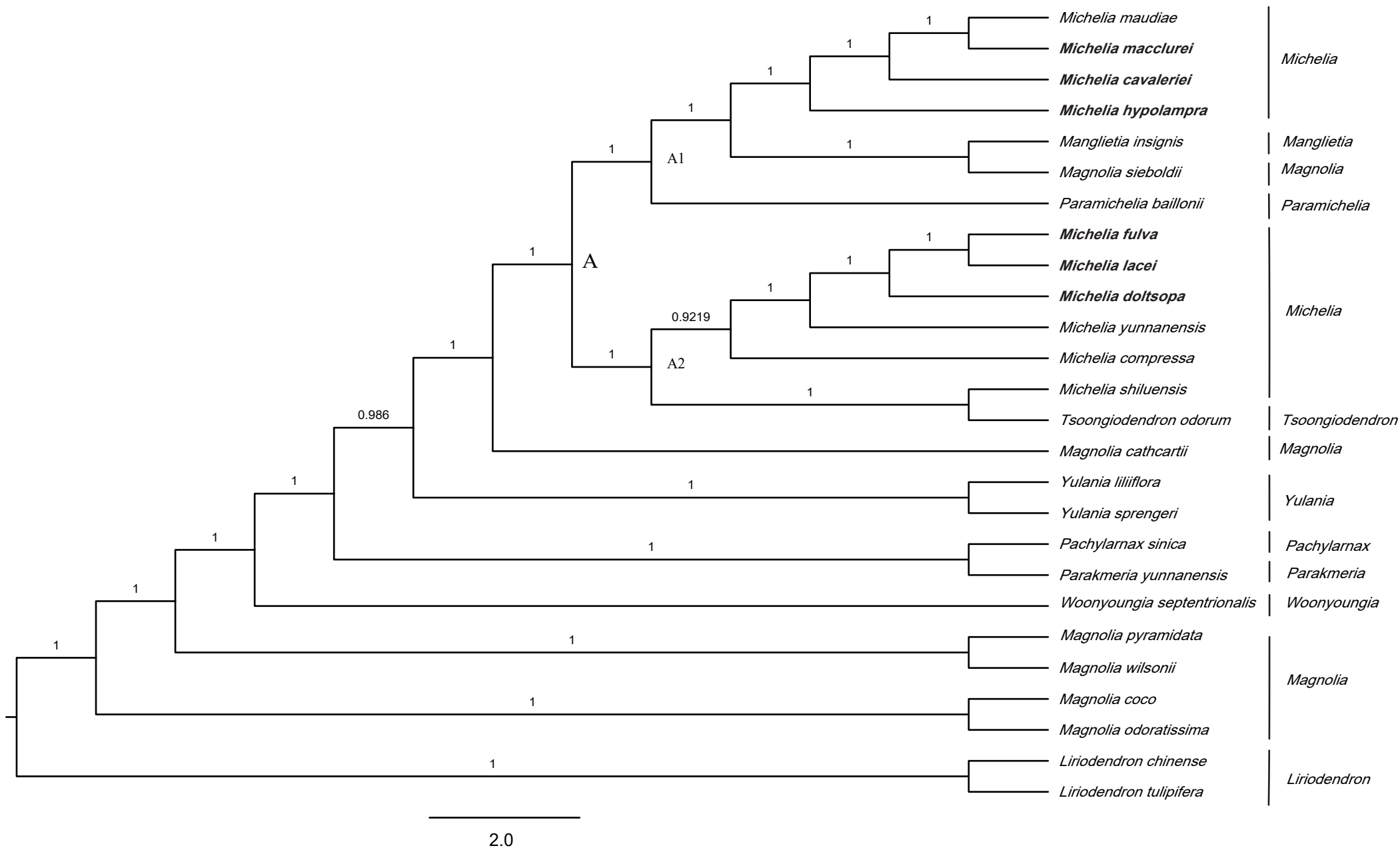
Figure S1. Phylogenetic relationships by Maximum Likelihood of 26 Magnoliaceae species.
