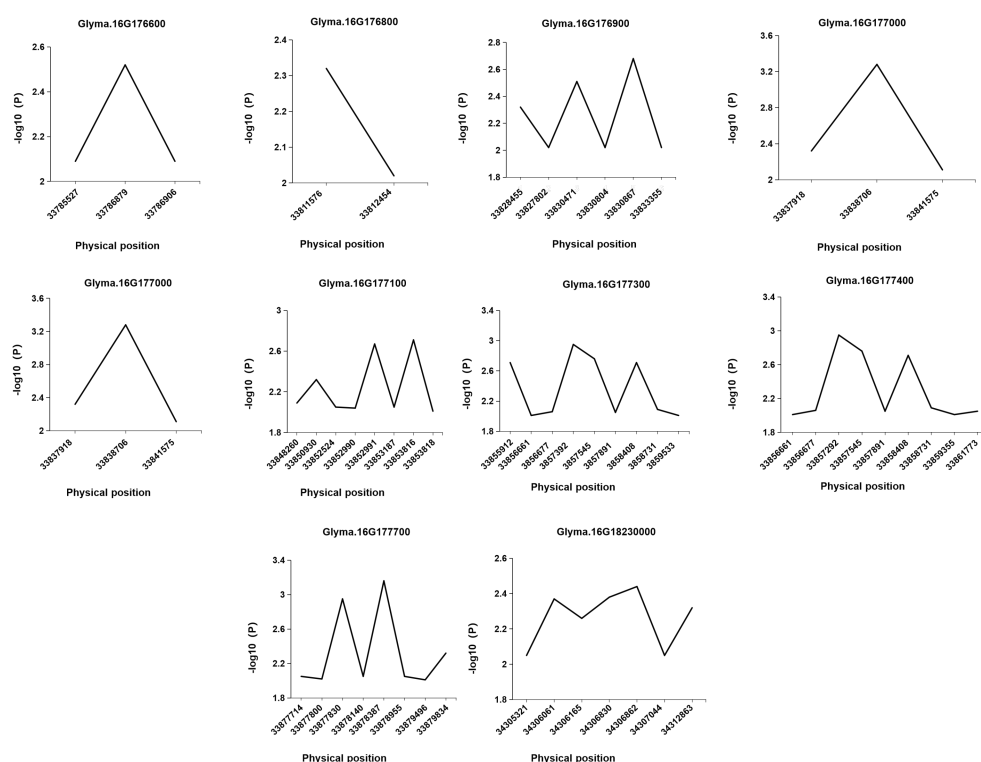
Figure S2: Candidate gene-based association. Gene-based association analysis of candidate genes with SNPs that were significantly correlated to partial resistance to FLS. Horizontal line indicated that the threshold was set to 2.0.
