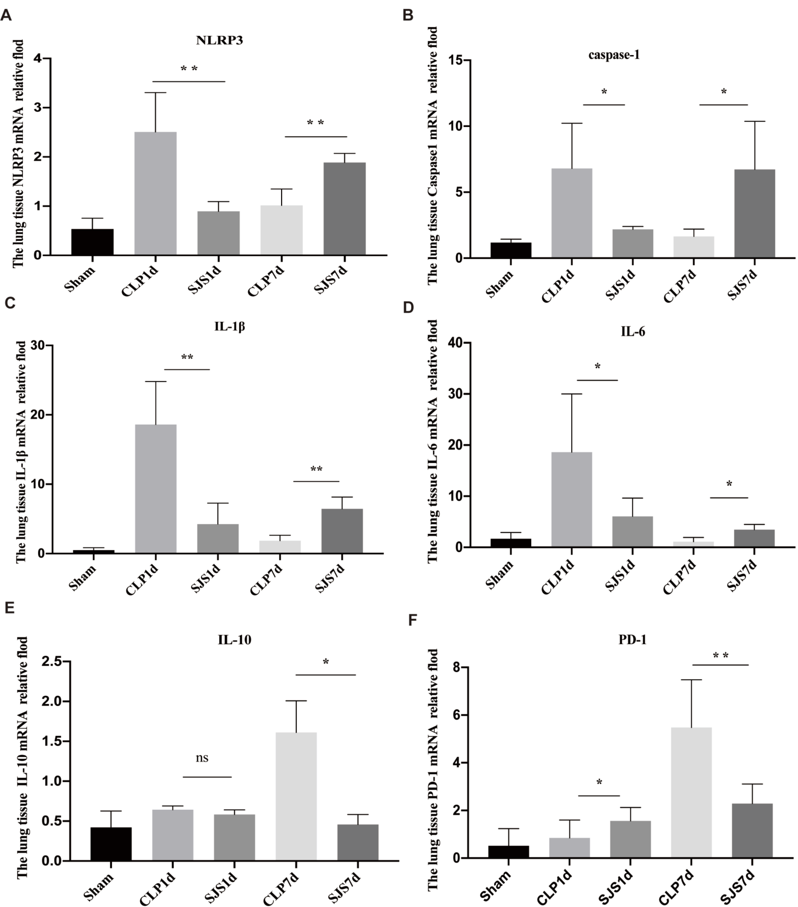
Fig. S1. SJS bidirectionally regulates immune homeostasis in lung injury with sepsis. A-F The mRNA levels of NLRP3、caspase-1、IL-1 \beta 、IL-6、IL-10、PD-1 using qRT-PCR (n=4) * P <0.05, ** P <0.01, ns no significant difference.
