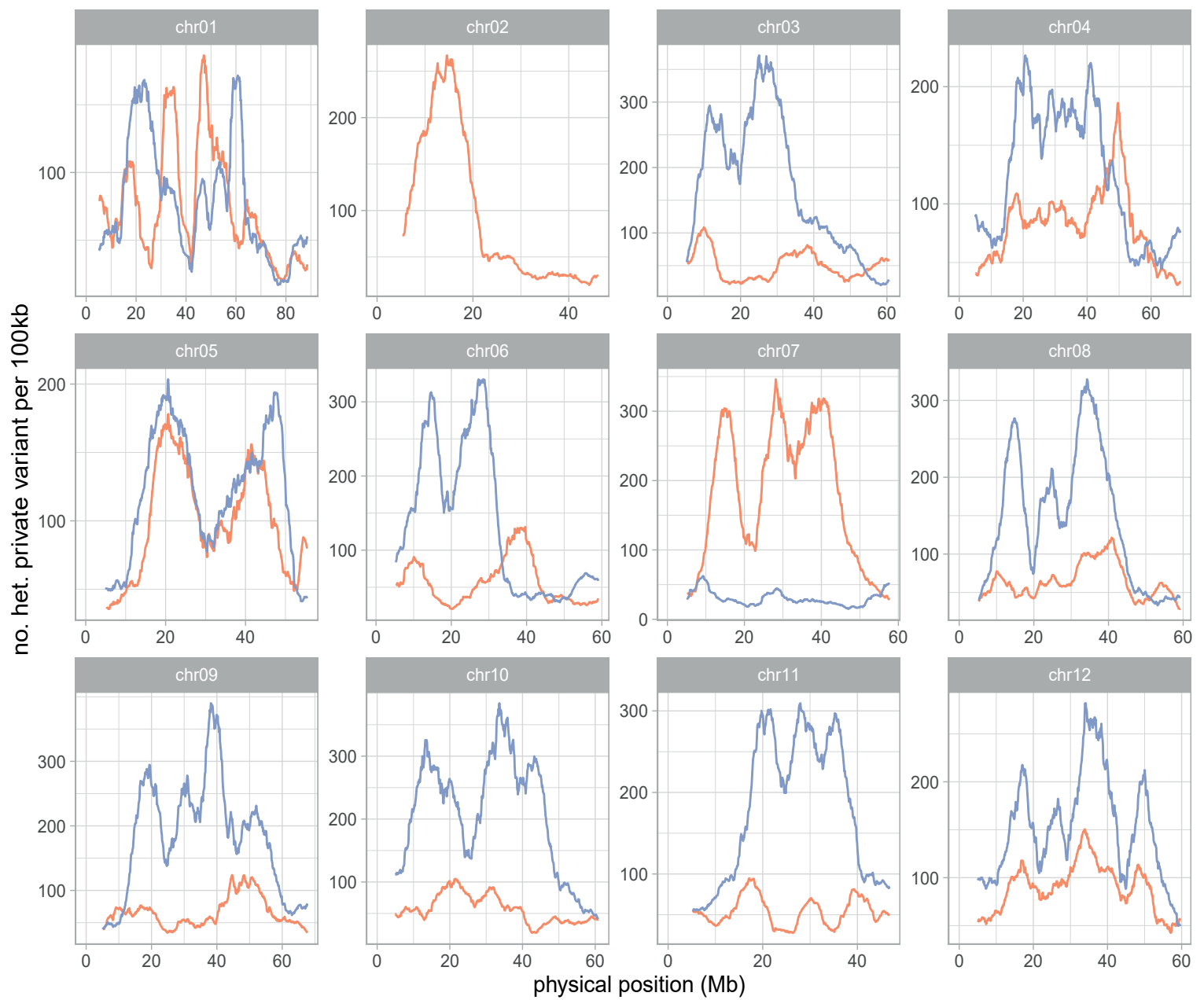
Suppl. Fig. 2: Five Mb moving average of the number of heterozygous parent-private variants across bins of 100 kb. Clone C data are displayed in orange and clone E in blue.
