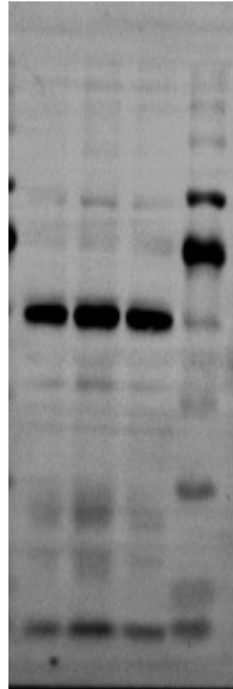
Beclin-1
