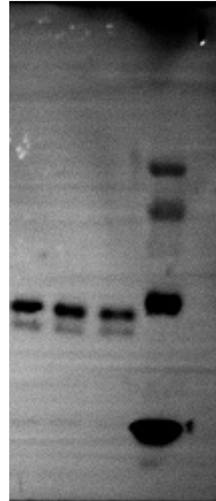
GAPDH
