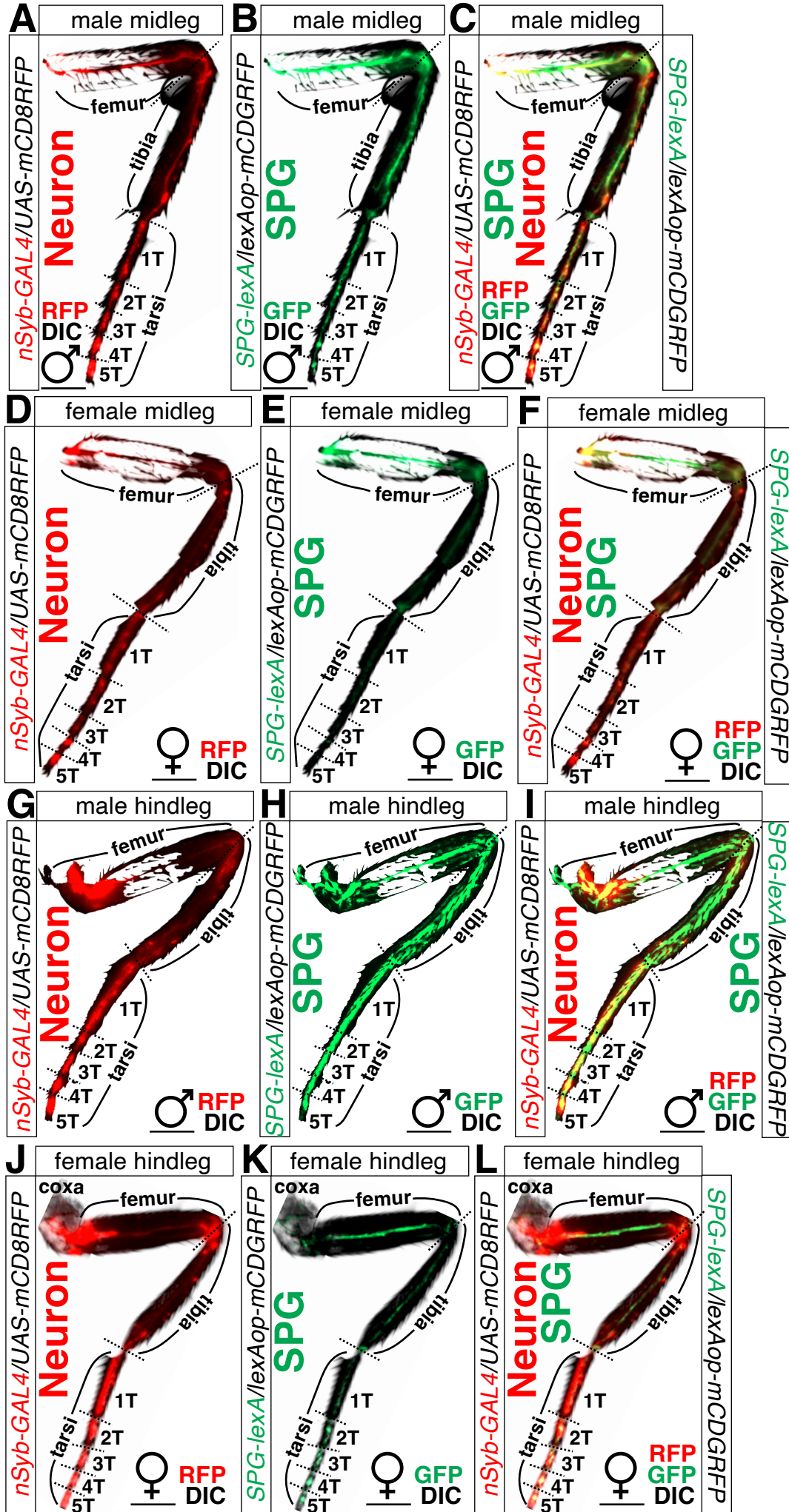
Snow., Fig.S12
