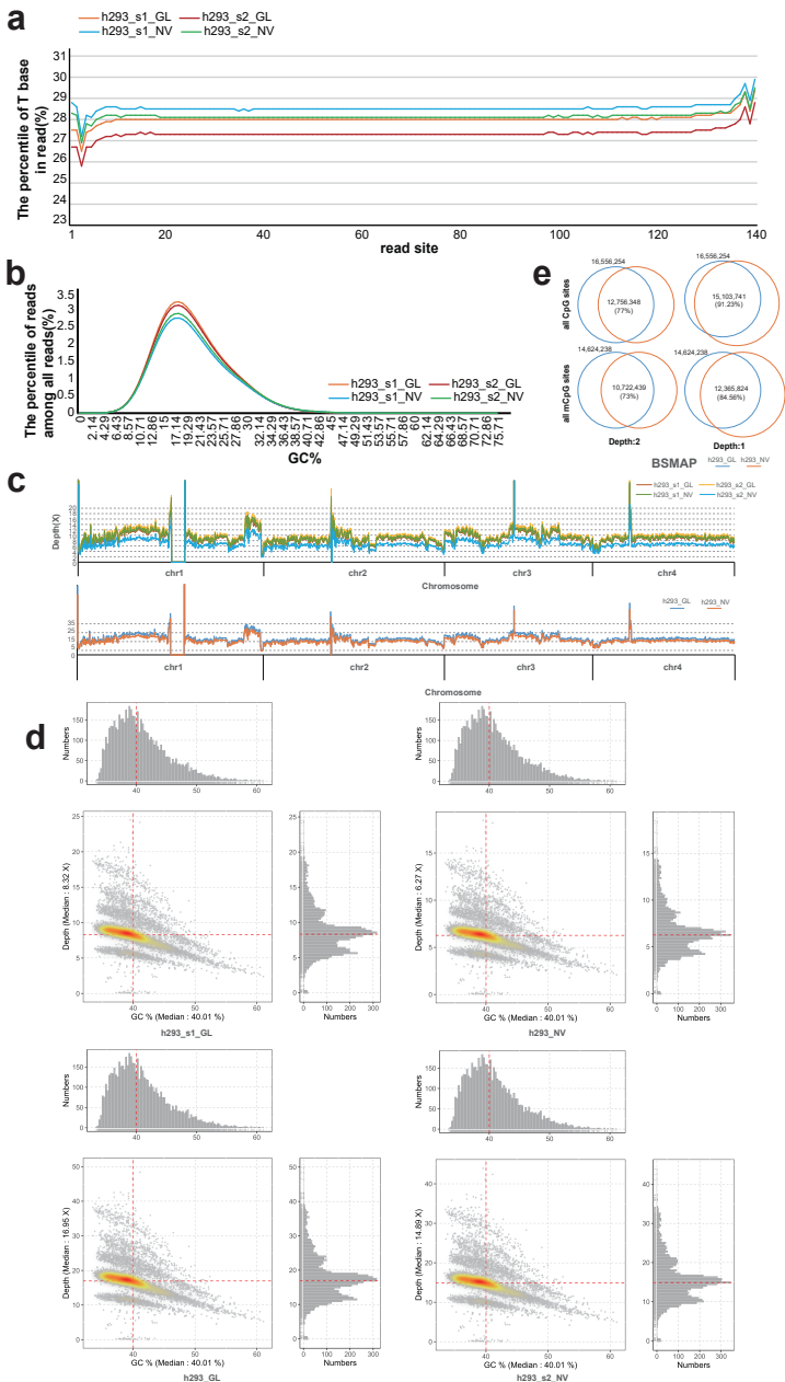
Supplementary Figure 6 The shortcoming for datasets. a The percentile of T base in reads. b The ratio of reads with different CG percentages. c The distribution of depth according to chromosomes in four samples and two platforms. d The relationship between GC percentage and different depth reads. e The overlap CpG sites between two platforms in different filter parameters
