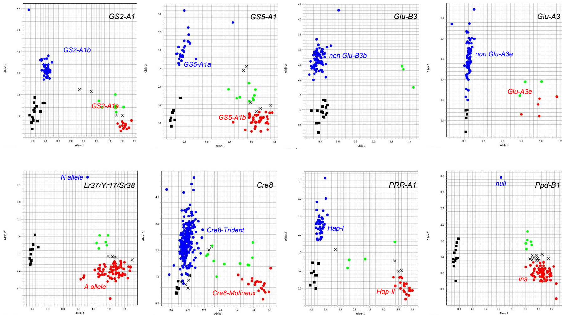
Additional file 12: Fig. S2. Scatter plots of eight genes identified using KASP genotyping. Red and blue dots show homozygous alleles, green and black dots represent heterozygous alleles and the negative control, respectively, and 'x' indicates missing types.
