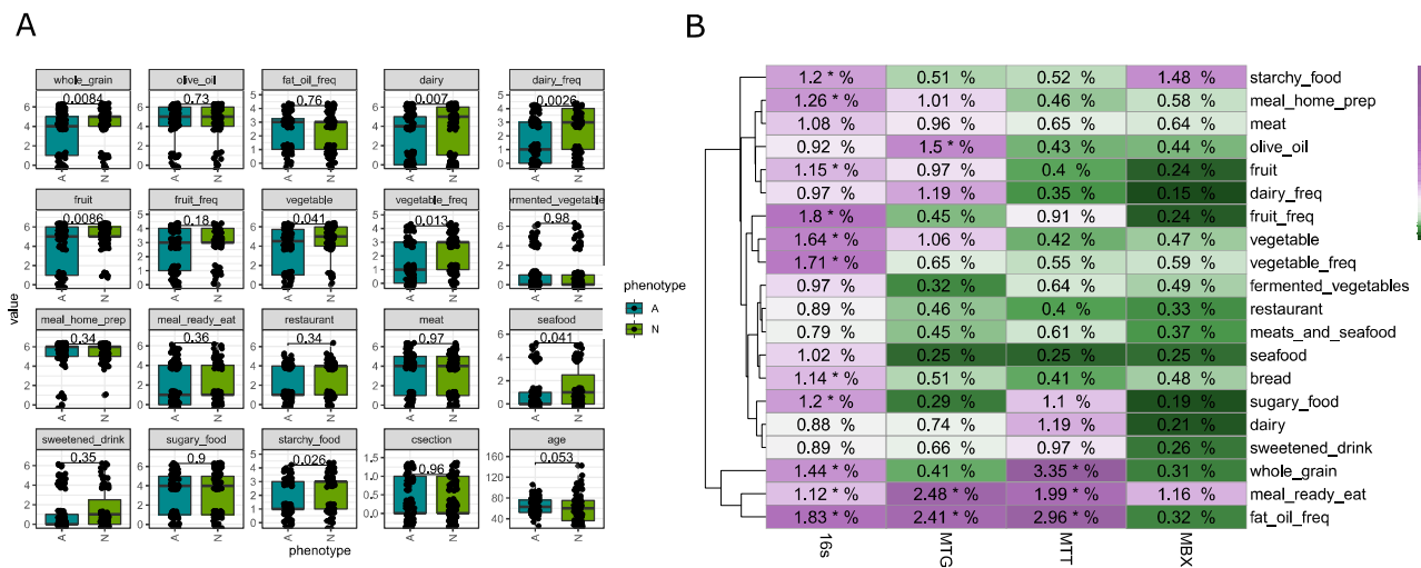
Supplementary Figure 2 Dietary and lifestyle characteristics between autistic and typically developing children compared using a Wilcoxon rank sum test (A). Association between individual dietary variables and omic data (B). Omic data was normalized using relative log expression (RLE), numbers in the cell are R^2 values as percents, and a star indicates a significant association by a permanova test
