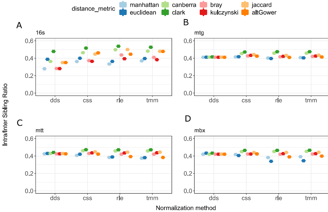
Supplementary Figure 9 Choosing a normalization method per omic datasets. Normalization methods that minimized the distance between siblings vs. the distance between all unrelated samples there selected. When differences in normalization performance were negligible, the majority method was used. 16S DeSeq2 (A), MTG RLE (B), MTT RLE (C), MBX RLE (D)
