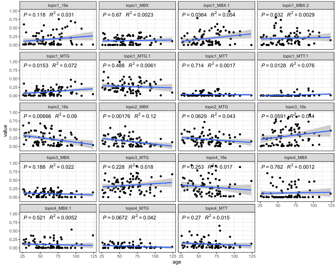
Supplementary Figure 5 Spearman correlation between age (in months) and topic values. Topic 2 most consistently correlates inversely with age, and Topic 1 correlates with age in some omics.
