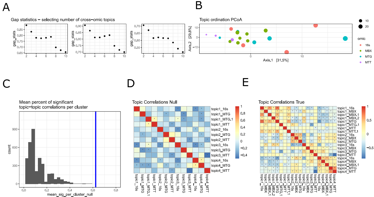
Supplementary Figure 1 Cross-omic topic evaluation
