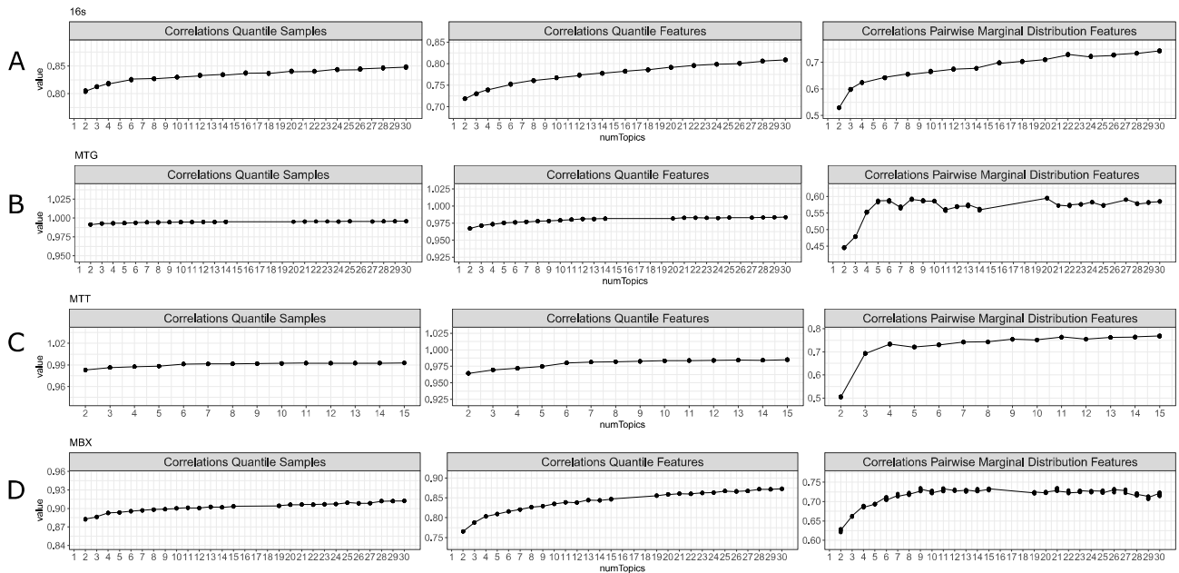
Supplementary Figure 10 Selecting number of topics per model. To evaluate model fit, sample data was simulated using each model, and simulated and true data were compared using three metrics: correlation of sample quantiles, correlation of feature quantiles, and marginal pairwise distribution of features. Number of topics was selected using the elbow method. The final number of topics selected were 4 for 16s data (A), 5 for MTG data (B), 4 for MTT data (C), and 7 for MBX data (D).
