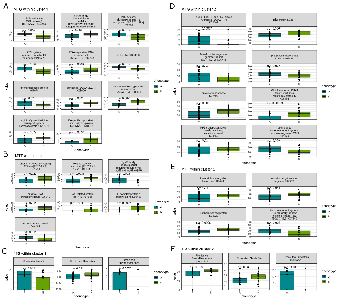
Supplementary Figure 8 Differential analysis of MTG, MTT, and 16S features between autistic and typically developing children within sample clusters as determined by topics. Within cluster 1, MTG features (A), MTT features (B), 16S features (C). Within cluster 2, MTG features (D), MTT features (E), 16s features (F). Features are first filtered using the Boruta package, and then p values are reported using Wilcox rank sum test.
