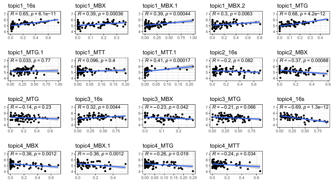
Supplementary Figure 3 Correlation between topic values and 16S Shannon diversity. Lines and confidence intervals are linear regression fits, while R and p values are spearman correlations.
