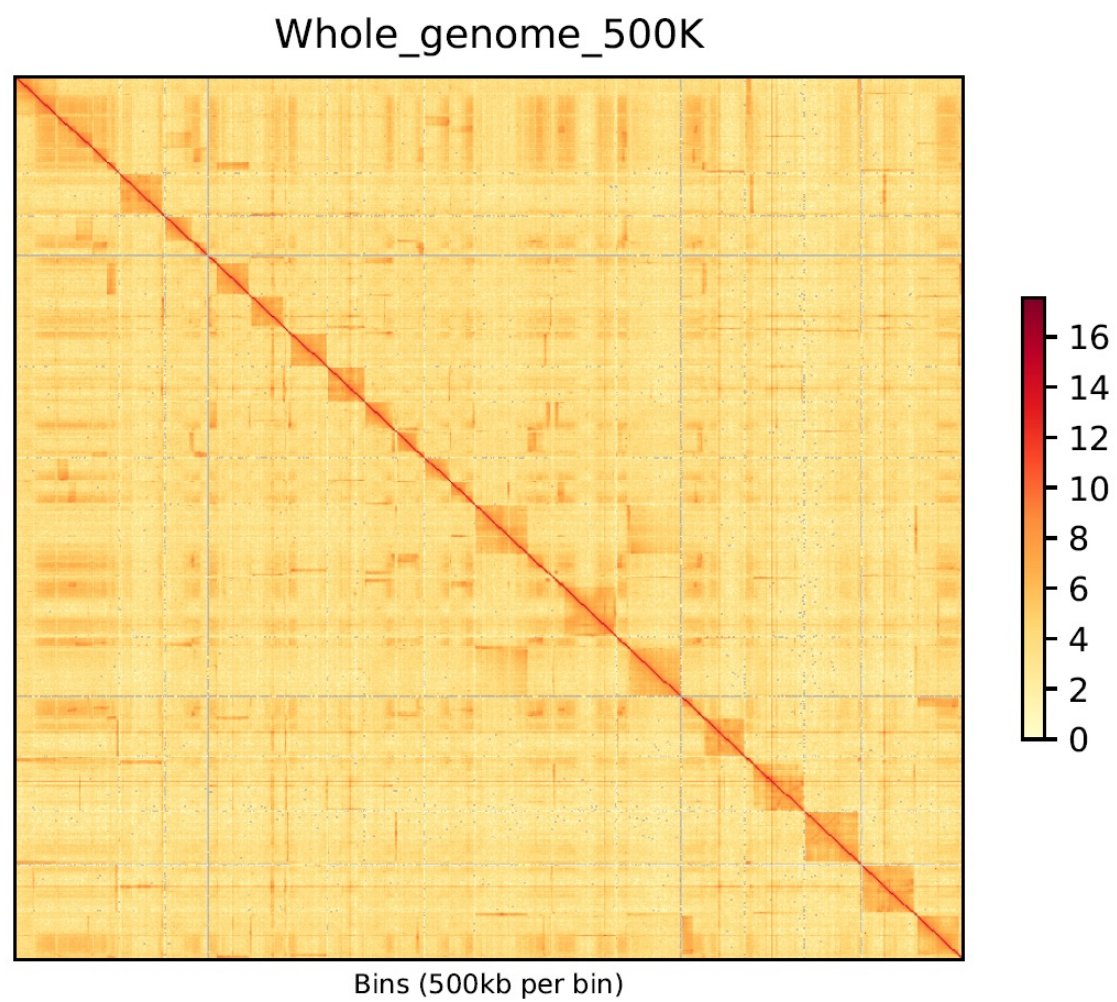
Figure S2. Hi-C interaction map of the S. exigua assembly.
