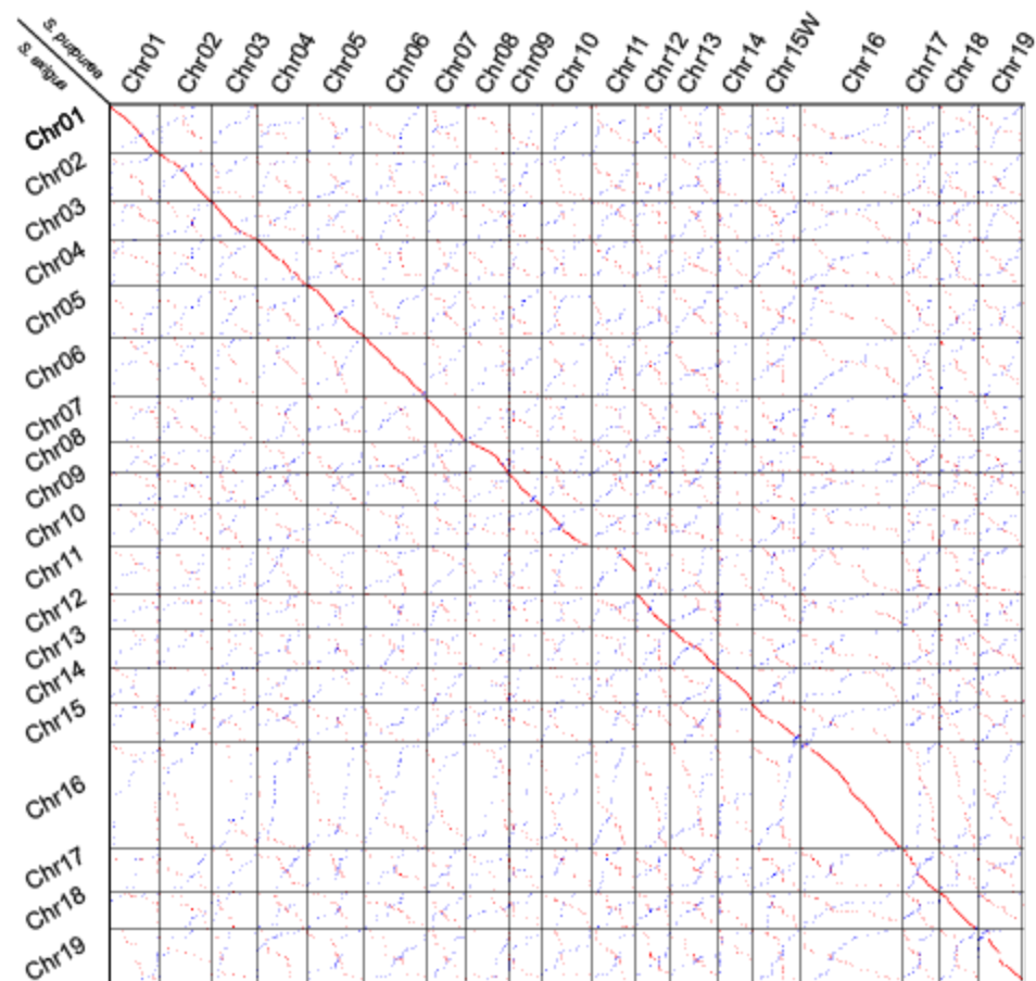
Figure S1. All-to-all alignment between our S. exigua male assembly and the S. purpurea reference genome v5.1 From JGI.
