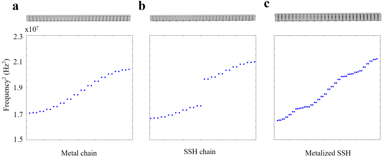
FIG. S2. Dispersion of the acoustic modes a Resonant spectrum of a periodic acoustic pattern. b Resonant spectrum of a SSH acoustic pattern. c Resonant spectrum of a metalized SSH acoustic pattern.
