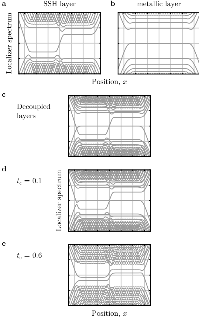
FIG. S4. Evolution of the localizer's spectrum as the inter-layer coupling is increased. a Localizer spectrum at E = 0 for the SSH layer in isolation, with t_{\text{in}} = 0.4 and t_{\text{out}} = 1 . b Similar, except for the metallic layer in isolation, with t_M = 1 . c , d , e Localizer spectrum at E = 0 for the two-layer system, with t_{\text{in}} = 0.4 , t_{\text{out}} = 1 , t_M = 0.8 , and t_c = 0, 0.1 , and 0.6 .
