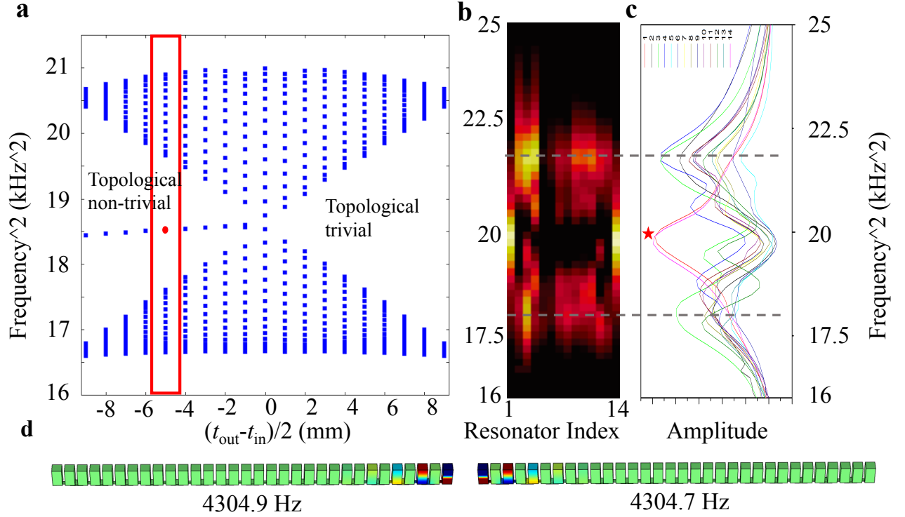
FIG. S1. Experimental mapping of the SSH model resonant spectrum. a COMSOL simulated SSH model resonant spectrum. The red vertical box indicates t_{\text{in}} = 15 mm and t_{\text{out}} = 5 mm, used in the experiments. b Experimentally measured local density of states, assembled from normalized microphone readings from the top of the block resonators. The bright dispersive modes indicates the bulk and edge modes. c Collapse on the frequency axis of the intensity plot in b . The spectral gap can be clearly identified and the edge modes show up in the gap marked as red asterisk. d Acoustic pressure field distribution for the edge modes marked as red dot in panel a
