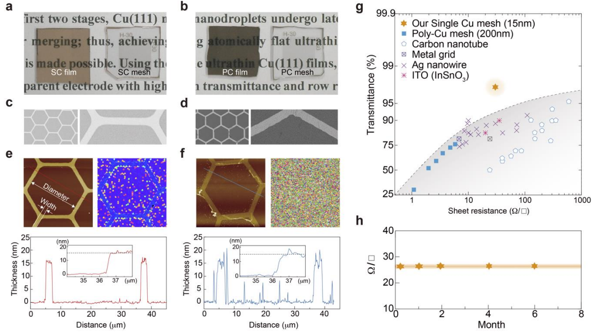
Supplementary Fig. 11. Transparent Cu mesh electrodes. a , A 15-nm-thick single-crystal (SC) Cu film and SC honeycomb mesh electrode on a sapphire substrate. b , A polycrystalline (PC) Cu film and PC honeycomb mesh electrode with a thickness of 15 nm deposited on a glass substrate. c , d , Scanning electron microscope images of (c) SC and (d) PC meshes. Enlarged images are also displayed. e , (Upper left) atomic force microscopy (AFM) image and (upper right) electron backscatter diffraction map of the SC mesh and (lower) its height profile along the indicated line, as obtained by AFM, along with (inset) a magnified view of part of the profile. f , Corresponding images and profile of the PC mesh. g , Comparison of the transmittance at 550 nm and sheet resistance of our SC mesh with those reported for other trichloroethylene materials, including carbon nanotubes, metal grids, Ag nanowires, and indium tin oxide. 34 h , Sheet resistances (Ω/sq) of freshly prepared and 1-, 2-, 4- and 6-month-old samples, which demonstrate the aging effect.
