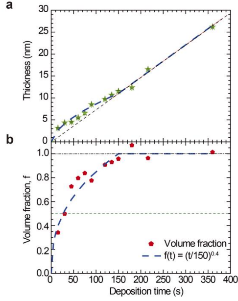
Supplementary Fig. 10. Estimates of the volume fractions ( f ) of Cu films based on the relationship between thickness and deposition time. a , Thickness as a function of deposition time. b , Estimated volume fraction as a function of deposition time. The thick blue dashed line is a guide for the eye. The measured thicknesses may include some uncertainties.
