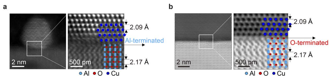
Supplementary Fig. 6. Transition of surface termination during growth. a , Structures of the Cu nanodroplet/ \text{Al}_2\text{O}_3 . b , Cu film/ \text{Al}_2\text{O}_3 interfaces with an orientation relationship of (111)_{\text{Cu}}// (0001)_{\text{Al}_2\text{O}_3} .
