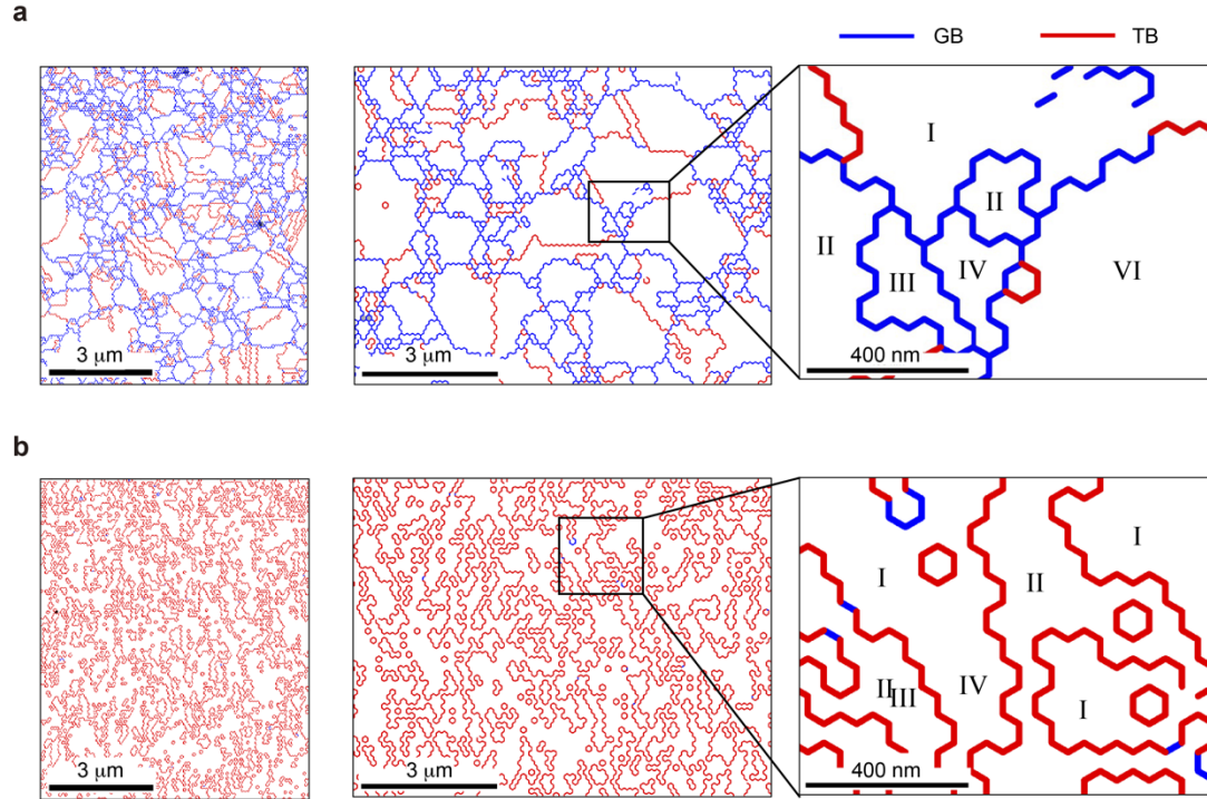
Supplementary Fig. 4. Grain boundaries (GBs) and twin boundaries (TBs). a , Misorientation line distributions for a polycrystalline film. Red and blue lines denote TBs and GBs. Regions in the magnified image (third column) have various orientations (ORs). b , Misorientation line distributions for a single-crystal Cu film. Misorientation lines are composed mostly of TBs. There are one of two ORs in the regions in the magnified image in the third column.
