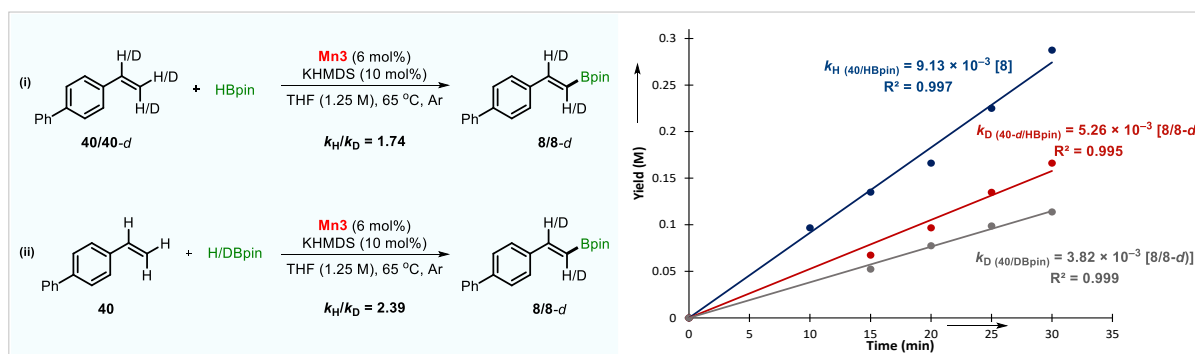
Fig. S7. Yield vs time plot for determination of kinetic isotope effect.
