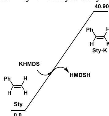
Fig. S14. Potential energy surface of deprotonation of unbound styrene.
