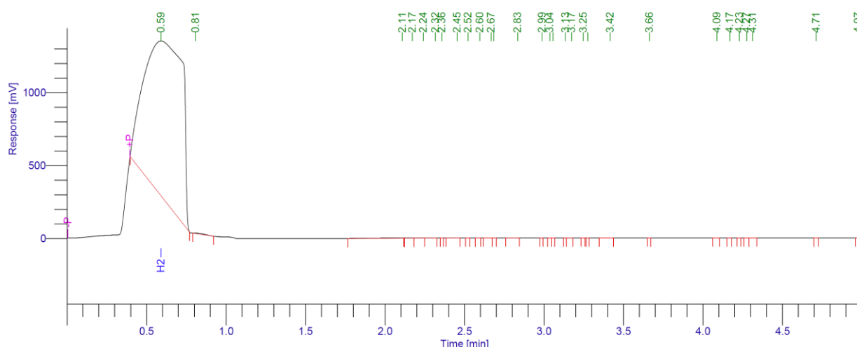
Fig. S4. GC sample of the gas phase for the standard dehydrogenative borylation.
