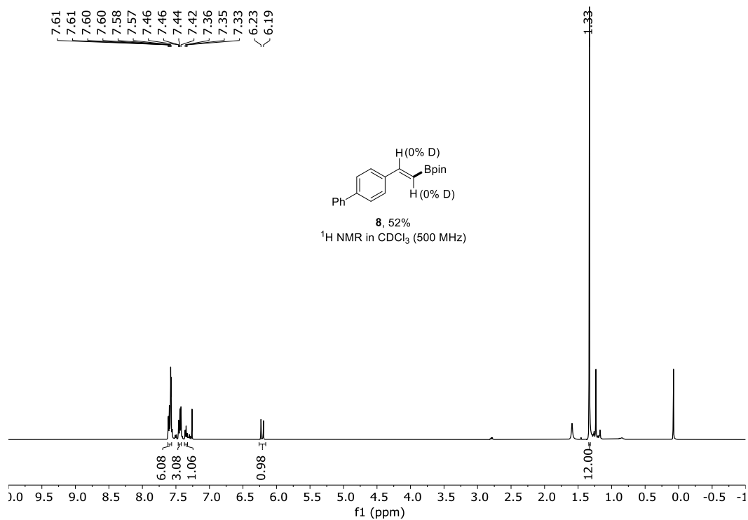
Fig. S6: 1 H NMR of 8 .
