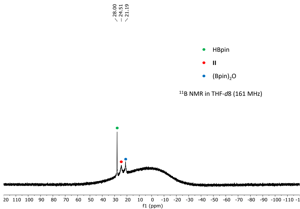
Fig. S12. ^{11}\text{B} NMR spectra of Mn3 after treatment with KHMDS and HBpin.
