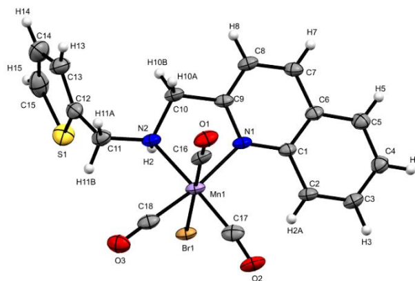
Fig. S2. ORTEP diagram of Mn3 (50% probability ellipsoids). 3
