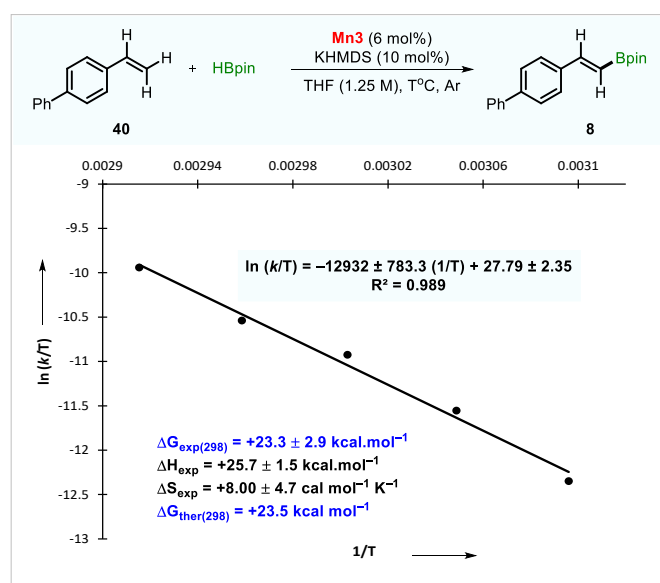
Fig. S9: ln ( k/T ) vs 1/T plot for Eyring analysis.
