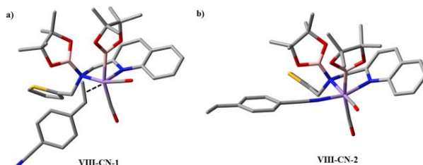
Figure S17. Optimized geometries for (a) \pi -bound ( VIII-CN-1 ) and (b) nitrile bound ( VIII-CN-2 ) intermediates while 4-cyano styrene was used as substrate.
