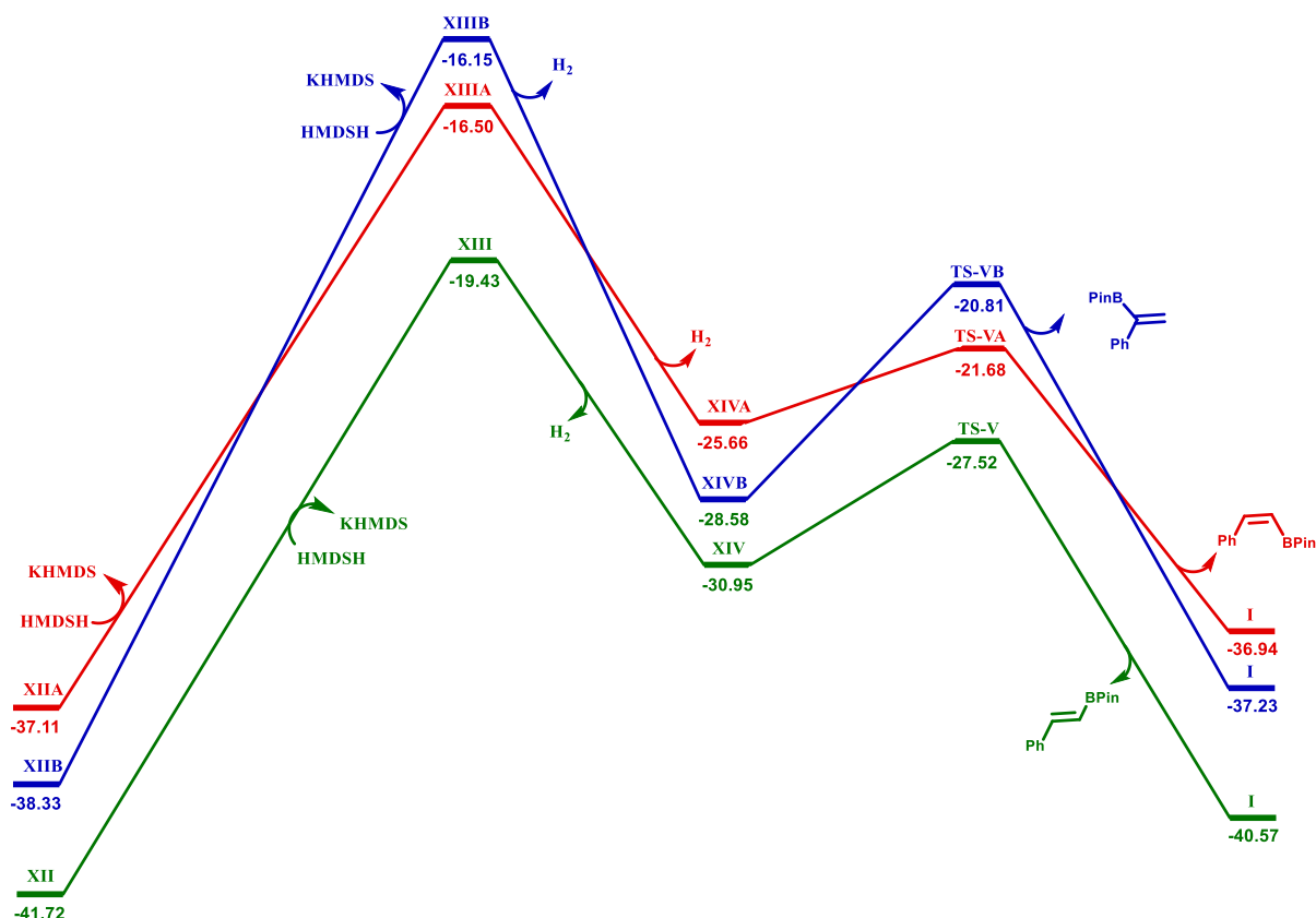
Fig. S16. Potential energy surface for the formation of different regioisomers.
