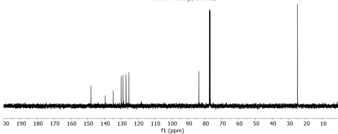
( E )-2-(3-chlorostyryl)-4,4,5,5-tetramethyl-1,3,2-dioxaborolane ^{13}\text{C} NMR in \text{CDCl}_3 (126 MHz)
