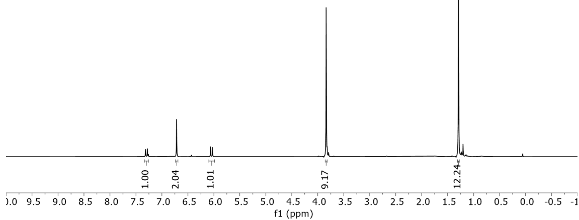
( E )-4,4,5,5-tetramethyl-2-(3,4,5-trimethoxystyryl)-1,3,2-dioxaborolane ^1\text{H} NMR in \text{CDCl}_3 (500 MHz)
