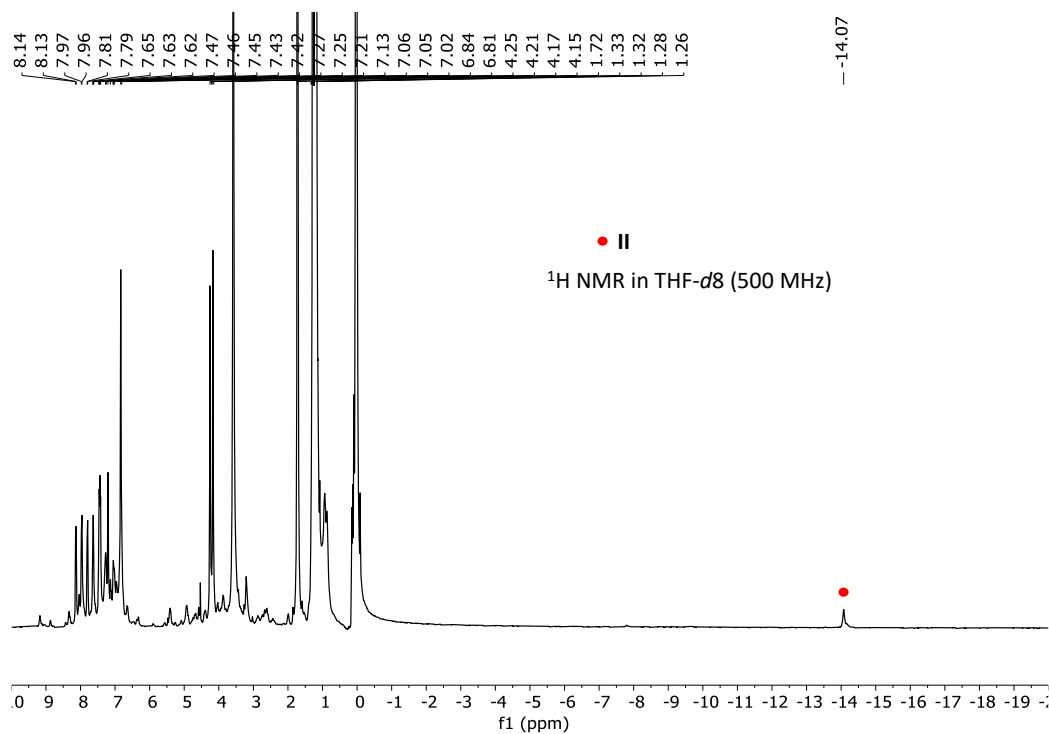
Fig. S11. ^1\text{H} NMR spectra of Mn3 after treatment with KHMDS and HBpin.
