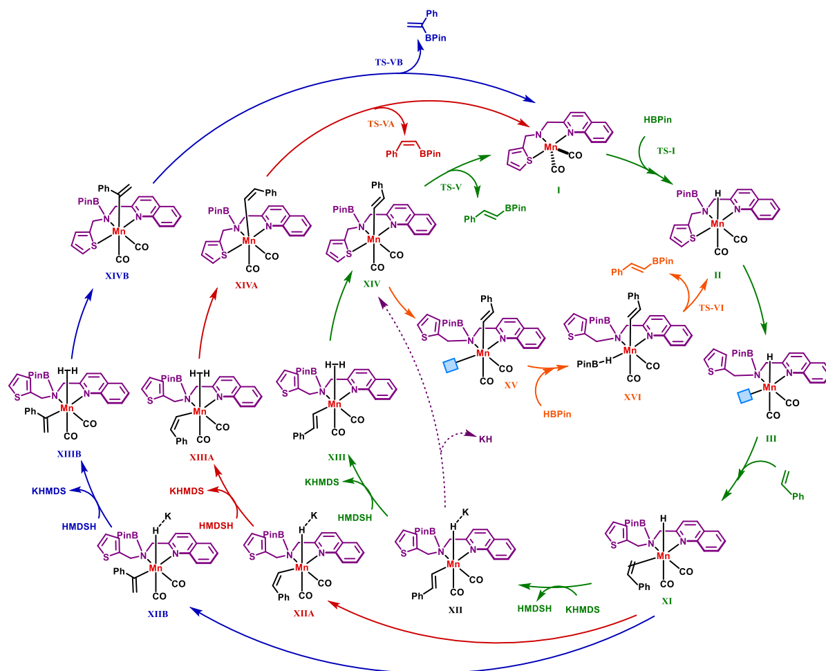
Fig. S13. Proposed alternative pathway for catalytic dehydrogenative borylation of olefins.
