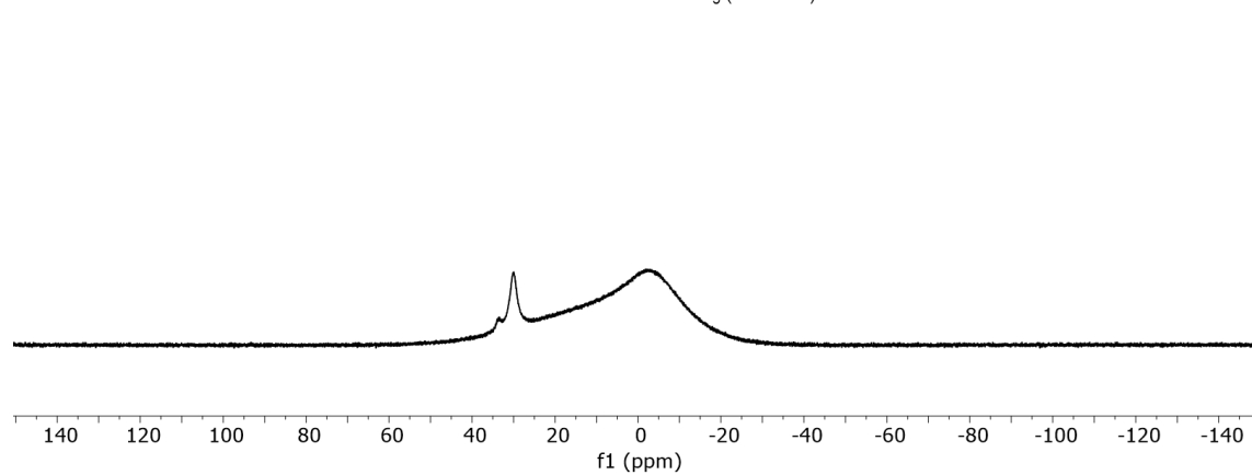
( E )-2-(3-chlorostyryl)-4,4,5,5-tetramethyl-1,3,2-dioxaborolane ^{11}\text{B} NMR in \text{CDCl}_3 (161 MHz)
