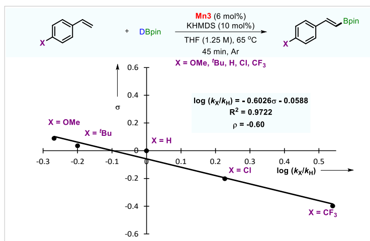
Fig. S8: \log(k_X/k_H) vs \sigma plot for Hammett correlation study.
