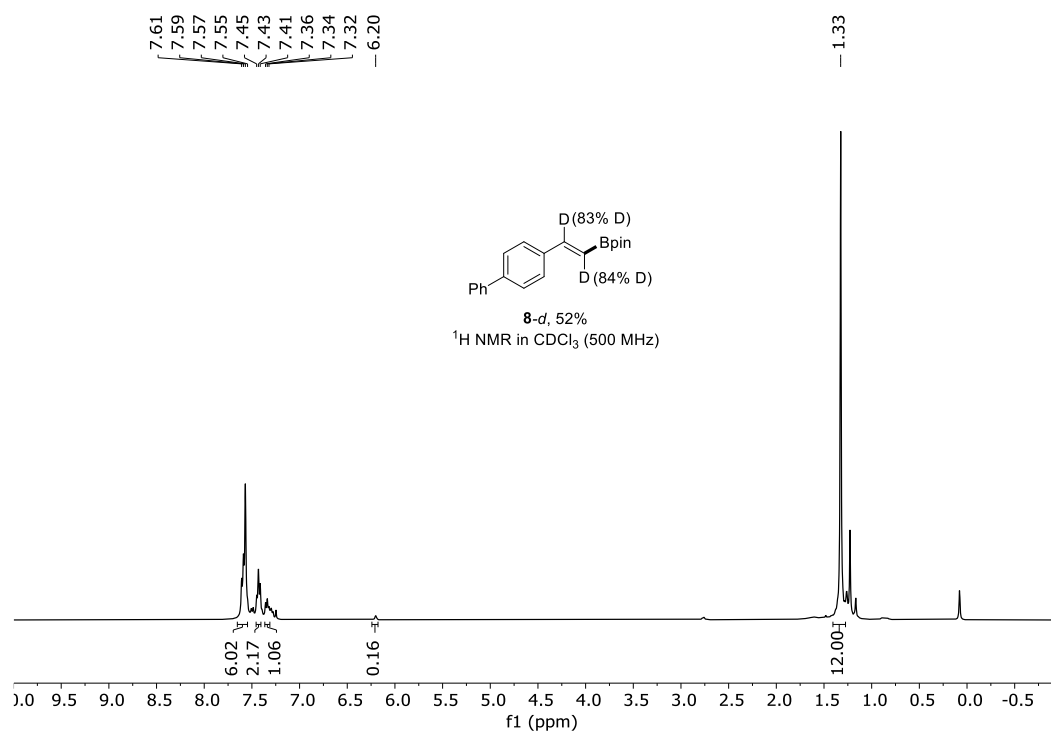
Fig. S5: 1 H NMR of 8-d .
