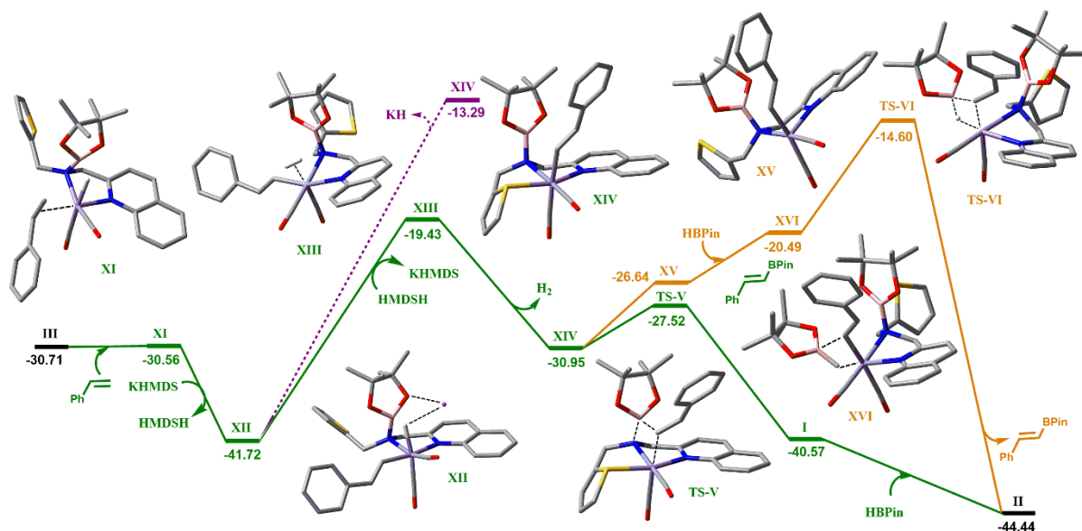
Fig. S15. Potential energy surface of alternate pathway for catalytic dehydrogenative borylation of olefins.
