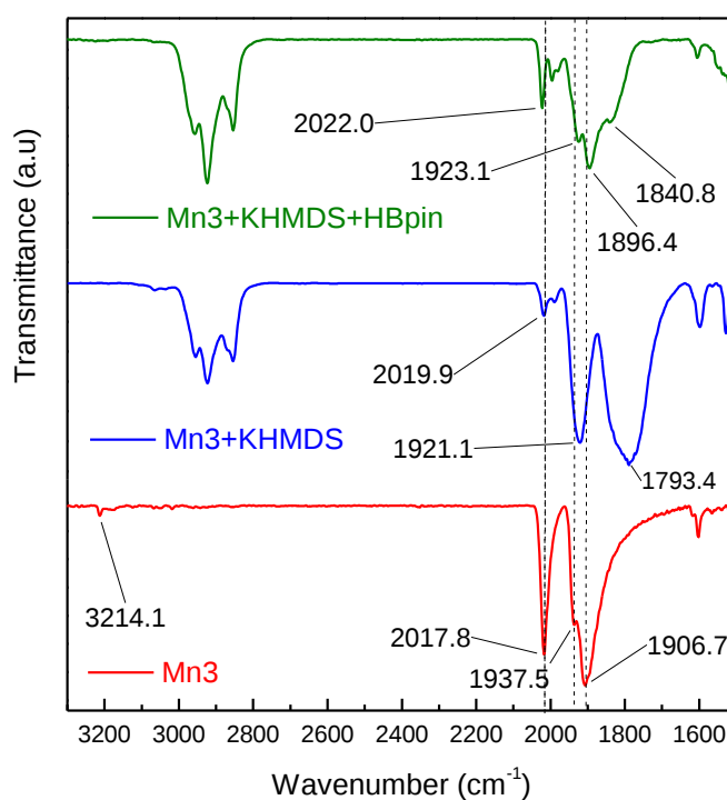
Fig. S10. IR spectrum for a) Mn3 catalyst; b) Mn3 catalyst after treatment with KHMDS; c) Mn3 catalyst after treatment with KHMDS and HBpin.
