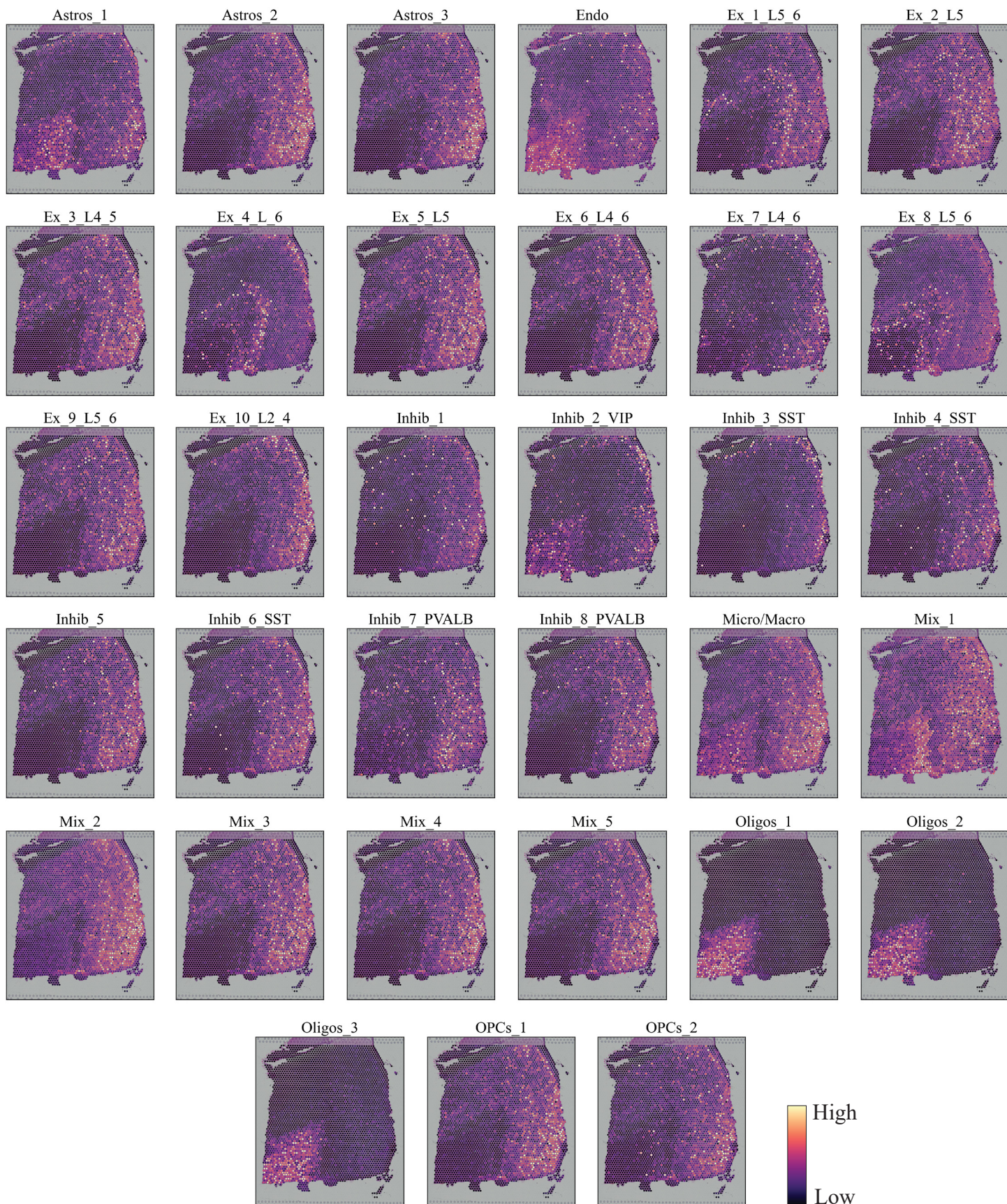
Figure S7. cell2location predicted spatial distributions of all 33 cell types in the 151673 slice of DLPFC dataset.
