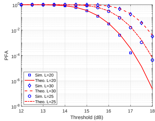
Figure 4: PFA versus threshold value for different L .
