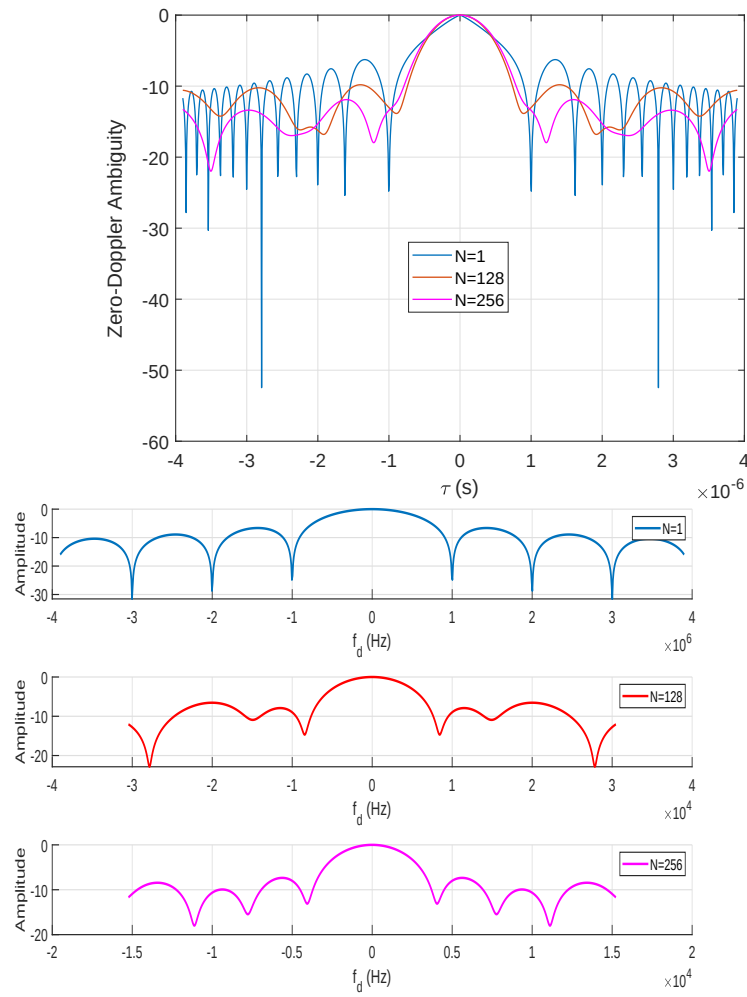
Figure 8: Amplitude of the OCDM CAF: a-(top)) zero-Doppler cut, b-(bottom)) zero-delay cut
