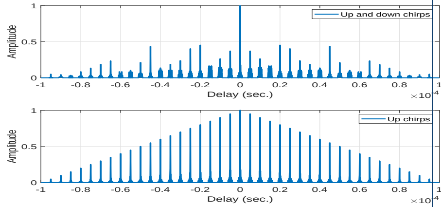
Figure 6: Zero-Doppler cut of the CAF for a sequence of a-(top)) up- and down-chirps, b-(bottom)) only up-chirps
