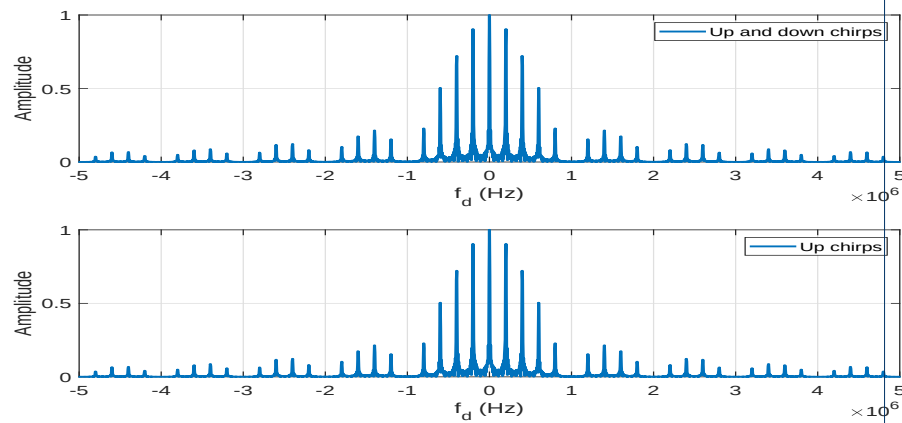
Figure 7: Zero-delay cut of the CAF for a sequence of a-(top)) up- and down-chirps, b-(bottom)) only up-chirps
