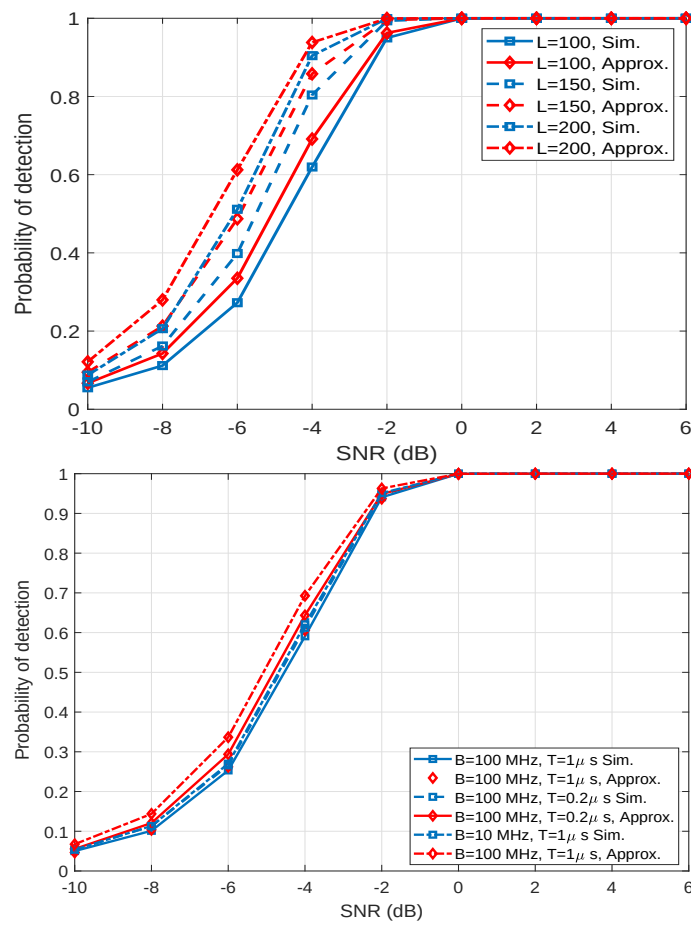
Figure 5: Probability of detection versus SNR for a-(top)) different L , b-(bottom)) different time-bandwidth product
