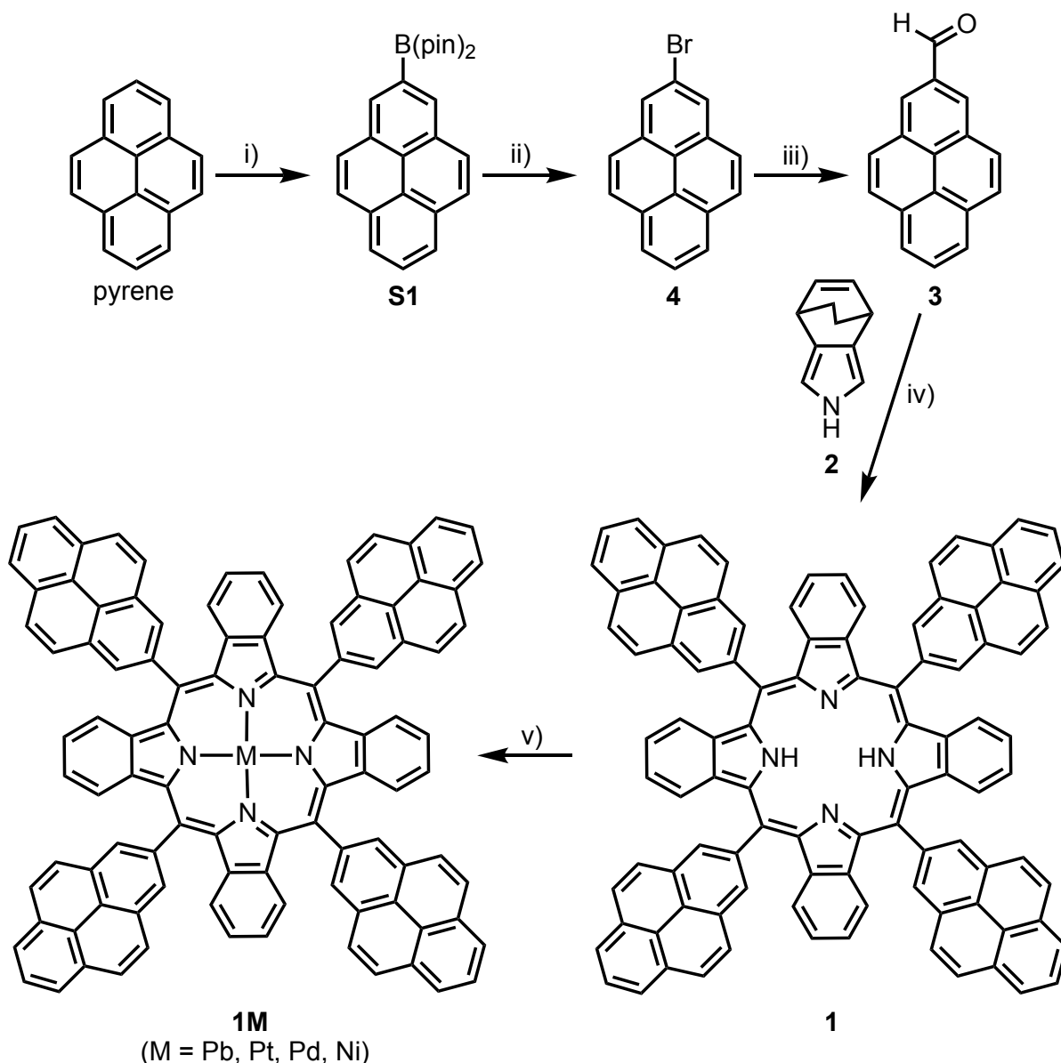
Fig. S1. Synthetic scheme to benzoporphyrin 1M. i) B_2pin_2 (1.1 equiv), [[Ir(\mu-OAc)cod]_2] (1 mol%), dtbpy (2 mol%), hexanes, 80 °C, 16 h ( S1 65%); ii) CuBr_2 (3.0 equiv), MeOH/H 2 O (1:1), 90 °C, 16 h ( 4 83%); iii) 1. n -BuLi (2.2 equiv), Et 2 O, -20 °C, 1 h, then 30 min, rt; 2. DMF (40 equiv), rt, 1 h; 3. 10% HCl ( 3 53%). iv) 1. 4,7-dihydro-2H-ethanoisoindole 2 , BF_3 \cdot OEt_2 , CH_2Cl_2 , rt, 20 h; 2. DDQ, reflux, 2 h; 3. 200 °C, 1.5 h ( 1 81%); v) 1Pb : Pb(OAc)_2 \cdot 3H_2O (15 equiv), DMF, 140 °C, 2 h; 1Pt : Pt(acac)_2 (15 equiv), PhCN, 180 °C, 3 h; 1Pd : PdCl_2 (15 equiv), PhCN, 180 °C, 3 h; 1Ni : Ni(acac)_2 (20 equiv), toluene, 130 °C, 1 h. B_2pin_2 = bis(pinacolato)diboron; cod = cyclooctadiene; dtbpy = 4,4'-di- tert -butyl-2,2'-dipyridyl; DMF = N,N -dimethylformamide; DDQ = 2,3-dichloro-5,6-dicyano-1,4-benzoquinone; acac = acetylacetonate.
