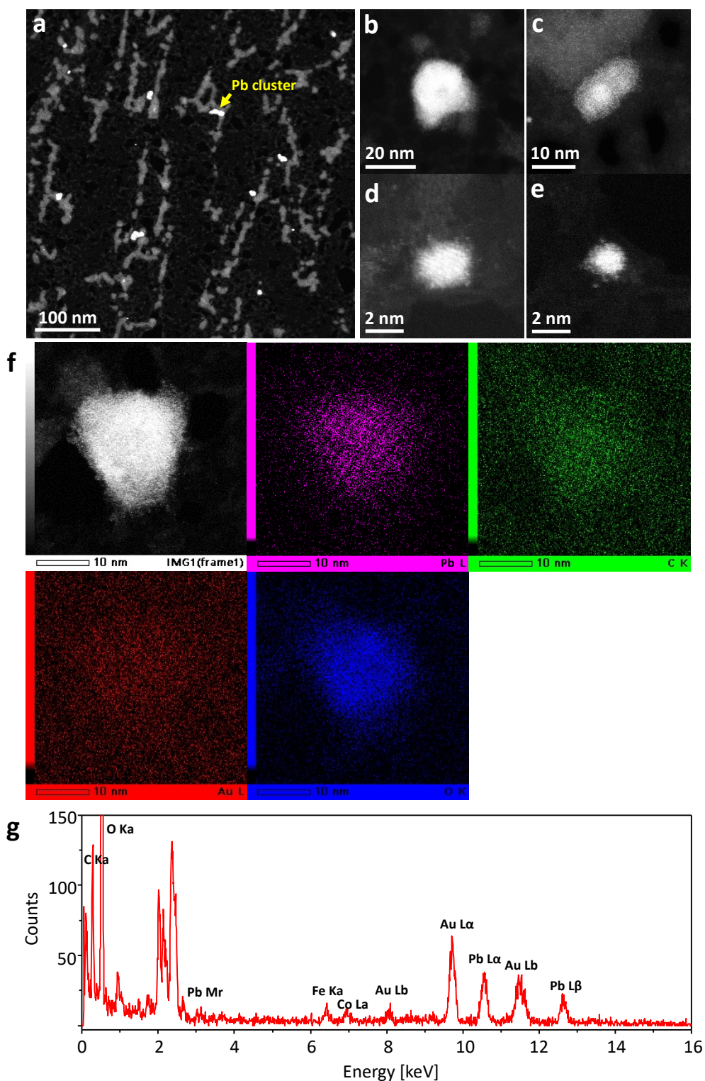
Fig. S14. STEM-EDX analysis of Pb aggregates. a-e, HAADF-STEM images of the Pb aggregates. f, EDS elemental mapping of Pb. (g) EDX spectrum.
