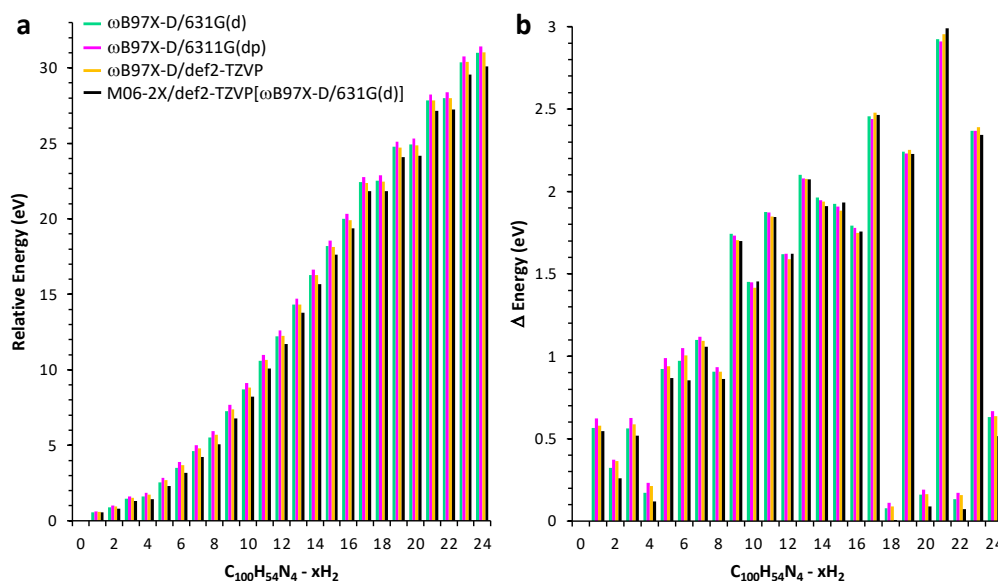
Fig. S15. Comparison of density functionals and basis set on thermochemical results.
