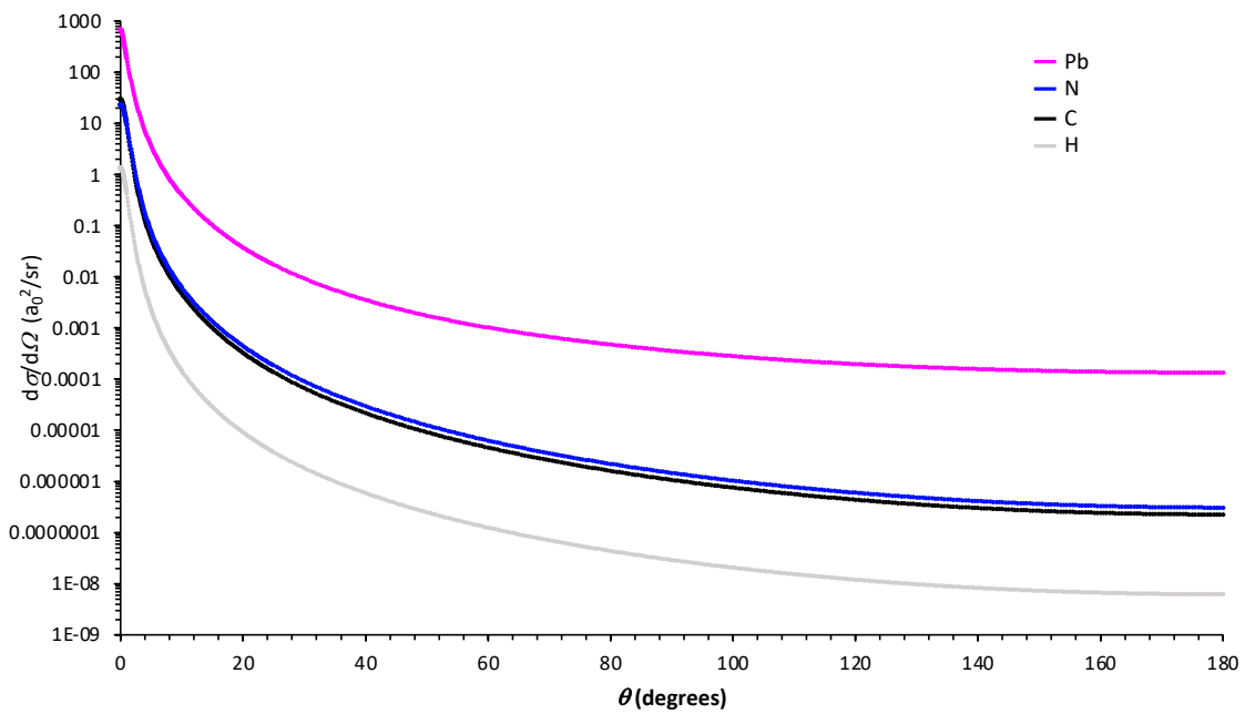
Fig. S2. Differential elastic-scattering cross-section of H, C, N, and Pb at 80 keV. a_0 = Bohr radius ( a_0^2 = 2.8002852 \times 10^{-21} \text{ m}^2 ); Total cross-section: H = 1.55 \cdot 10^{-3} a_0^2 ; C = 3.42 \cdot 10^{-2} a_0^2 ; N = 3.68 \cdot 10^{-2} a_0^2 ; Pb = 9.56 \cdot 10^{-1} a_0^2 .
