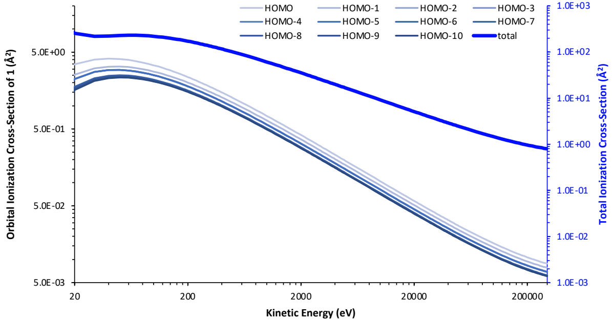
Fig. S3. Electron-impact ionization cross-section of 1. Calculated with the relativistic Binary Encounter Bethe model for the valence orbitals HOMO – HOMO-10, and the total ionization cross-section over all orbitals.
