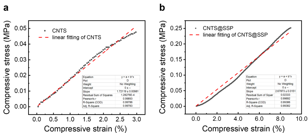
Supplementary Figure 2. (a) The compressive stress-strain curve of CNTS was linearly fitted at the strain of 0-3 %; (b) The compressive stress-strain curve of CNTS@SSP was linearly fitted at the strain of 0-9 %.
