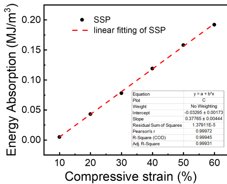
Supplementary Figure 4. The energy absorption curve of SSP was linearly fitted at the compressive strain of 10 % - 60 %.
