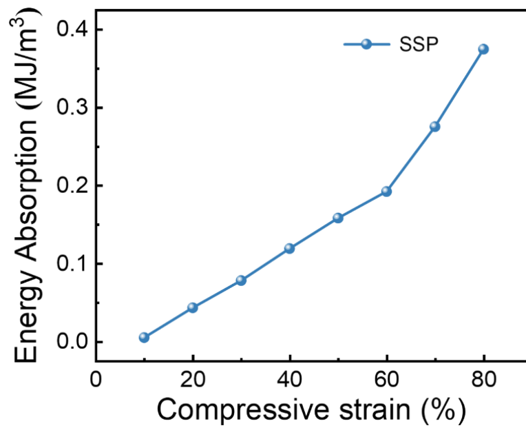
Supplementary Figure 3. Energy absorption curve of SSP at 10 % - 80 % compressive strain.
