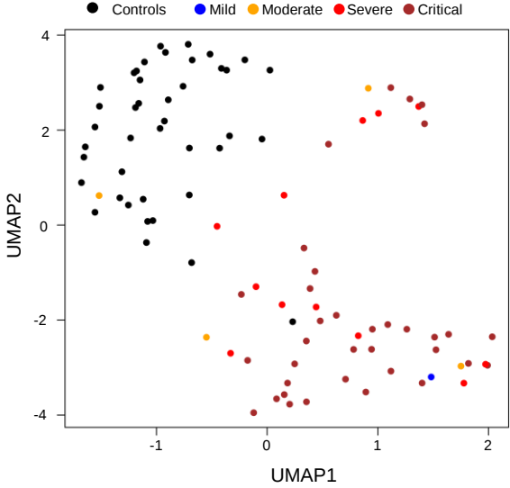
Supplementary Fig. 1. UMAP plot representing the proteomic profiles in non-pregnant patients by disease severity. Black = control, blue = mild case, yellow = moderate case, red = severe case, brown = critical case.
