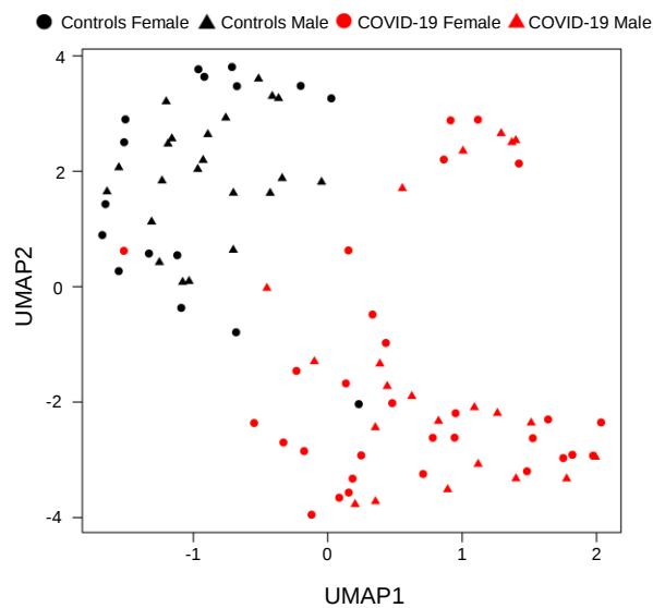
Supplementary Fig. 2. UMAP plot representing the proteomic profiles of non-pregnant patients according to sex. Black = control, red = case. Circle = female, triangle = male.
