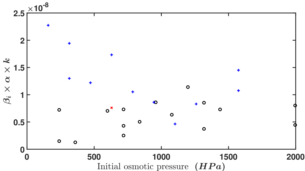
Figure S3: Calculated coefficient \beta\alpha k as a function of the calculated osmotic pressure at initial time for both dextrans. Black circles denote D6, blue crosses denote D20 and red star denote D20 with a 3.5 K membrane.
