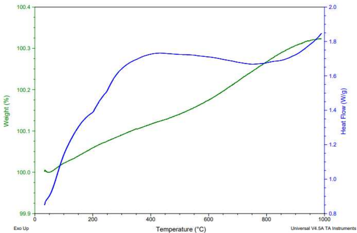
Fig. 3c DSC-TGA curves of NN-3
