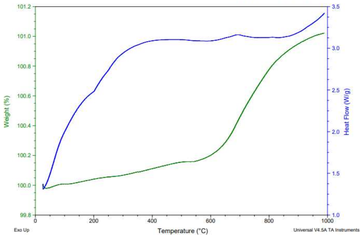
Fig. 3b DSC-TGA curves of NN-2
