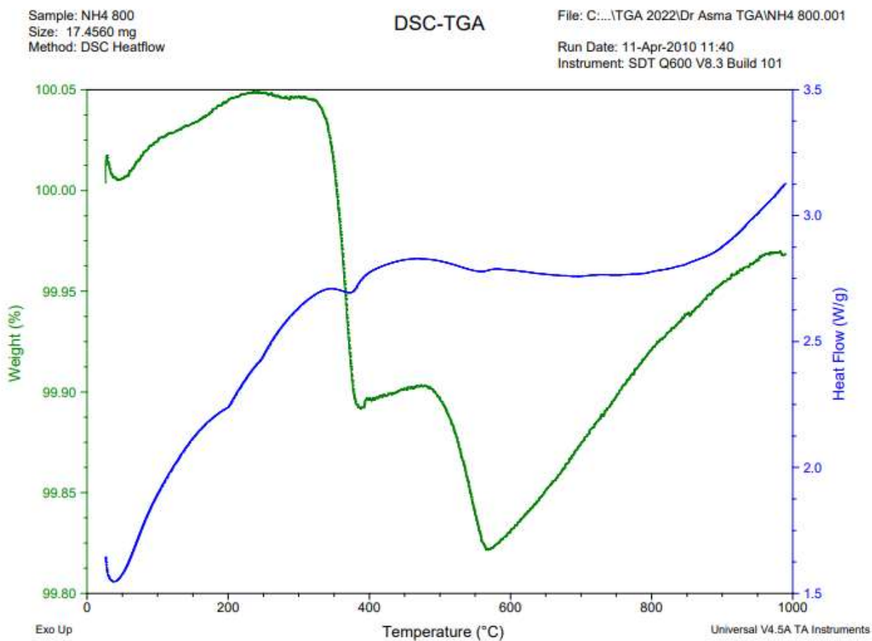
Fig. 3d DSC-TGA curves of NN-4
