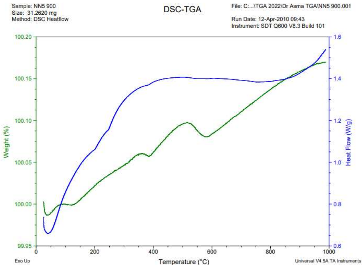
Fig. 3e DSC-TGA curves of NN-5
