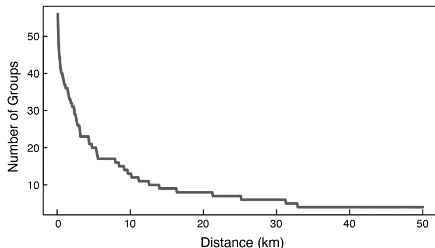
Fig. S3. Number of groupings owing to changes in distance (km) calculated from hierarchical clustering using pairwise Euclidean distances between reefs. The number of unique groups showed a rapid decline up to and over 10 km. We therefore explored section sizes of 10 – 30 km (in 5 km increments) as the random factor in our GAMM models. Regardless of section size, the random factor remained non-significant in all of our models.
