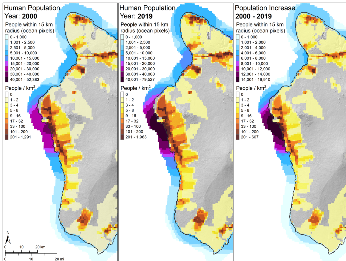
Fig. S5. Human population density on land from NASA GPW v4 and calculated data layer showing the total population within 15 km of each nearshore oceanic pixel for years 2000 (left), 2019 (middle), and increase from 2000 to 2019 (right).
