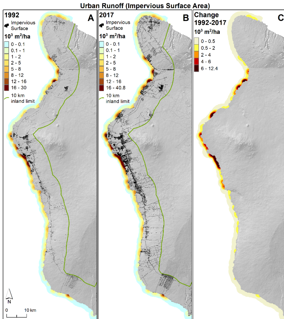
Fig. S13. Maps showing the impervious surface land use footprint on land (black) within 10 km inland of the shoreline (green line), and derived proxy for urban runoff into coastal waters for years (A) 1992, (B) 2017, and (C) the increase from 1992 – 2017.
