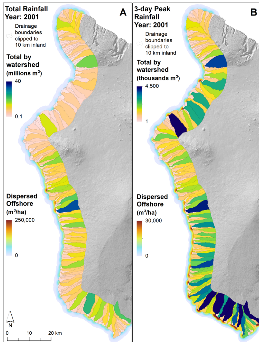
Fig. S15. Map showing the annual total (A) and peak 3-day total (B) rainfall for example year 2001. Totals from interpolated rainfall by watersheds clipped to 10 km inland are shown on land, and dispersed offshore. Layers are symbolized relative to the range in values over the full 30-year time series (1990 - 2019). In 2001, the highest peak rainfall occurred in Ka‘ū (far southern coastline) as well as south Kohala, while total rainfall was moderate too low for most of the coastline. In many years there are more similar spatial patterns between the two metrics with the same areas experiencing both high total and peak rainfall.
