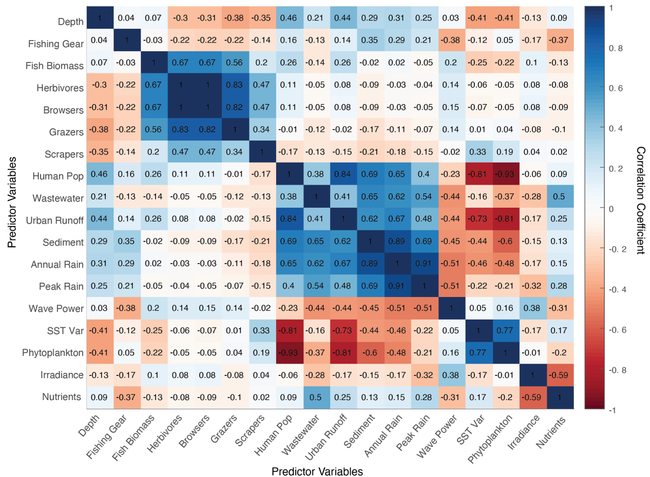
Fig. S4. Pearson correlation ( r ) coefficients for all predictor variables considered for the ordinal logistic regression (OLR) relating the percentage cover of reef-builders (hard coral + crustose coralline algae) four years following the 2015 marine heatwave to local land-sea human impacts and environmental factors. Where r = > 0.7 for any given pairwise comparison, one of the predictors was removed. We chose the predictor that was considered more interpretable in driving variation in the response variable should it come out as important in the top models. See Table S1 for summary information on local land-sea human impacts and environmental factors included in analysis. See Supplementary Methods for detailed information on calculating each impact or factor, including data collection methods, data sources and ancillary data sets, and specific tools or software utilised.
