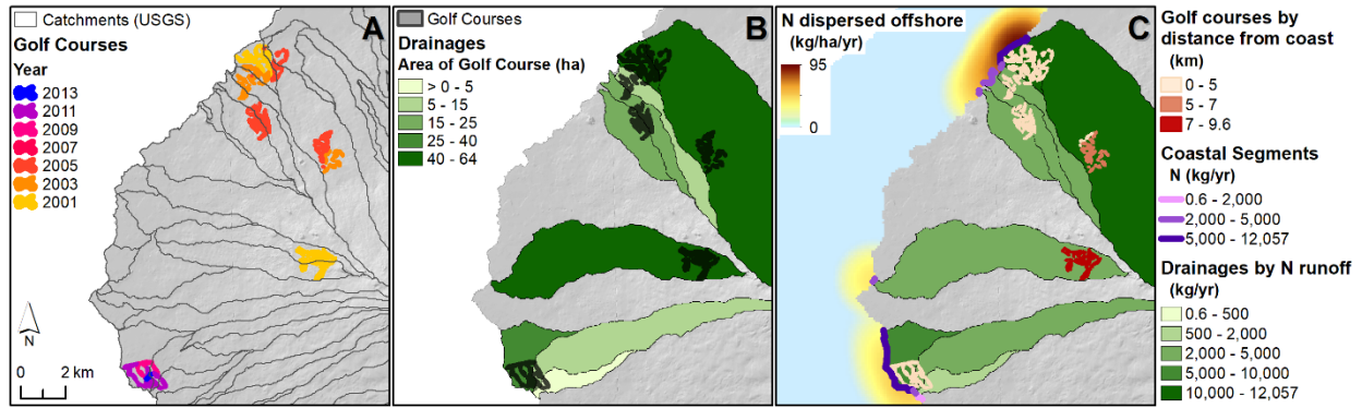
Fig. S10. Maps zoomed in to Keāhole Point vicinity illustrate the sequential process of deriving golf course nitrogen runoff from golf courses. A) Golf course footprints extracted from satellite imagery, coloured by the first year in which they appear in our time series of Landsat cloud free composite images (yellow to red to blue colouring), overlaid with USGS sub-watershed catchments (grey lines). B) Catchment polygons aggregated into larger drainage polygons that reach the coastline, coloured by the area of golf course contained in each (increasing from light to dark green). Golf course footprints are shown in dark grey. C) Drainages coloured by estimated nitrogen from golf courses reaching the coast (light to dark green) based on nitrogen application rate, leaching rate, and distance inland from coast. Coastline segments of each drainage are symbolized by the nitrogen load of the corresponding drainage (increasing from light to dark purple) and used as the input source features for offshore dispersal by a Gaussian decay function (light blue to dark orange shading represents low to high nitrogen input). Golf course footprints are coloured by distance inland from coast (increasing from light beige to red).
