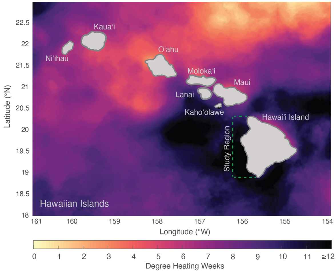
Fig. S1. Maximum heat stress during the 2015 marine heatwave. Map of the Hawaiian Islands showing the maximum Degree Heating Weeks (i.e., heat stress) experienced during the 2015 marine heatwave. Anything above 8 Degree Heating Weeks is expected to cause severe coral mortality 1 . The green dashed line encompasses the study region. Data shown are from NOAA's Coral Reef Watch 5 km Coral Temp version 3.1 data set ( https://coralreefwatch.noaa.gov/product/5km/ ).
