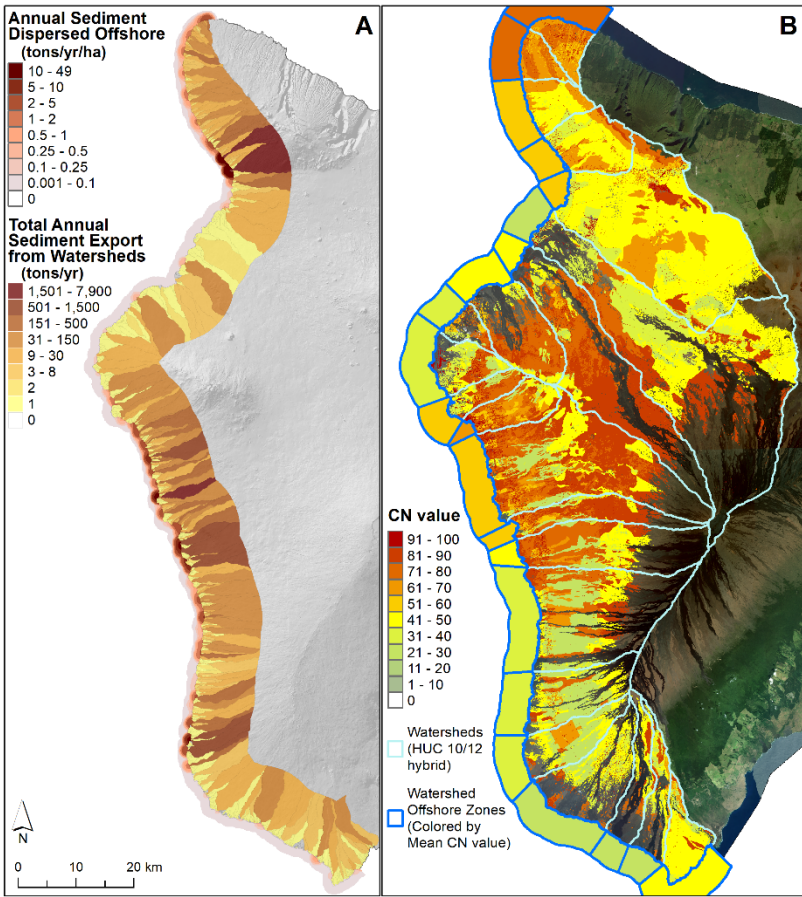
Fig. S16. Maps showing the static data input components used to produce the annual time series of sediment input. A) Average annual sediment load in tons by subwatershed (light yellow to brown; from 0-10 km inland), and average annual sediment load dispersed offshore with Gaussian kernel decay function (light pink to dark red). All values were derived from InVEST sediment delivery modelling. B) Curve number (CN) raster used in calculation of surface runoff (discharge) from rainfall data. CN values represent the runoff potential of hydrologic soil-cover complexes. Low values of CN represent low runoff potential and occur in highly permeable areas where the ground can absorb large amounts of rainfall before surface runoff occurs. High values of CN reflect areas where very little rainfall is required before surface runoff occurs (i.e., high runoff potential). The CN raster was derived by combining high resolution NOAA CCAP data (2010) and USGS soil hydro-group data (gSSURGO). CN values were assigned following the NRCS hydrology handbook 26 . Note that CN values of zero are displayed as no-colour and therefore the satellite image background shows through in these areas.
