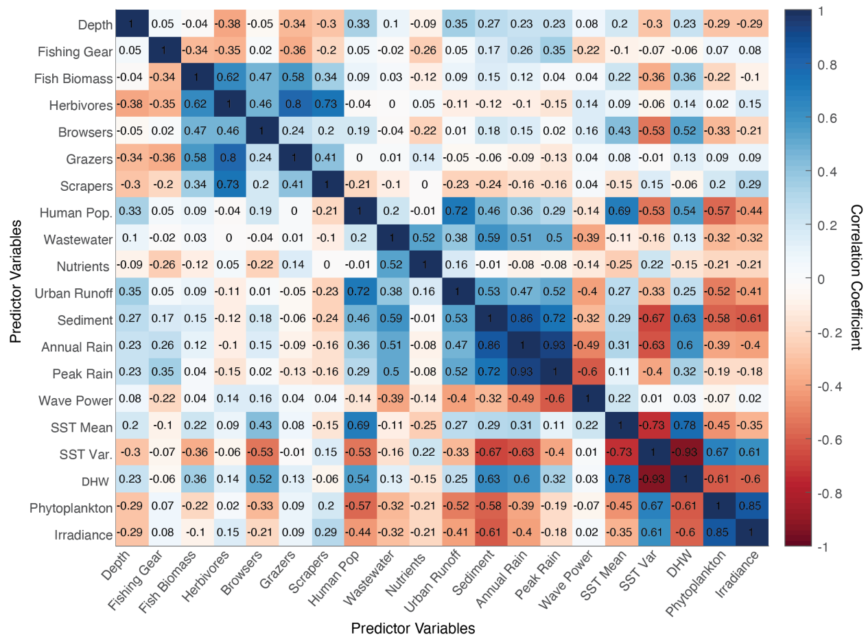
Fig. S2. Pearson correlation ( r ) coefficients for all predictor variables considered for the generalized additive mixed effects modelling relating coral response to the 2015 marine heatwave to local land-sea human impacts and environmental factors. Where r = > 0.7 for any given pairwise comparison, one of the predictors was removed. We chose the predictor that was considered more interpretable in driving variation in the response variable should it come out as important in the top models. See Table S1 for summary information on local land-sea human impacts and environmental factors included in analysis. See Supplementary Methods for detailed information on calculating each impact or factor, including data collection methods, data sources and ancillary data sets, and specific tools or software utilised.
