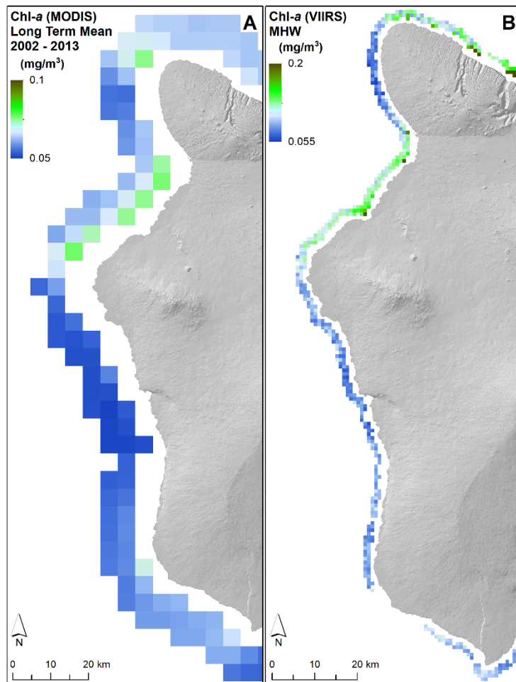
Fig. S20. Map showing the phytoplankton biomass (i.e. chlorophyll- a ) from A) Wedding et al., 2018 and (B) VIIRS. The VIIRS data provide much higher spatial resolution (750 m versus 4 km) but are only available from 2014 onwards. VIIRS data source: www.star.nesdis.noaa.gov/jpss/VIIRS.php
