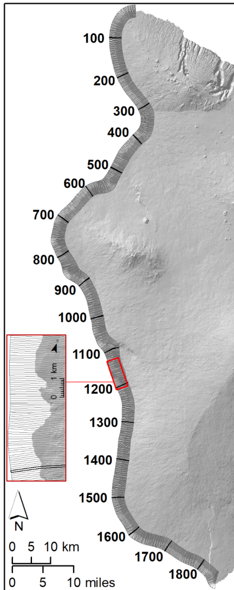
Fig. S22. The 100-m width coastal sectors along our study area numbered ascending from north to south (labelled every 100 sectors, or approx. every 10 km), with inset map showing detailed view of sectors.
