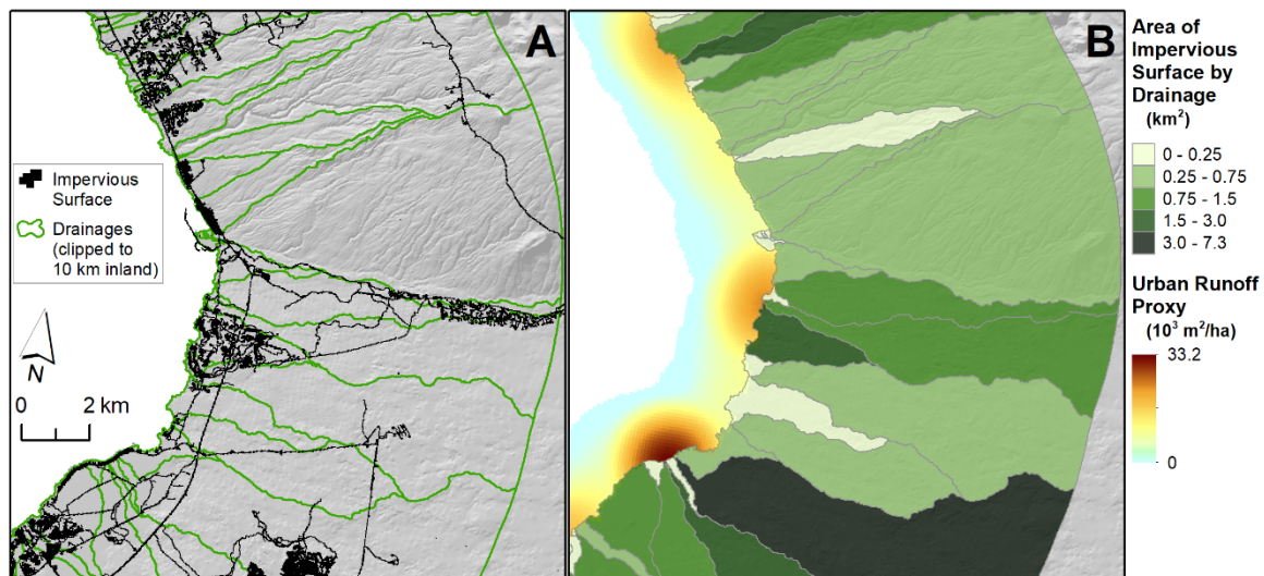
Fig. S12. These maps zoomed in to Kawaihae Bay area illustrate the process of deriving our proxy layer for urban runoff from impervious surface land cover data. A) Impervious surface land cover footprint (black) for an example year overlaid with sub-watershed drainage polygons clipped to 10 km inland. B) Drainage polygons coloured by area of impervious surface (light to dark green), and dispersal offshore by Gaussian kernel decay function (light blue to dark orange shading represents low to high urban runoff).
