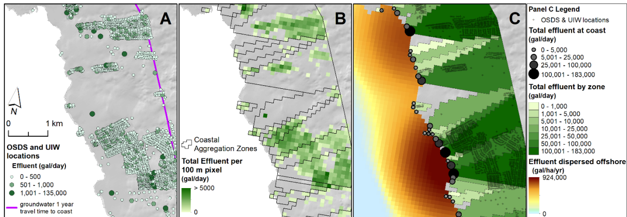
Fig. S7. These maps zoomed in to Kailua-Kona illustrate the sequential process of deriving wastewater pollution from OSDS and injection well location data. A) OSDS and injection well locations (circles) symbolized by effluent input into the environment: small, light green circles represent lower effluent and larger, dark green circles represent higher effluent. The purple line represents the 1-yr travel time of groundwater to the coast. B) Total effluent from OSDS and injection wells summed within 100 m pixels, with increasing values represented by light to dark green shading. Zones connecting OSDS and injection wells to the nearest pixel on the shoreline are outlined in black. C) Zones coloured by increasing total effluent (the sum of effluent pixels shown in panel B by zone; light to dark green), overlaid with OSDS and injection well locations (small grey crosses), and the terminal point of each zone along the shoreline symbolized by increasing total effluent (light to dark grey circles of increasing size). Terminal points have identical effluent values to their corresponding zones and are used as the source features for offshore dispersal with a Gaussian decay function (light blue to dark orange shading represents low to high effluent input).
