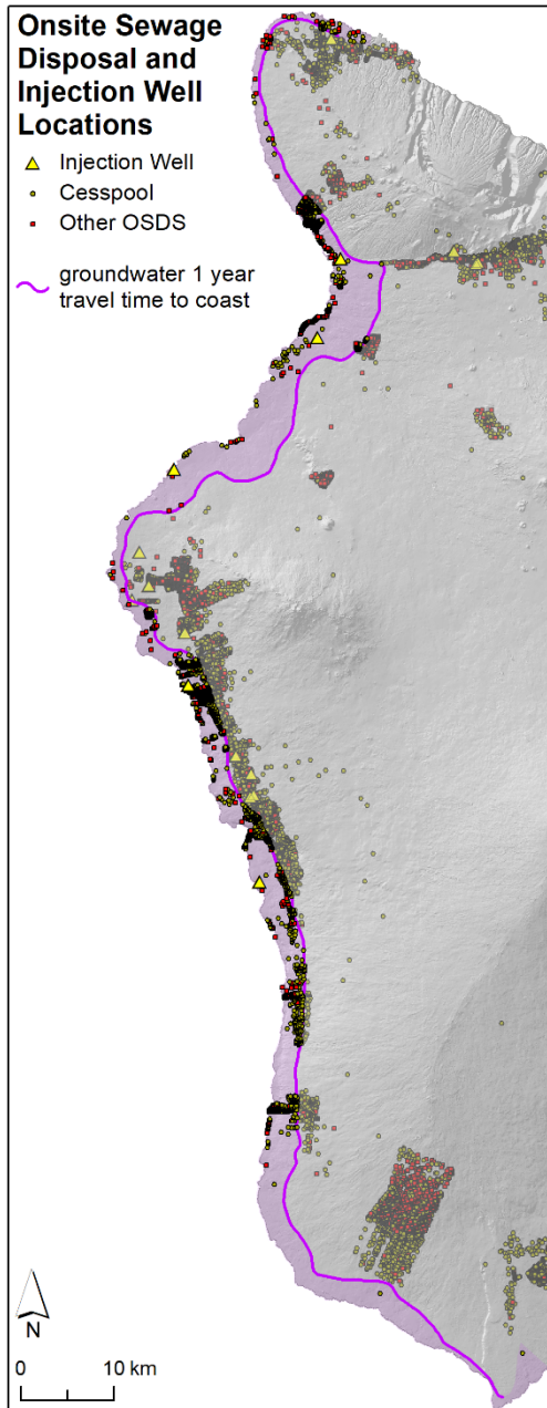
Fig. S6. Map of onsite sewage disposal systems (OSDS) and injection wells across our study region in West Hawai'i. The purple line delineates the 1-yr travel time in the groundwater to reach the coast and was used as a cut-off for inclusion of onsite sewage disposal systems (OSDS) and injection wells in this analysis.
