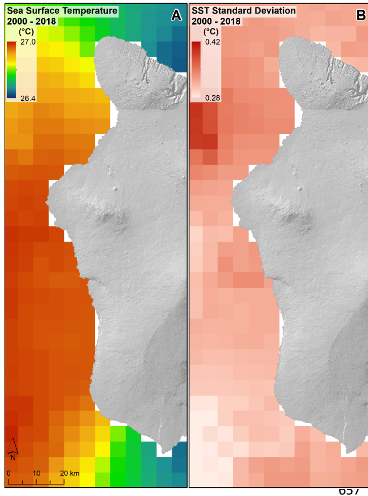
Fig. S19. Map showing the mean (A) and standard deviation (B) in summertime SST across the study region. Maps show the long-term mean from 2000 – 2018.
