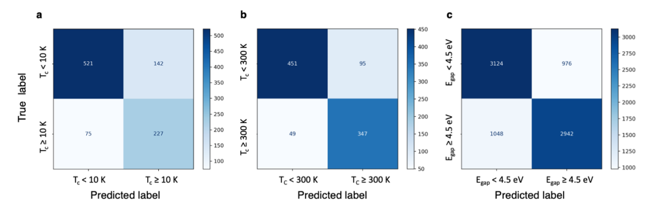
Supplementary Figure 11. Confusion matrices for binary classification models with threshold probability 0.5. a Superconducting materials classification of 20% of the collected data from MPDS 7 and SuperCon 8 with respect to transition temperature 10 K; b magnetic materials classification of 20% of the collected data from MPDS, with respect to Curie temperature 300 K; c classification materials with reported values of energy band gap with respect to energy gap value 4.5 eV, test set is 20% of randomly selected data collected from MPDS.
